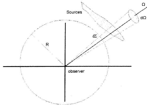
Figure 2: Geometry for computing incident electromagnetic radiation
