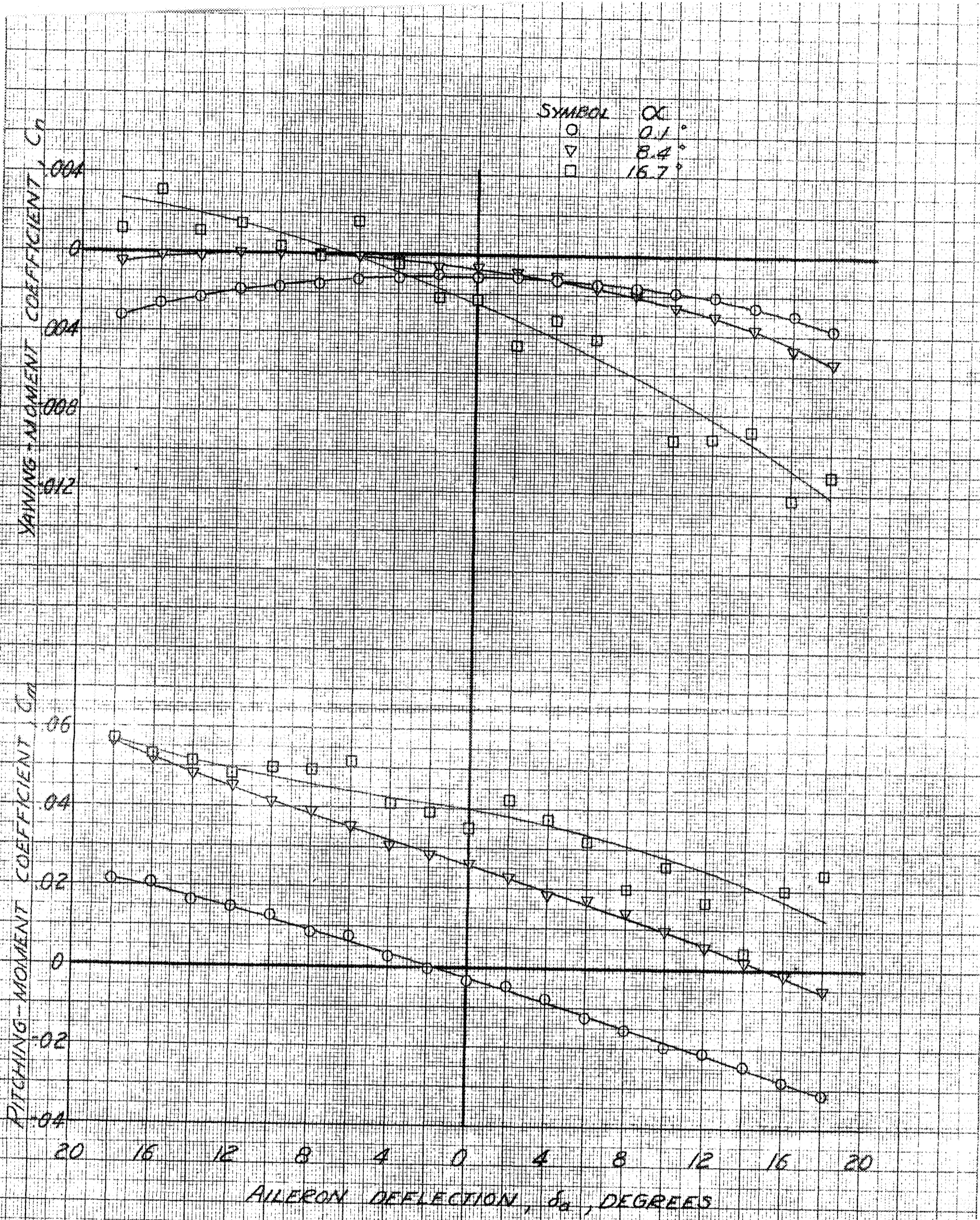
(b) C_{\eta} AND C_{\eta\eta} VS. \delta_a
