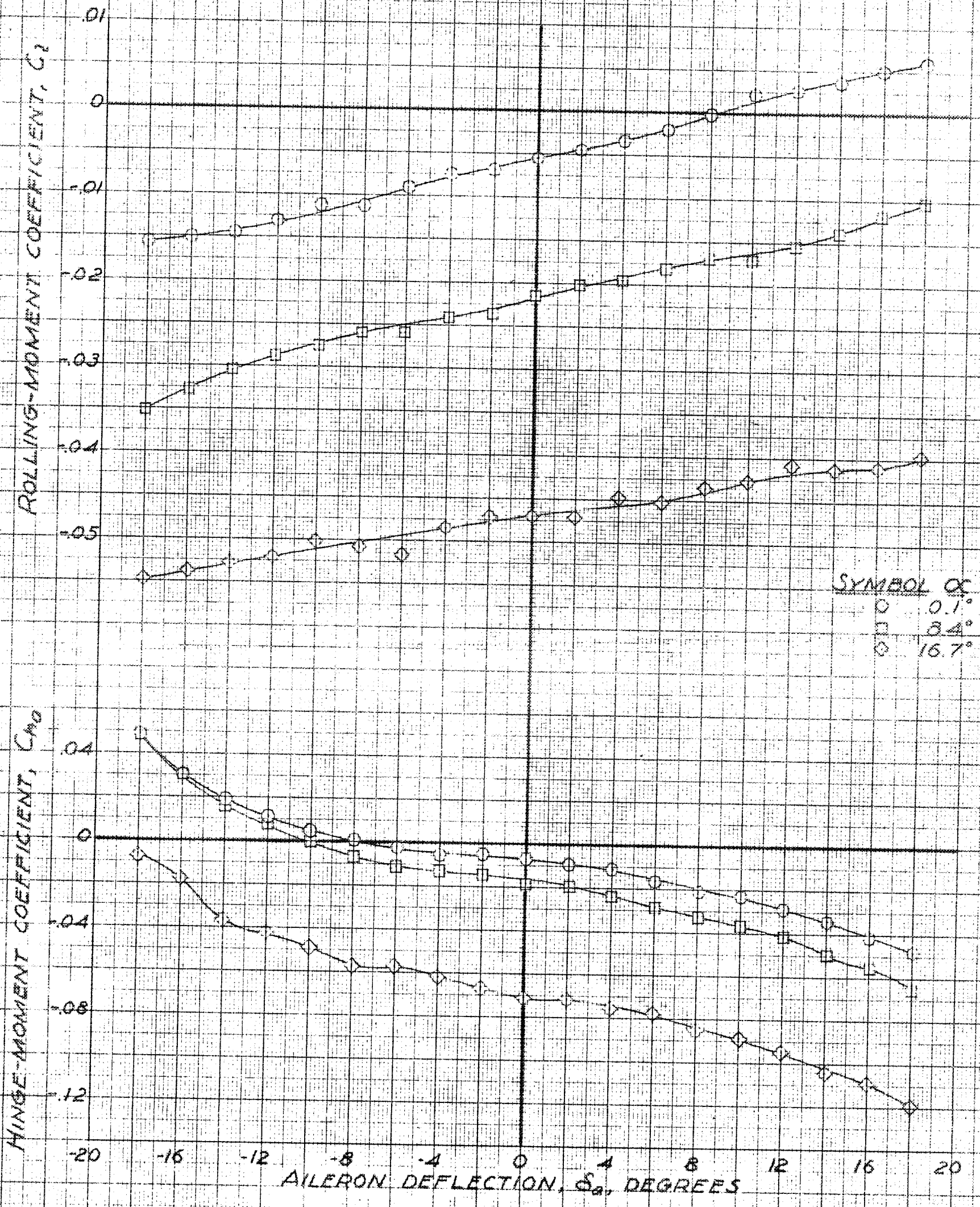
(a) C_l, C_{h0} vs. \delta_a .
