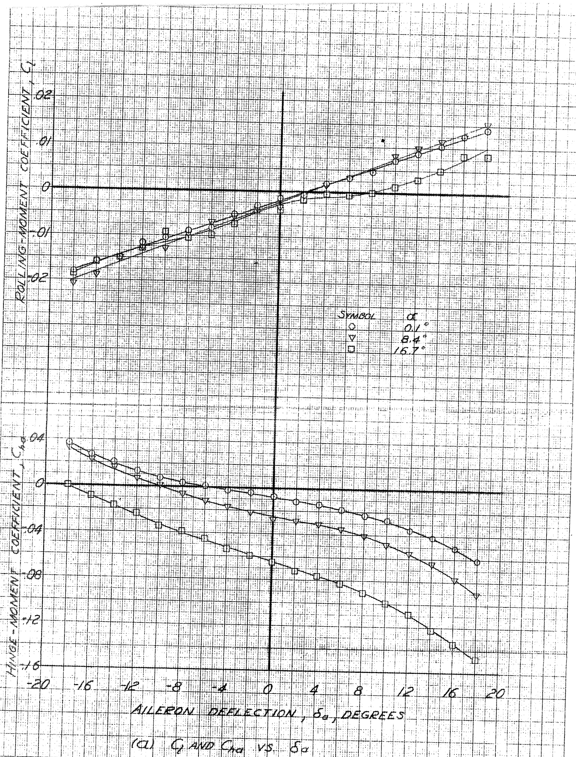
FIGURE 31. — EFFECT OF AILERON DEFLECTION ON THE AERODYNAMIC CHARACTERISTICS OF THE REPUBLIC XP-91 WING. OUTBOARD STRAIGHT FLATS EXTENDED 0.05 M.A.C.; \beta , 0.1°.
