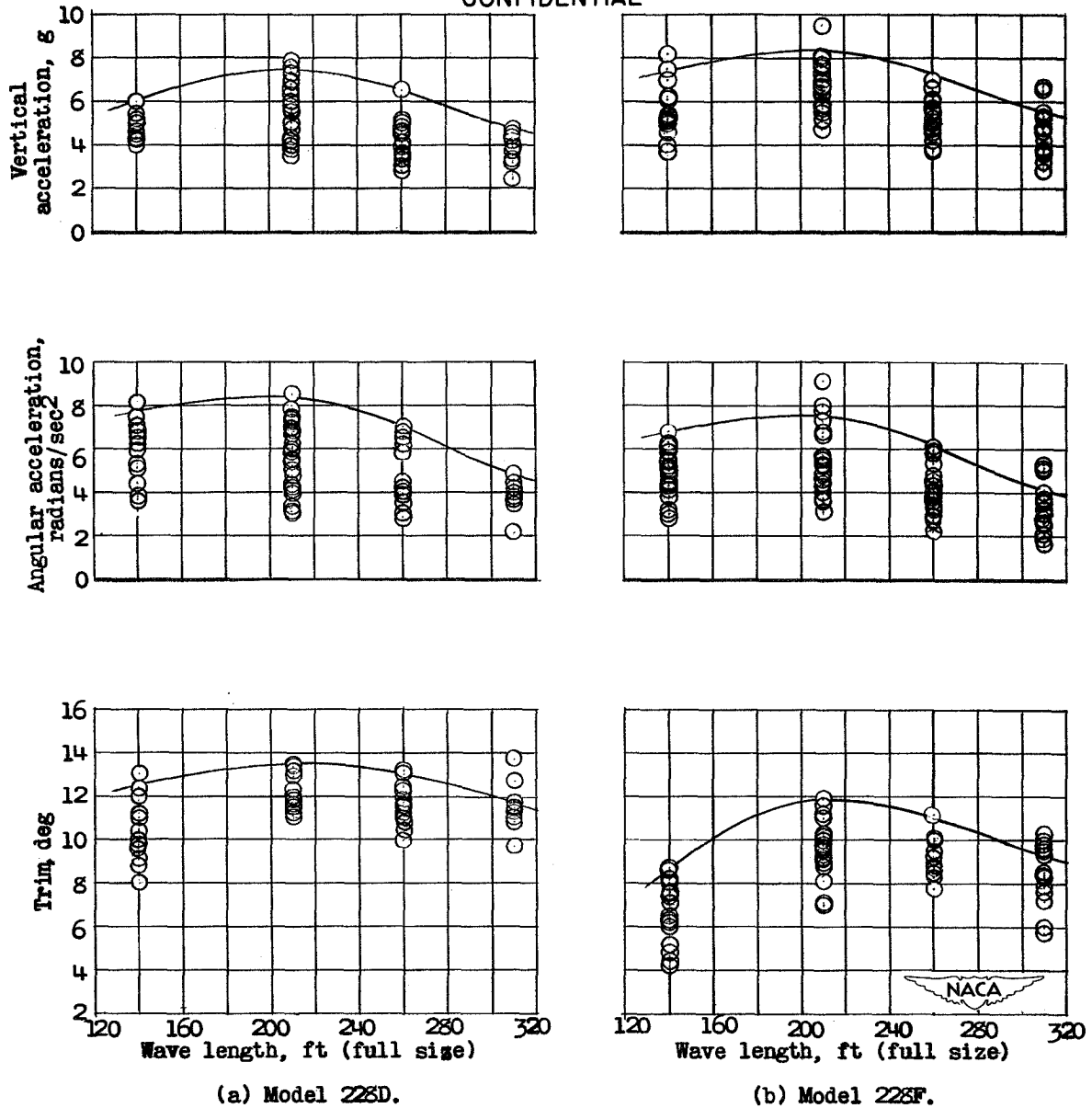
Figure 4.- Maximum accelerations and trims during landing run-out.
