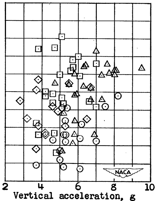
(b) Model 228F.
