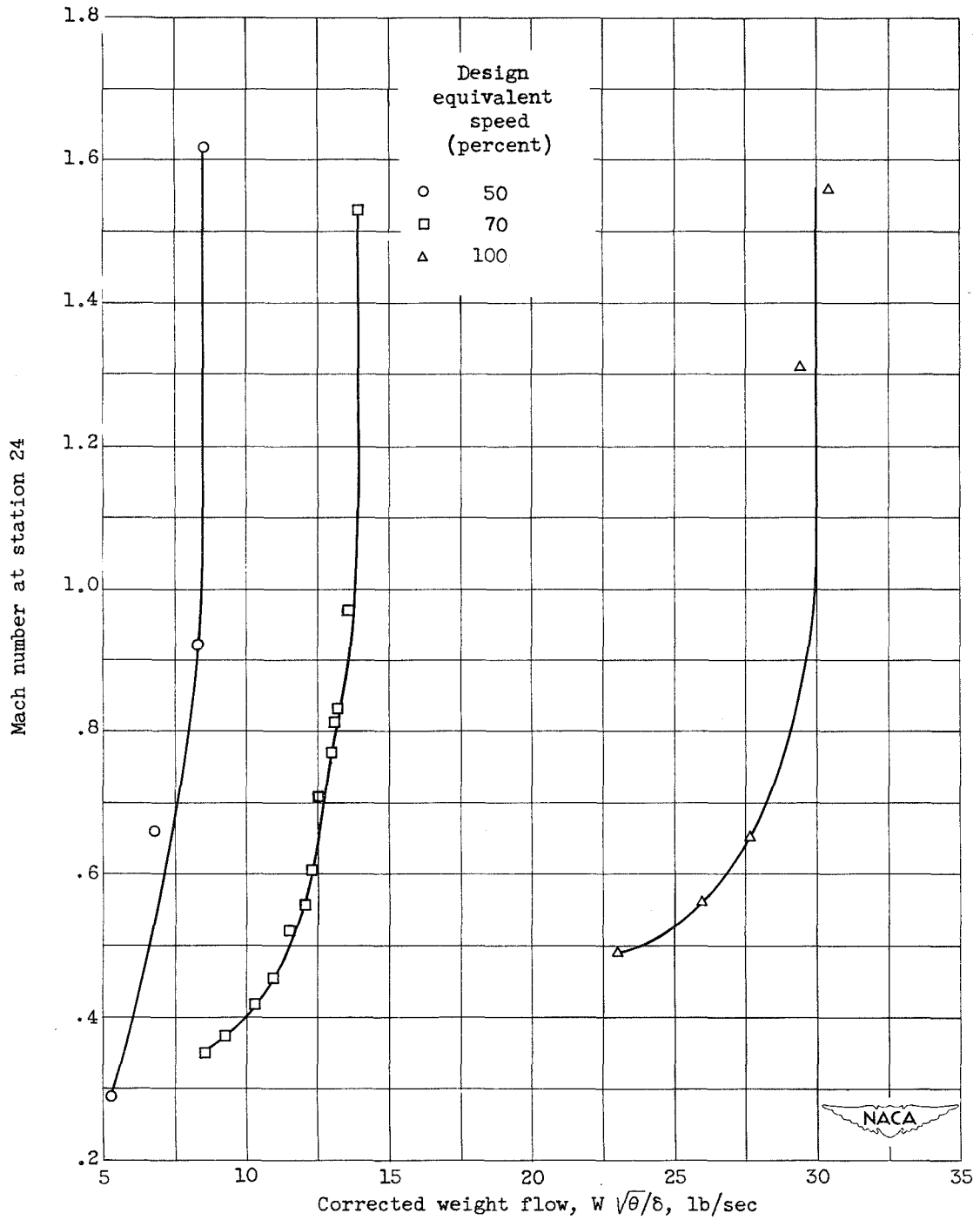
Figure 5. - Mach number at station 24.
