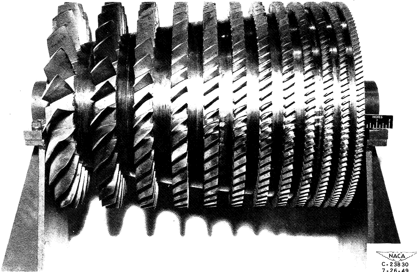
(a) Rotor.
