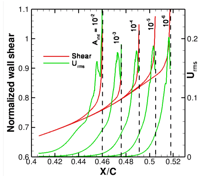
Fig. 9. Evolution of wall shear and secondary instability RMS amplitude for Z-mode secondary instability as control amplitude varies. The dashed vertical lines indicate the transition locations based on the wall-shear criterion.
