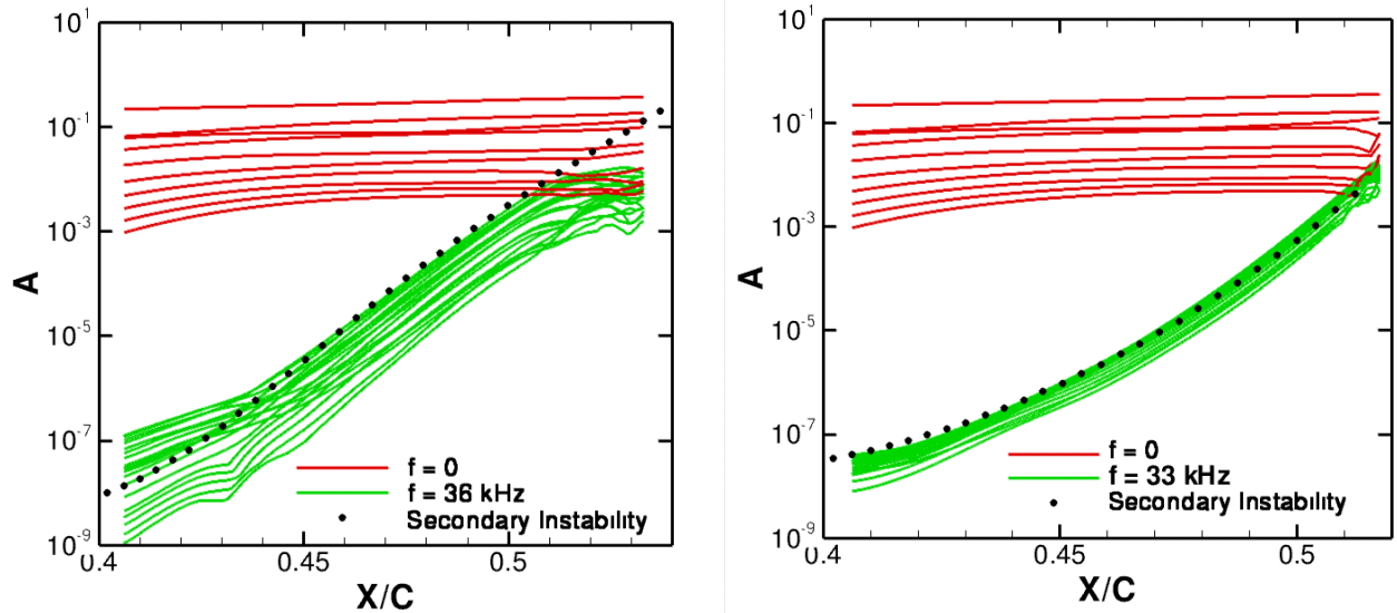
Fig. 8. Amplitude evolution of primary and secondary instability perturbations. Each line is associated with a fixed spanwise wavenumber. The red lines represent stationary modes (predominantly associated with primary crossflow instability) and the green lines represent secondary instability modes at the fundamental frequency (higher frequency harmonics are not shown). The black dots represent results from linear secondary instability theory. The y-mode secondary instability is shown on the left, and the z-mode on the right.
