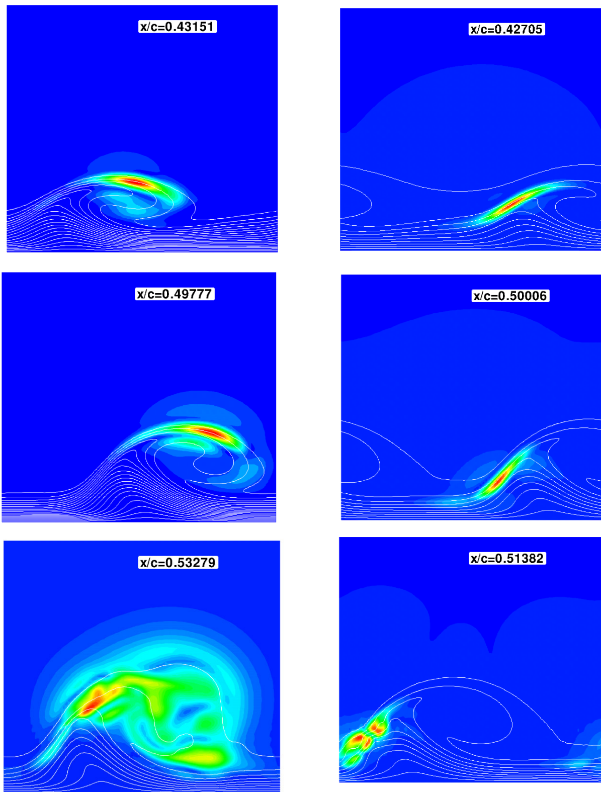
Fig. 11. Time-RMS distributions of chordwise velocity distributions at selected chordwise stations. The white lines in the background are the u-contours of stationary crossflow vortex. The y-mode is displayed on the left and the z-mode on the right. Secondary instability initial amplitude is 1e-6 .
