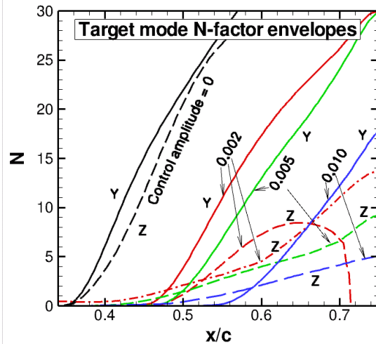
Fig. 7. Envelopes of N-factor curves for dominant Y and Z families of secondary modes at increasing levels of control amplitude.
