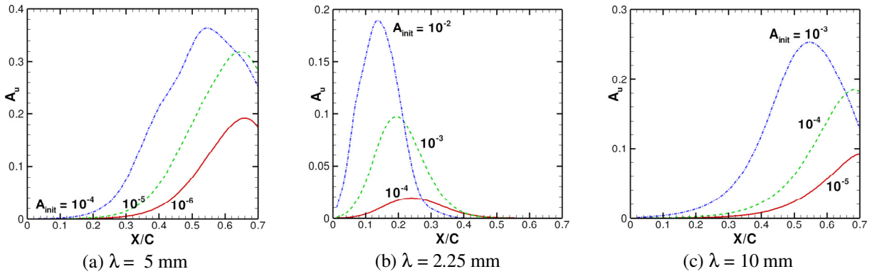
Fig. 1. Nonlinear evolution of fundamental disturbance amplitude for a stationary crossflow mode at specified spanwise wavelength, with the initial disturbance amplitude as a parameter
