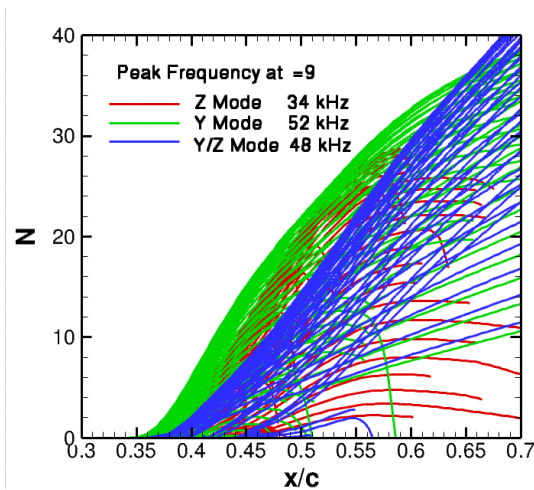
Fig. 6. N-factor curves for spatially growing disturbances at selected frequencies within each family of high-frequency secondary instabilities (indicated by different colors as described in the legend).
