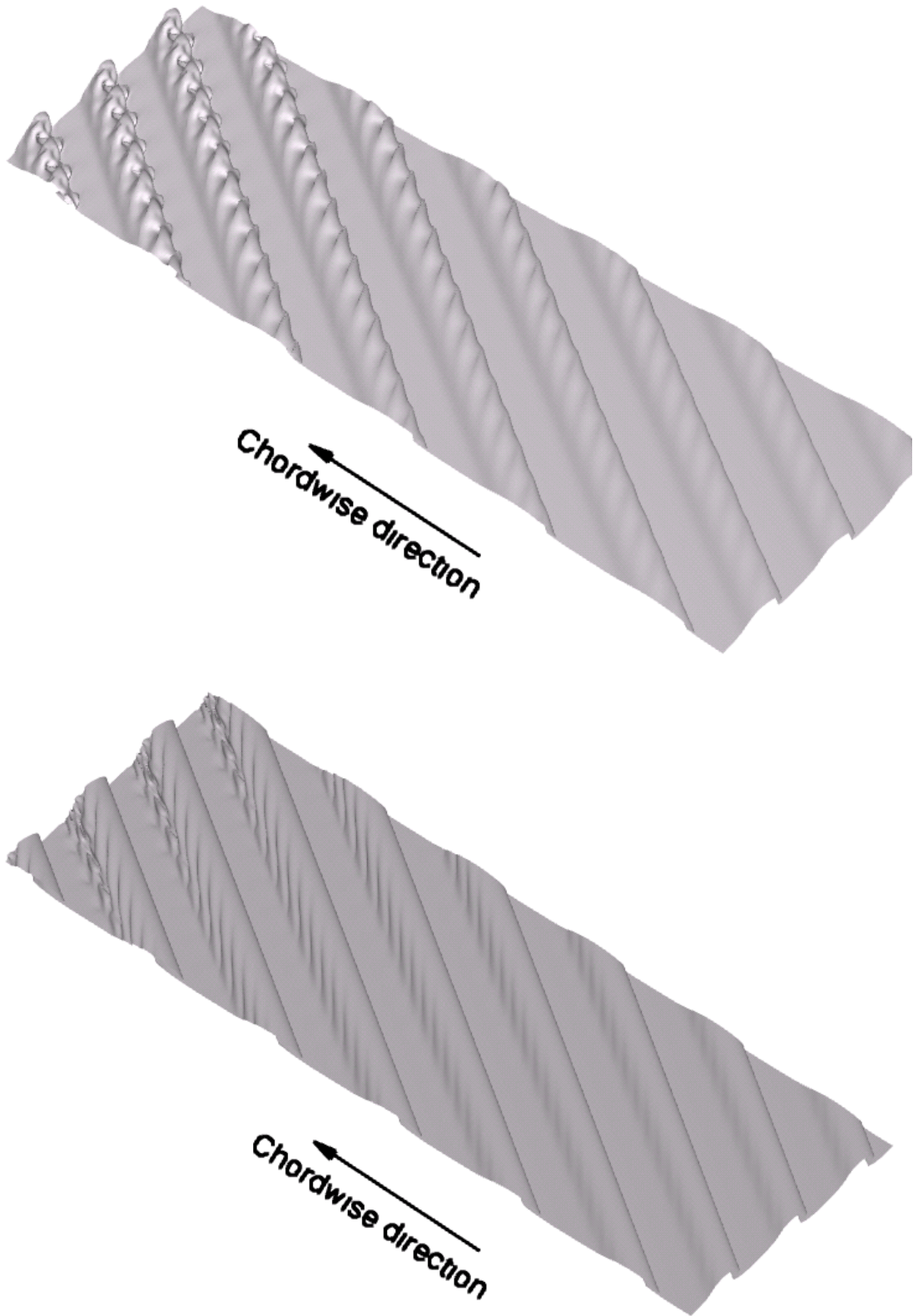
Fig. 12. Iso-surfaces of instantaneous chordwise velocity U . Top: Y -mode, U = 0.91U_\infty . Bottom: Z -mode, U = 0.87U_\infty .
