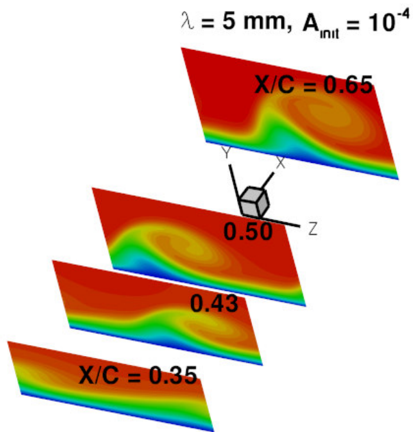
Fig. 2. Chordwise velocity contours across vortex cross section extending over one spanwise wavelength ( \lambda = 5 mm, A_i = 1e-4 )
