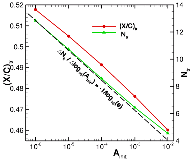
Fig. 10. Transition location and transition N-factor as function of logarithm of secondary instability initial amplitude is almost a straight line. The latter falls approximately on a straight line with a slope given by Eq (2). (Note: the expression indicating the slope is equivalent to Eq (2), but is expressed in logarithm to the base 10 instead of natural logarithm to be consistent with the scaling of the horizontal axis).
