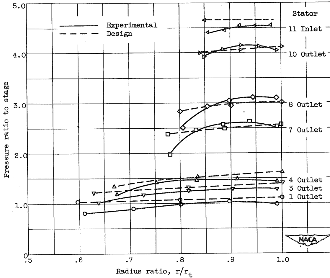
Figure 15. - Total-pressure-ratio distributions at several stator stations at an equivalent engine speed N/\sqrt{\theta} of 7198 rpm.
