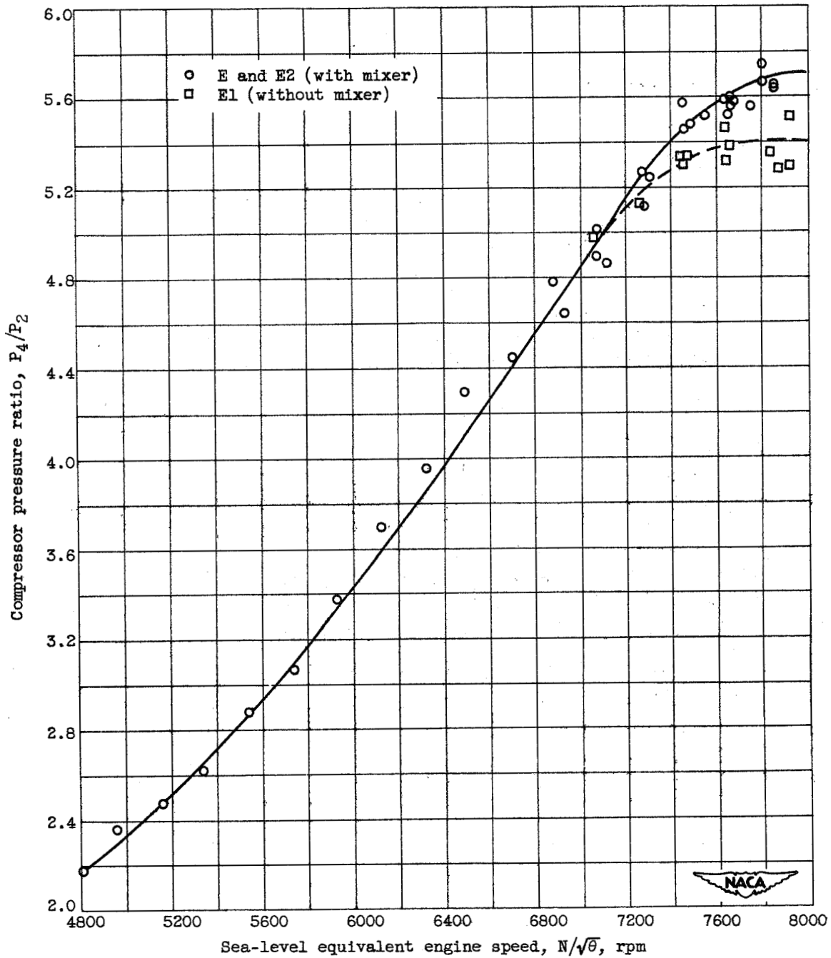
Figure 18. - Effect of mixer assembly at compressor outlet on surge limit of configuration E.
