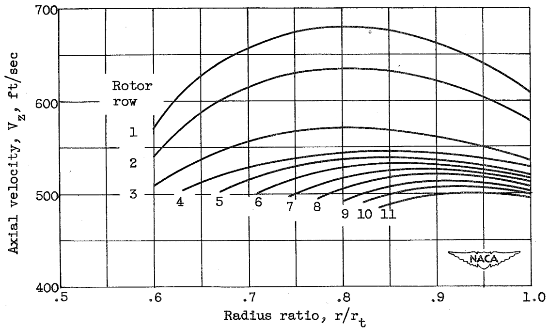
Figure 9. - Design axial-velocity distribution at rotor inlet on XJ40-WE-6 compressor.
