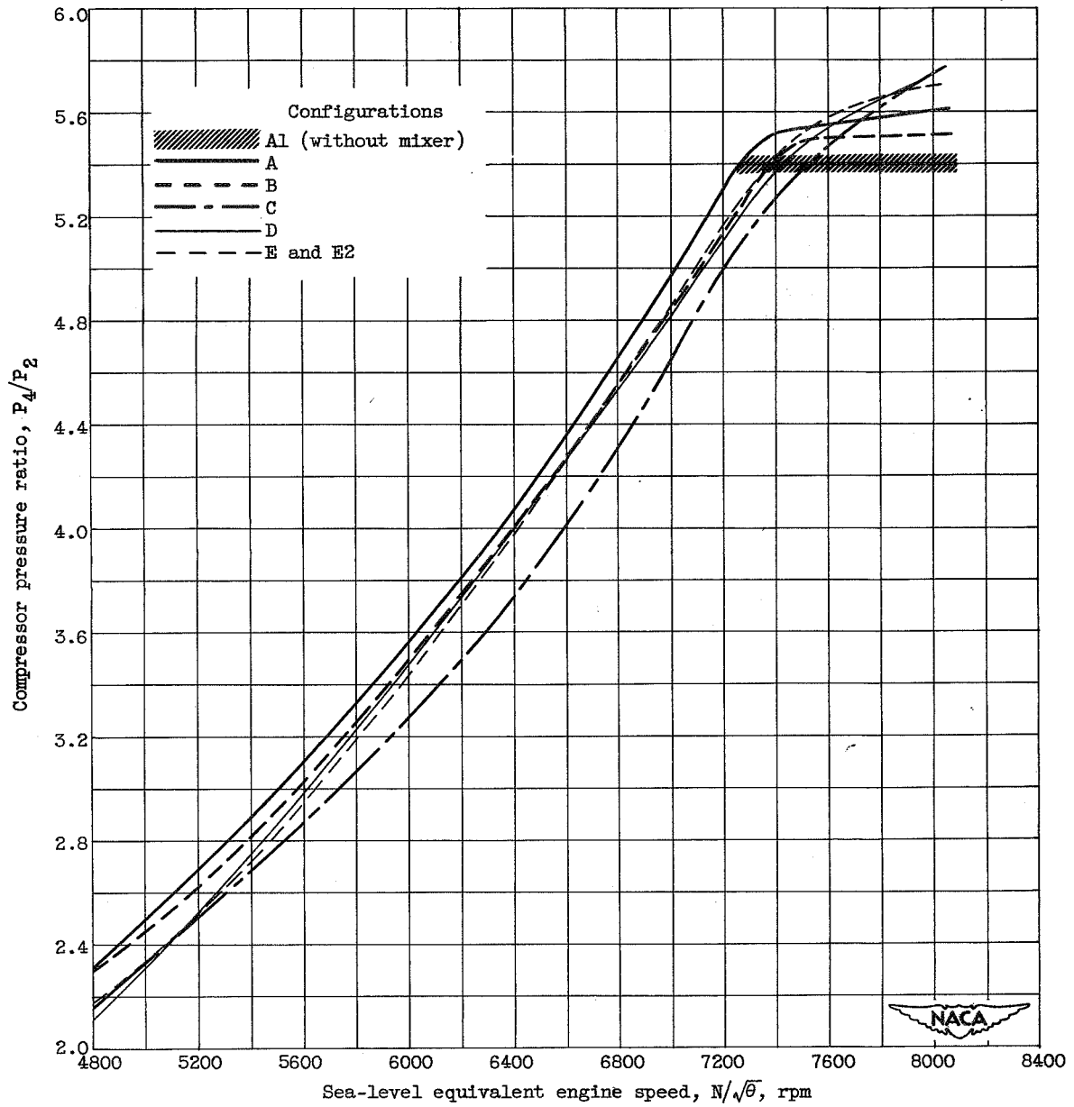
Figure 17. - Comparison of surge lines for the various compressor configurations investigated.
