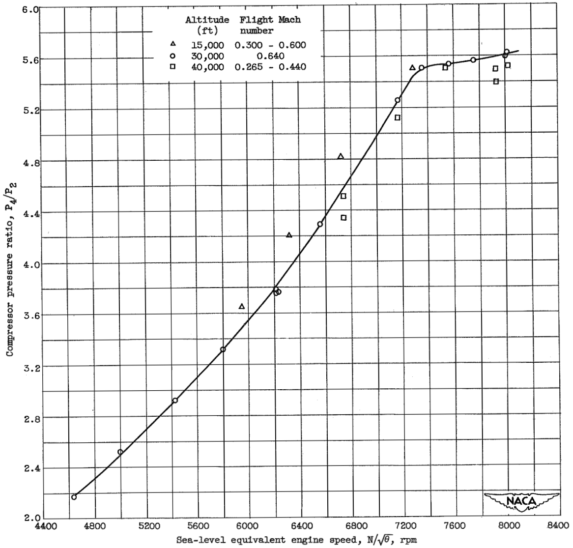
Figure 16. - Surge limit of standard compressor with mixer (configuration A).
