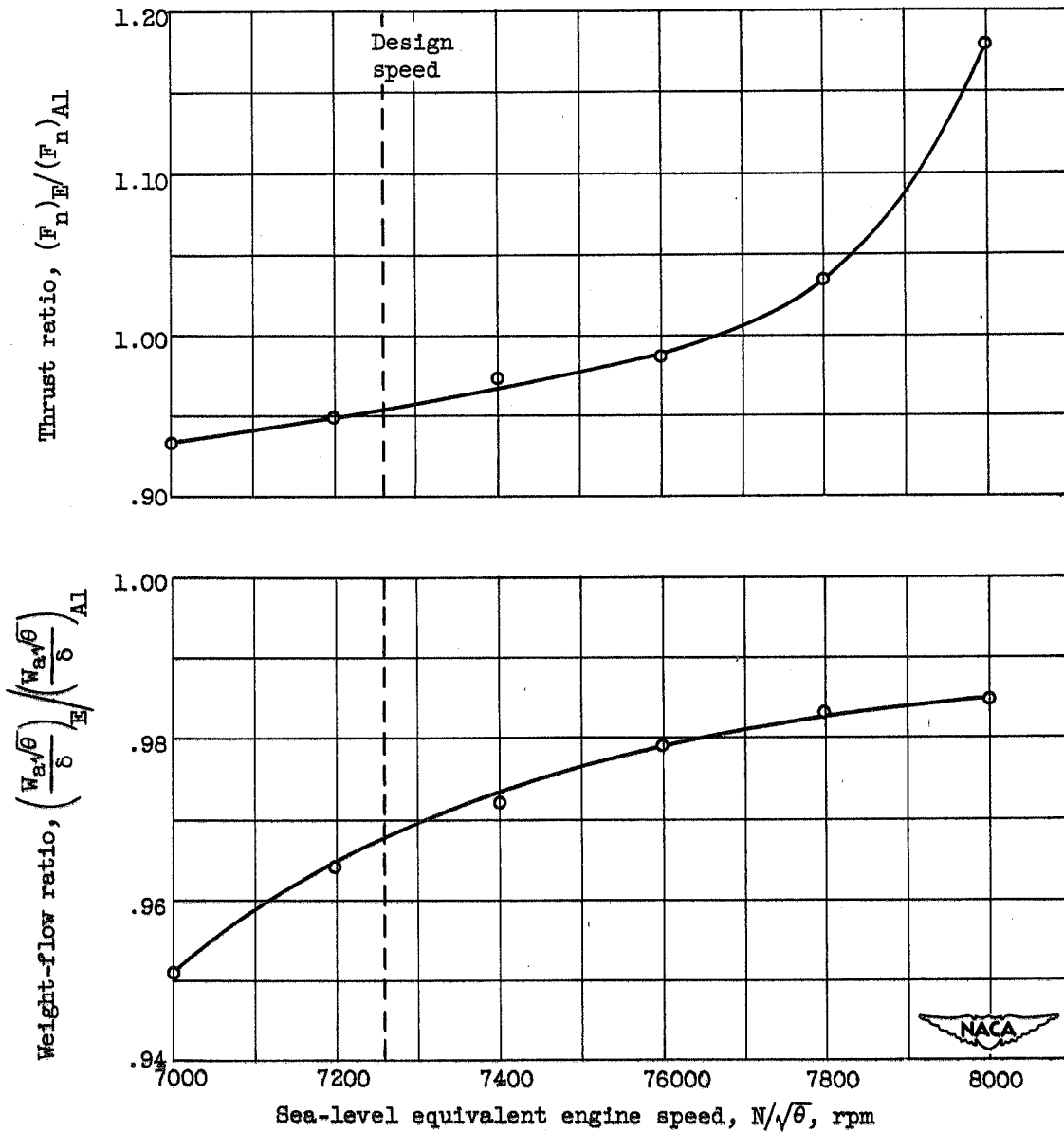
Figure 19. - Ratios of calculated net thrust and measured equivalent air flow for final and original compressor configurations. Altitude, 30,000 feet; flight Mach number, 0.64.
