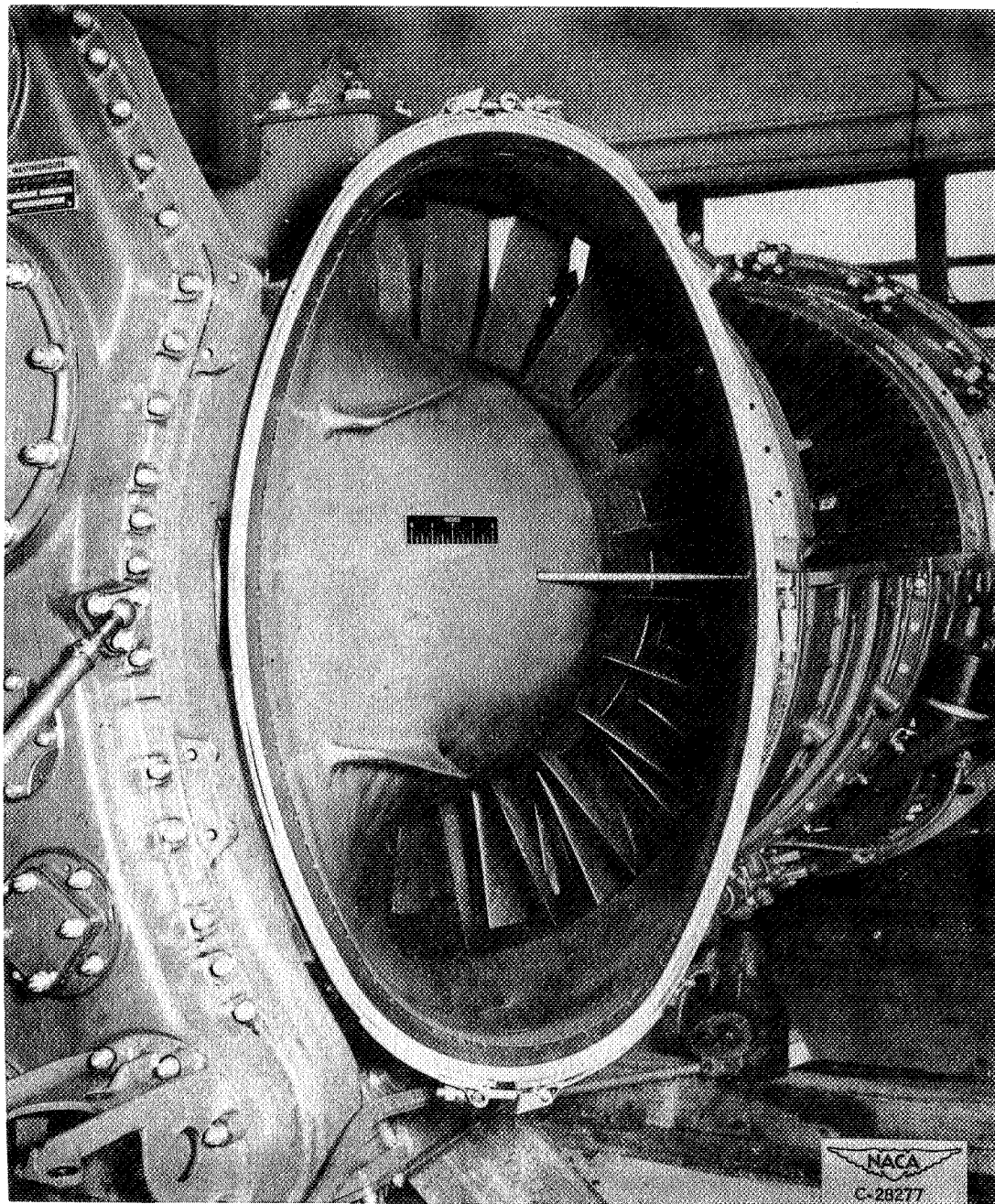
Figure 2. - Compressor-inlet duct section.
