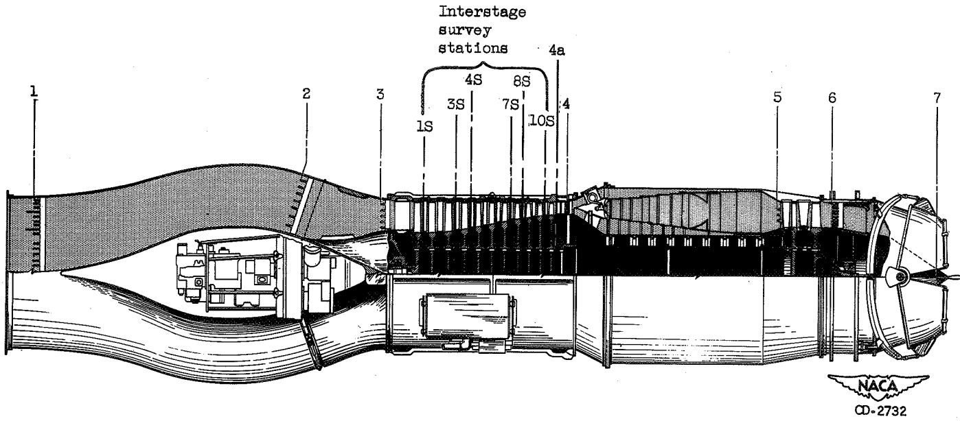
Figure 6. - Cross-section drawing of engine showing instrument stations.
