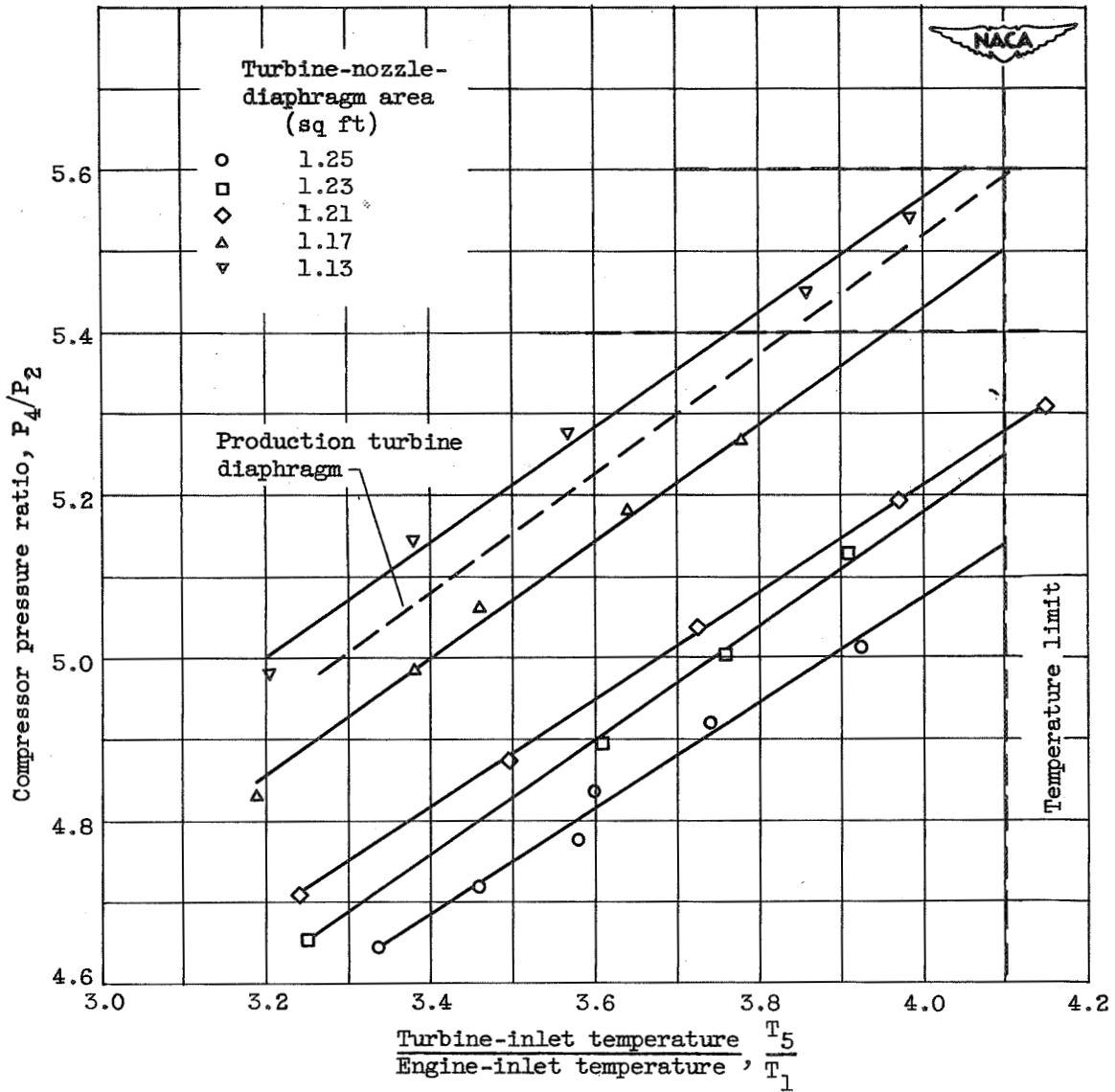
Figure 8. - Effect of changing area of turbine-nozzle diaphragm on compressor pressure ratio. Altitude, 30,000 feet; flight Mach number 0.64; equivalent engine speed N\sqrt{\theta} of 7710 rpm.
