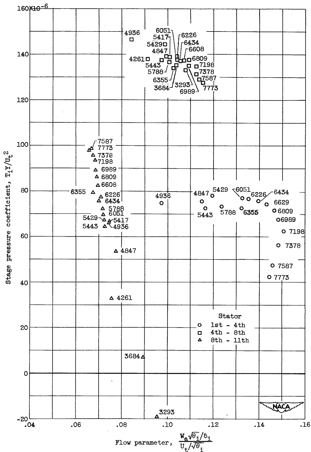
Figure 13. Operating points of front, middle, and rear sections of standard XJ40-WE-6 compressor for various equivalent engine speeds in rpm.
