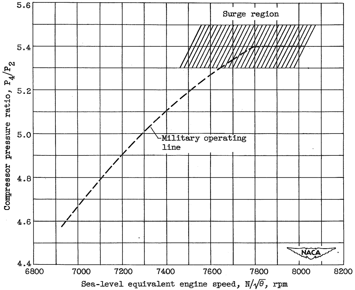
Figure 11. - Relation of military power operating line and surge limit of original compressor configuration (A1).
