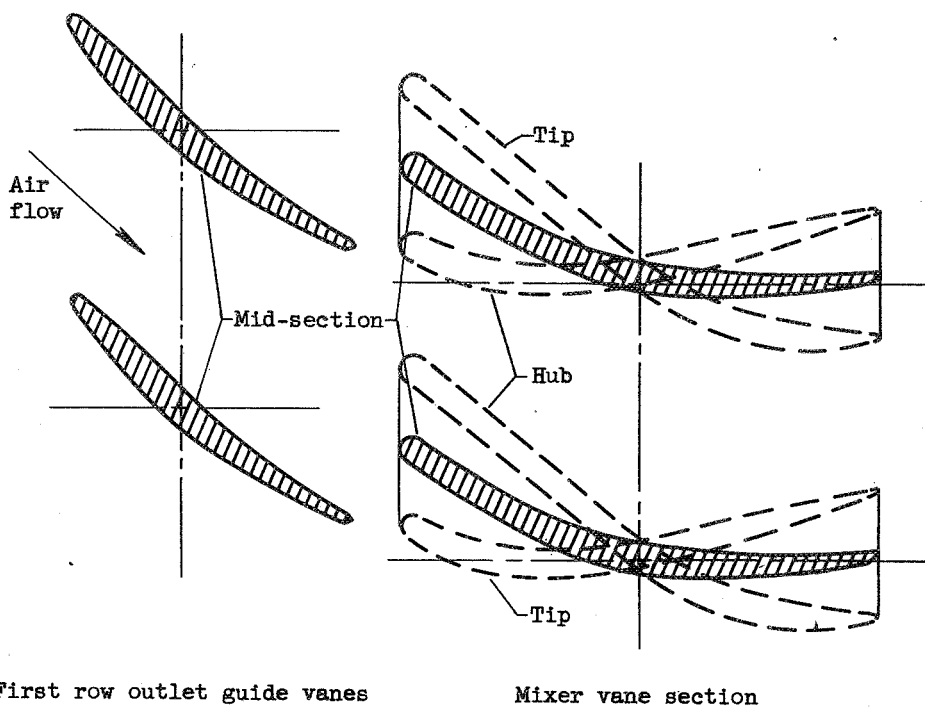
(a) Blade cross-sections
