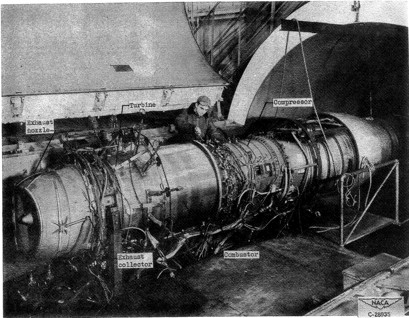
Figure 1. - XJ40-WE-6 engine installed in altitude wind tunnel.
