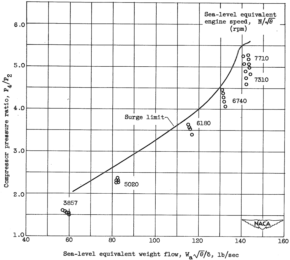
Figure 12. - Operating map of standard compressor with mixer installed (configuration A). Altitude, 30,000 feet; flight Mach number, 0.64.
