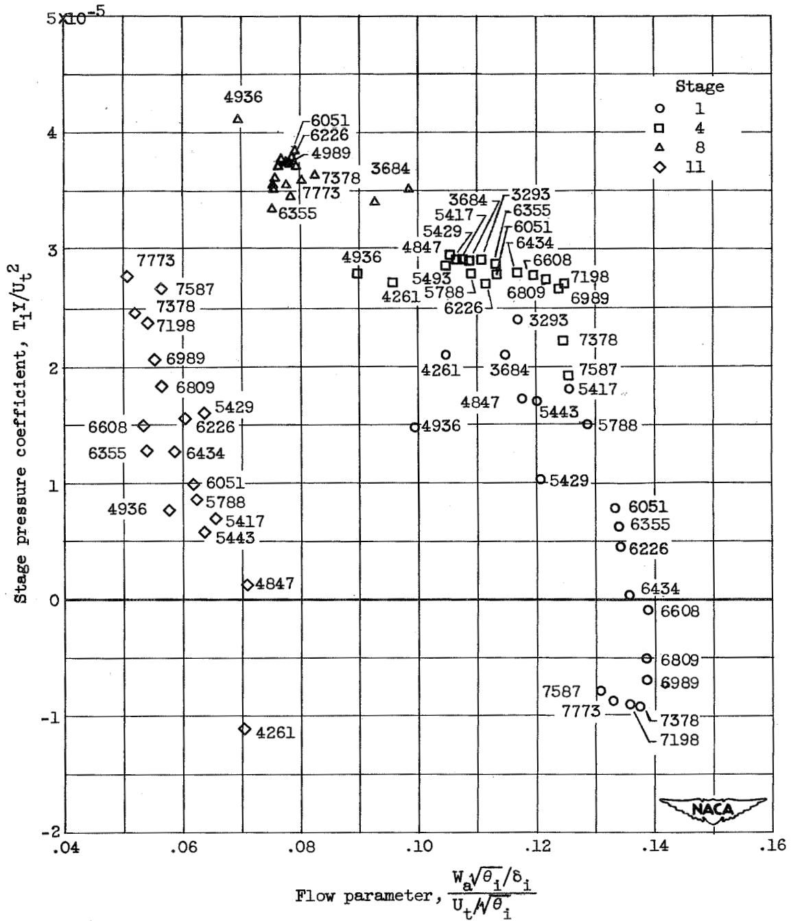
Figure 14. - Stage operating points for several stages of standard XJ40-WE-6 compressor for various equivalent engine speeds in rpm.
