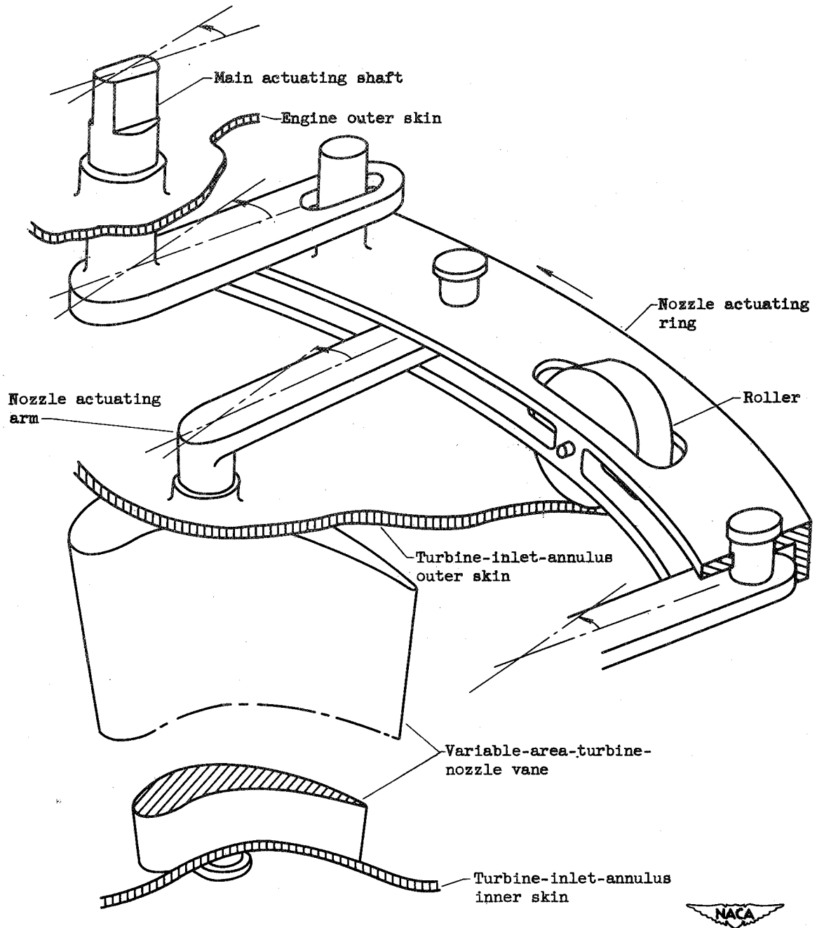
Figure 5. - Schematic sketch of variable-area-turbine-nozzle actuating mechanism.
