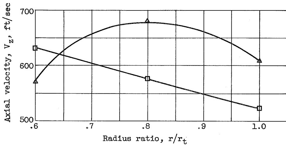
Figure 10. - Flow conditions at first rotor inlet for XJ40-WE-6 compressor.
