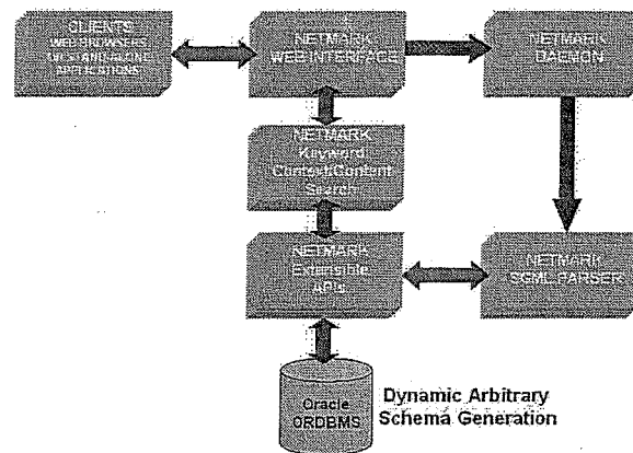
Figure 1: NETMARK Universal Process Flow
