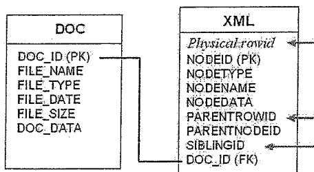
Figure 2: NETMARK Generated Schema
