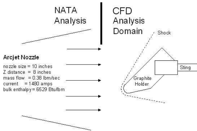
Figure 2. Case 2033. The schematics of the experimental facility.
