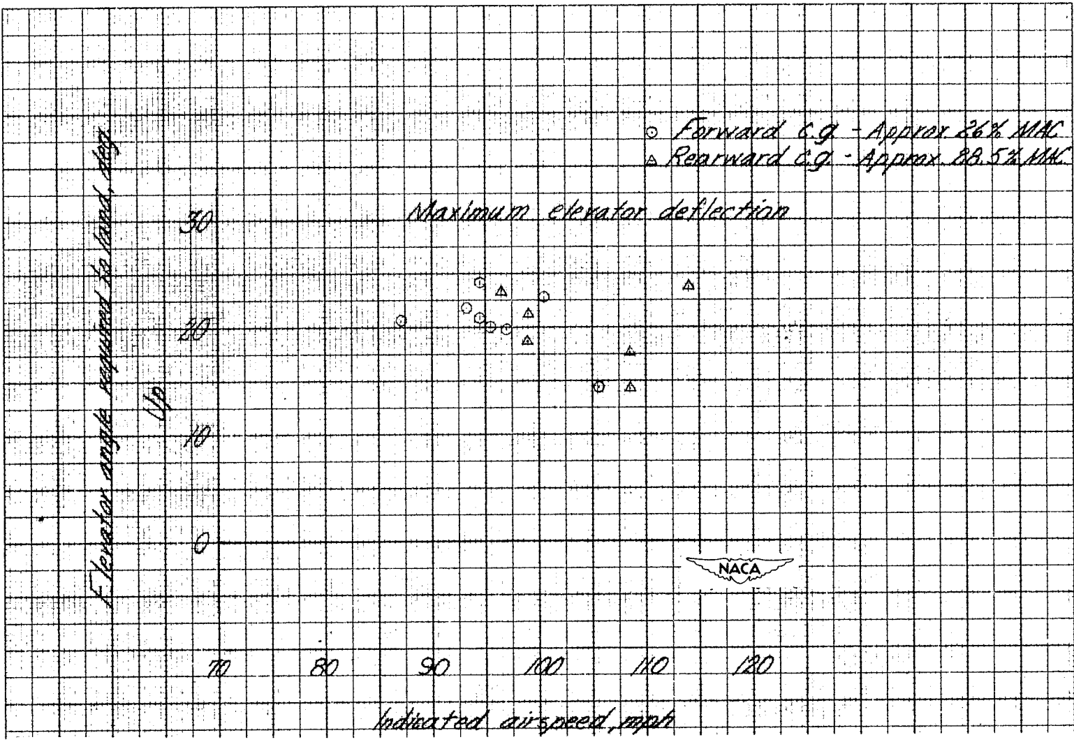
Figure 43.- Variation of elevator angle required to land with airspeed, P-47D-30 airplane.
