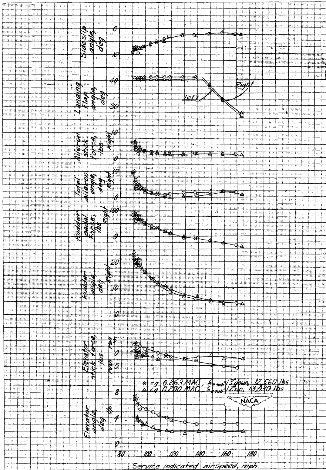
Figure 18.- Longitudinal stability characteristics of the P-47D-30 airplane in the approach condition at approximately 5000 feet.
