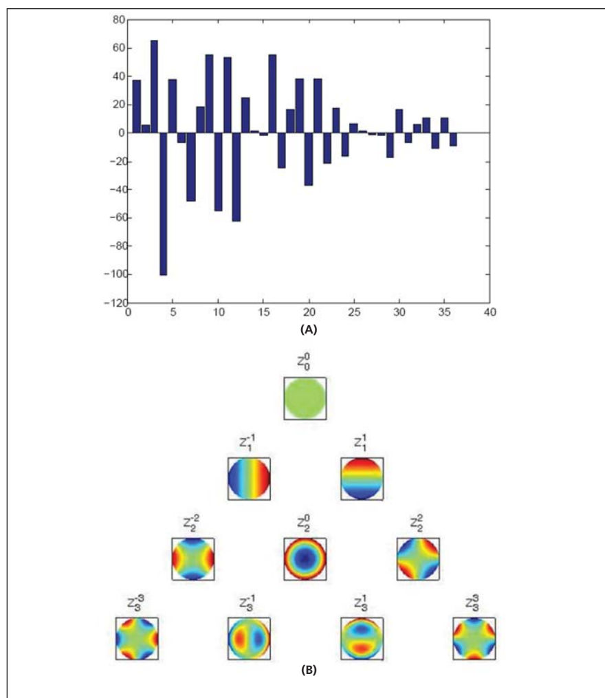
Figure 2. (a) Quantification of Optical Aberration as introduced by an arbitrary lens is manifested by amplitude of its Zernicke coefficients specified in the order of ( n=0, 1, 2, 3 , etc.: m=-n, \dots, 0, \dots, n if n even ; -n, \dots, n if n odd). (b) First 10 individual Zernicke functions are plotted.
