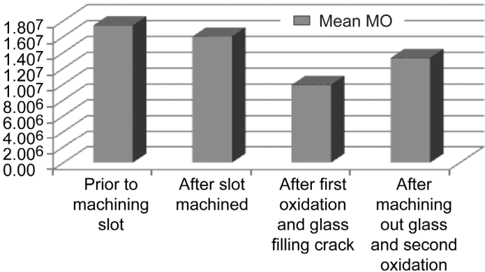
Figure 8. Ultrasonic guided wave (mean total energy M_0 ) results on sample RCC1 (fig. 2). Measurement variability is about 2 percent based on repeated trials.
