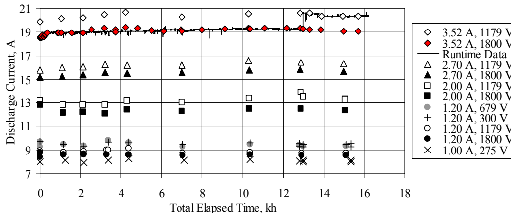
Figure 14.—Discharge current data as a function of time.
