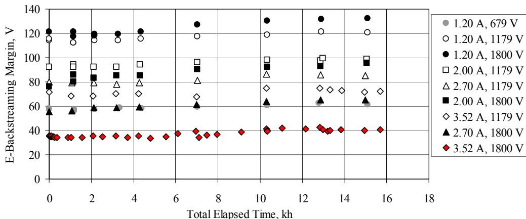
Figure 23.—Thruster ion optics' electron backstreaming limit data as a function of time.
