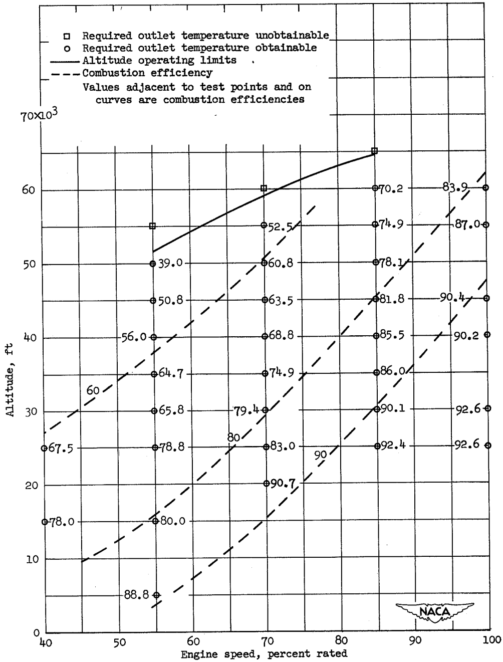
Figure 10. - Combustion efficiencies and altitude operating limits of J47 single combustor at various engine speeds and altitudes. Fuel, MIL-F-5572, grade 115/145 (weathered); flight Mach number, 0.52.
