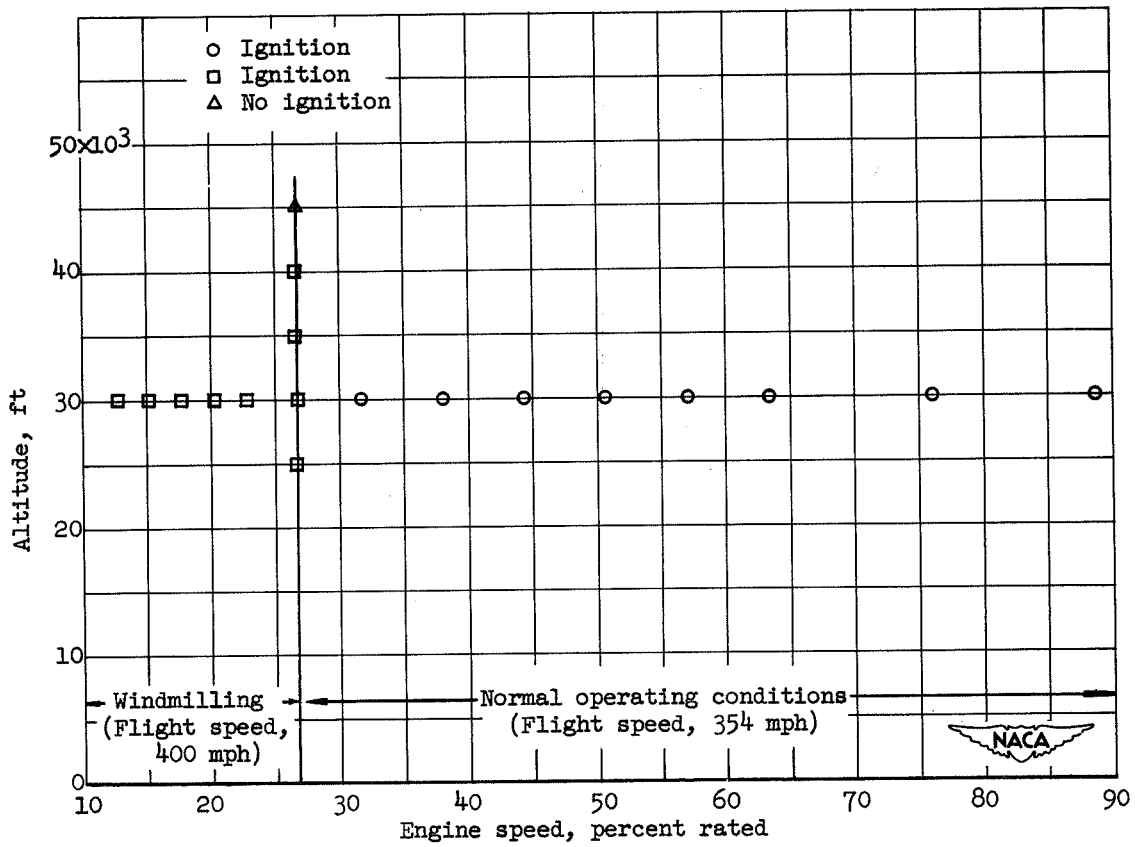
Figure 6. - Altitude-ignition trials with fuel MIL-F-5572, grade 115/145 (weathered).
