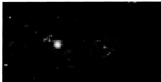
16-m LST, t~3 ksec
