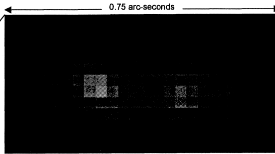
HST 2.4-m, t~900 ksec
