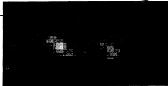
8-m LST, t~25 ksec
