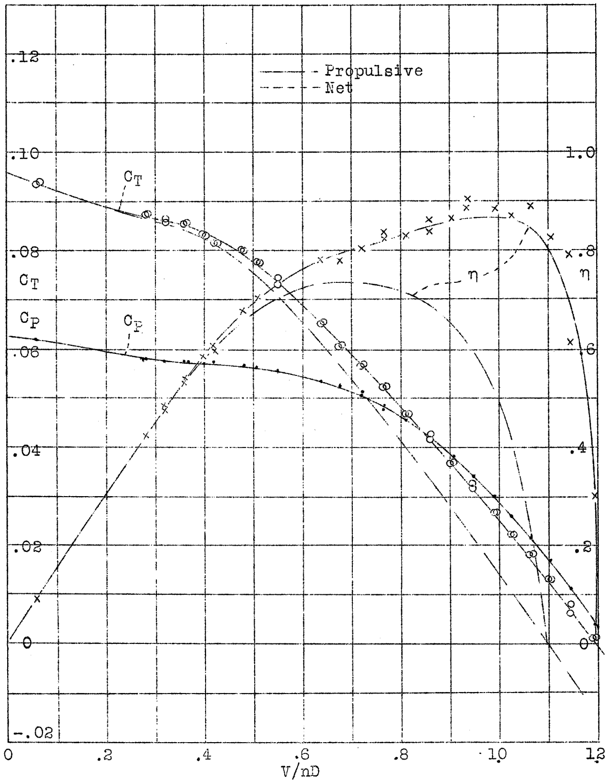
Figure 8.- Nacelle 15^\circ to chord; wing 0^\circ yaw, R.H. propeller No. 4412, Dia. 4 ft, Set 23^\circ , at .75 R.
