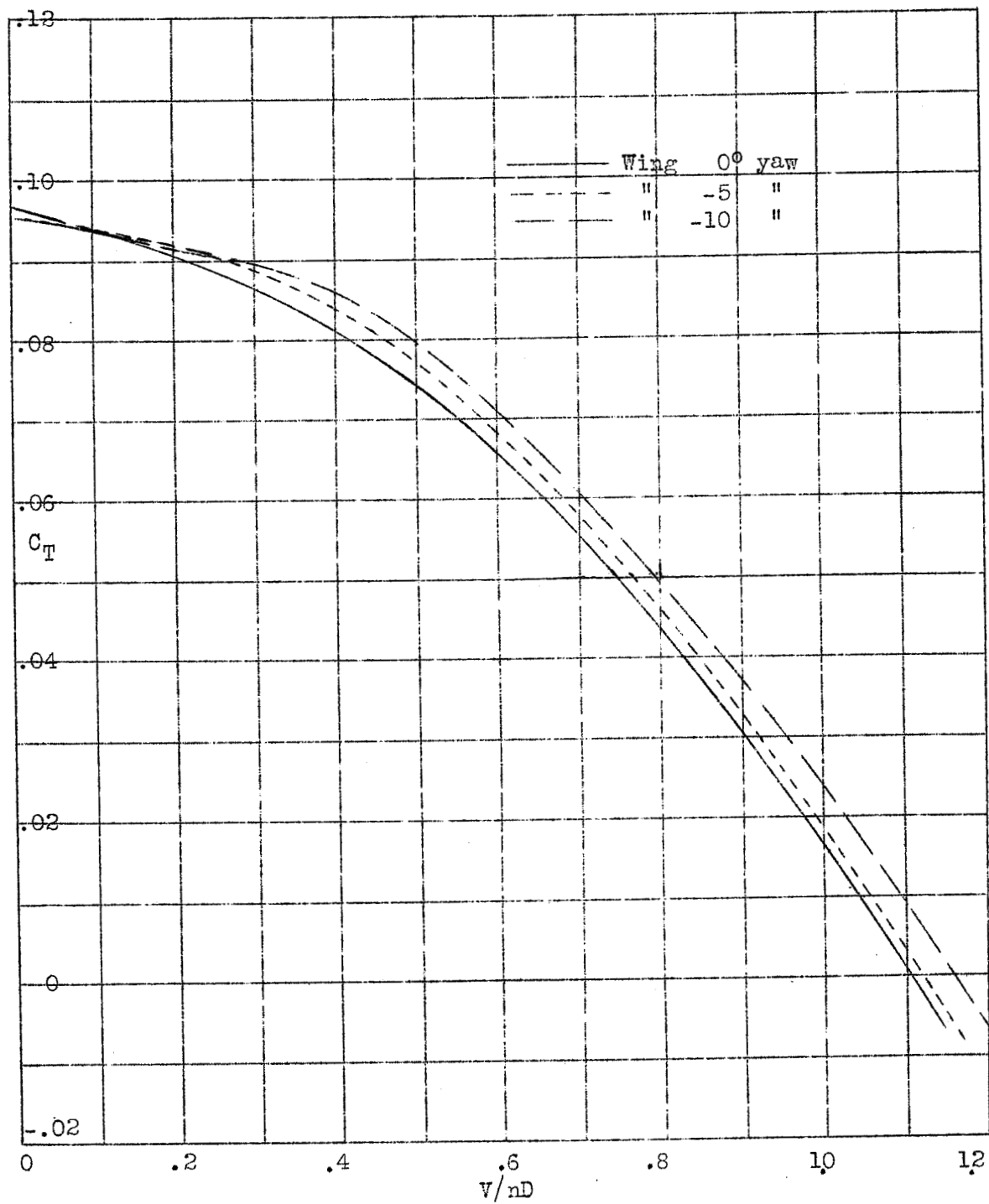
Figure 11.- Nacelle parallel to chord; propulsive thrust, R.H. propeller No. 4412, Dia. 4 ft., Set 28^\circ , at .75R.
