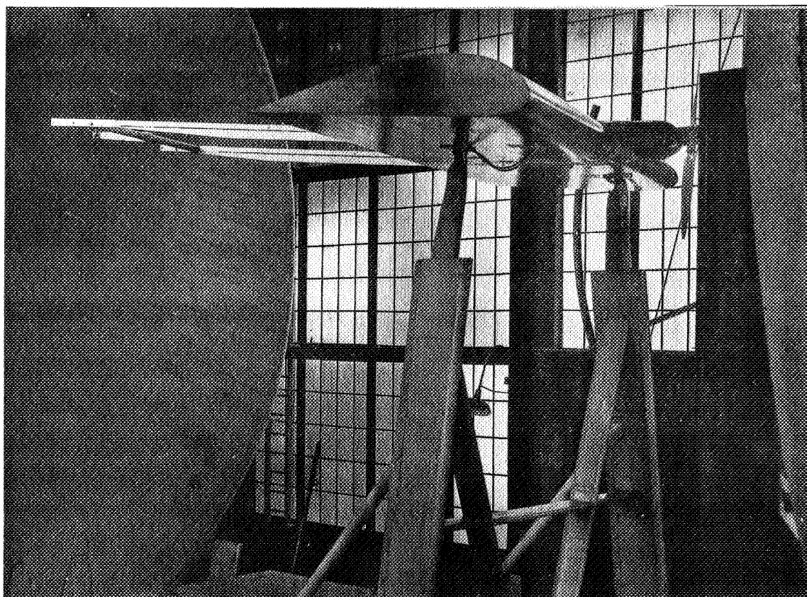
Figure 2.-Nacelle 15^{\circ} to chord; wing -20^{\circ} yaw.
