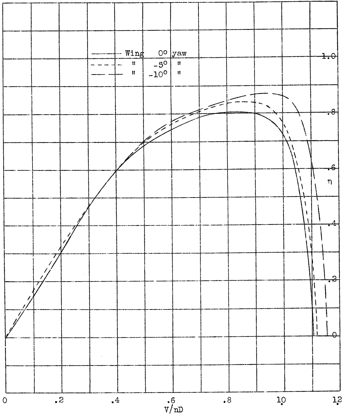
Figure 13.- Nacelle parallel to chord; propulsive efficiency, R.H. propeller No. 4412, Dia. 4 ft., Set 22°, at .75R.
