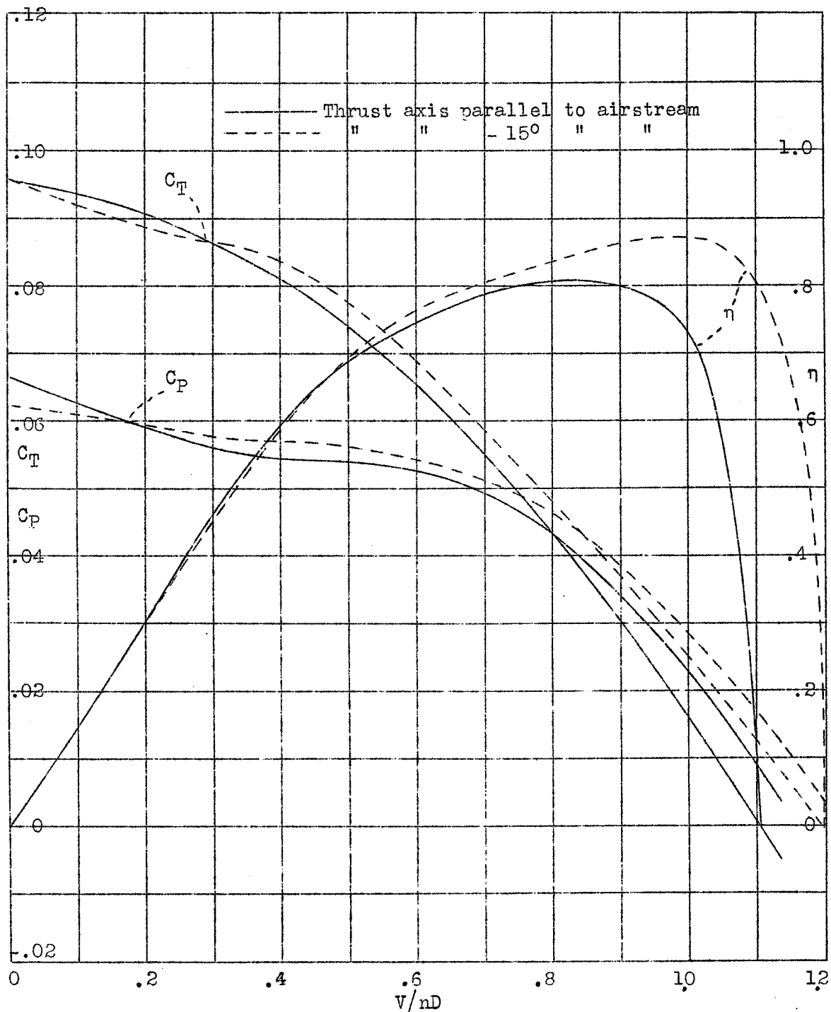
Figure 19.- Wing 0° yaw; propulsive curves, R.H. propeller No. 4412, Dia. 4 ft., Set 22° , at .75R .
