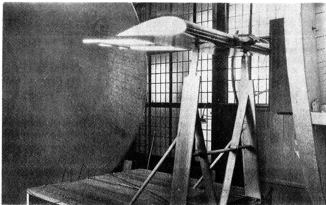
Figure 1.-Nacelle parallel to chord; wing -10^{\circ} yaw.
