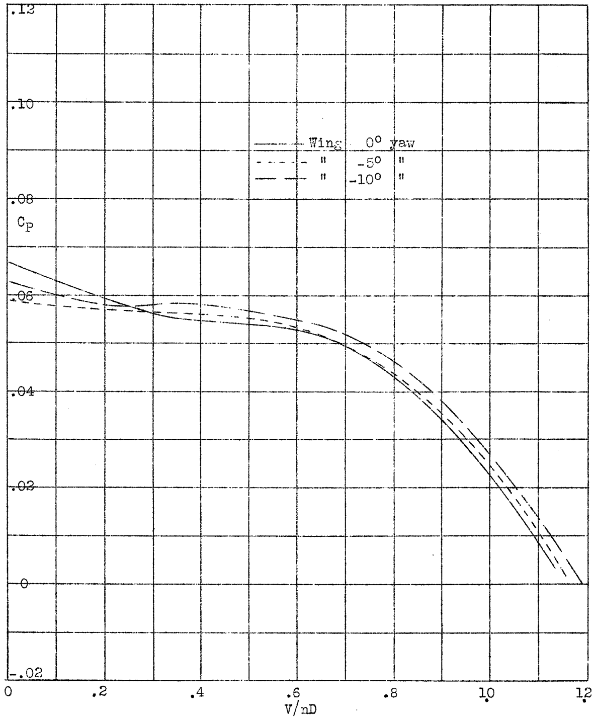
Figure 12.- Nacelle parallel to chord; power, R.H. propeller No. 4412, Dia. 4 ft., Set 22°, at .75R.
