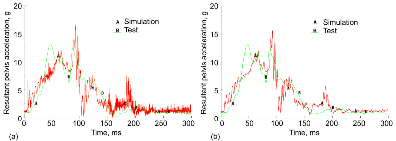
Figure 13.—Pelvis acceleration of Hybrid III physical and finite element dummies. (a) Unfiltered. (b) Filtered at 180 Hz.
