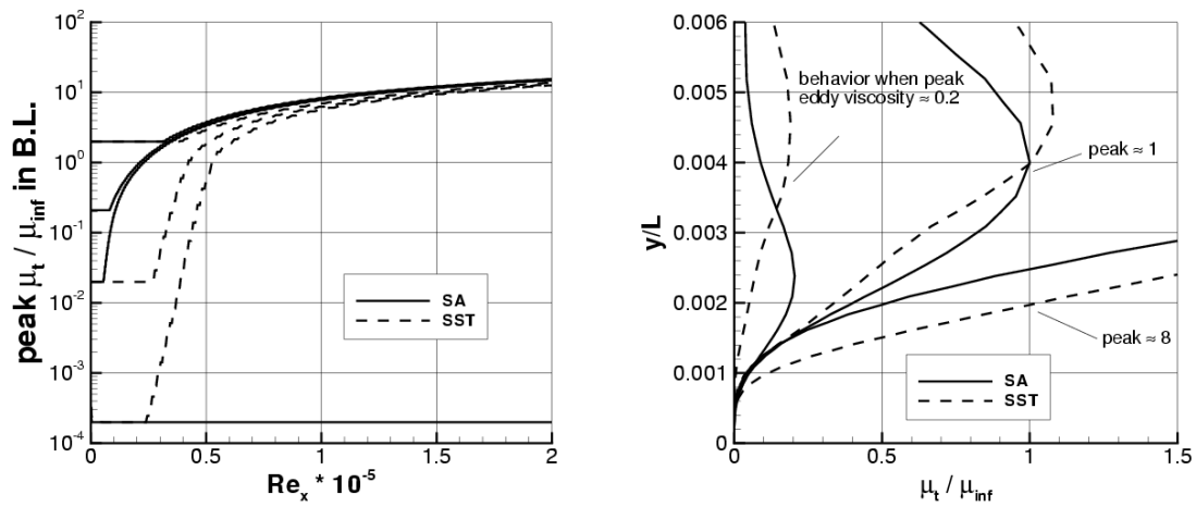
Figure 8. Eddy viscosity over flat plate, M = 0.2 , medium grid; (a) peak value for various freestream turbulence levels; (b) vertical profile at locations where peak \mu_t / \mu_\infty \approx 0.2, 1.0, \text{ and } 8.0 .
