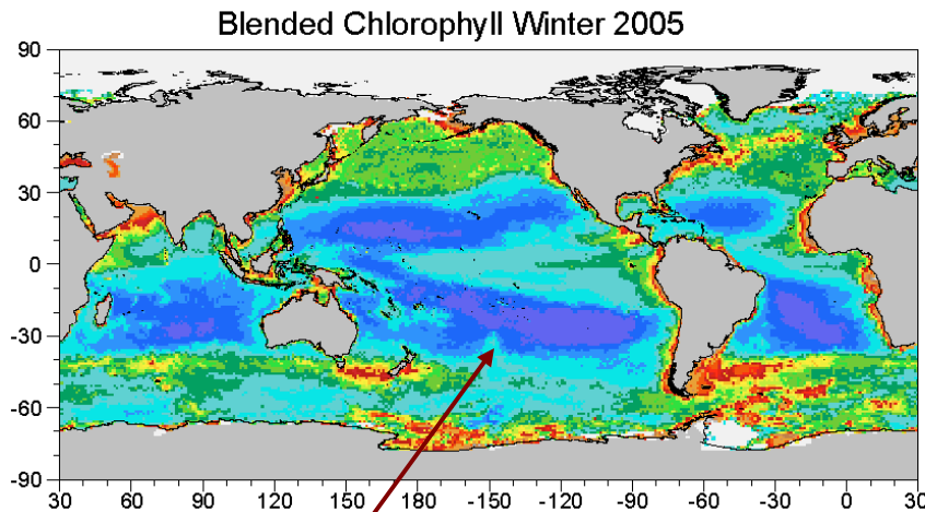
Figure 1. Example of the Blended Analysis for in situ data quality control. A north-south set of data from a single cruise in winter 2005 produced major distortion of the biological structure in the South Pacific. Adjustments from the Blended Analysis showed the cruise track in the blended chlorophyll, denoted by the arrow. The perturbations are apparent in the difference field, and align with the cruise track.
