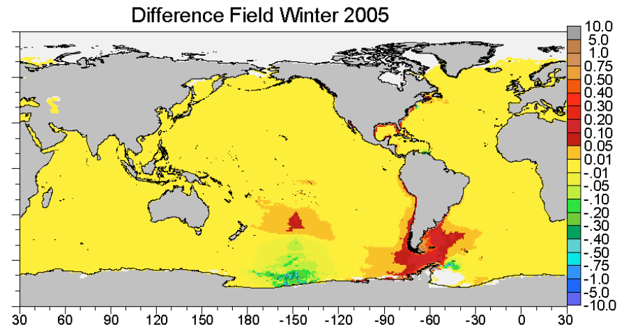
Figure 1. Example of the Blended Analysis for in situ data quality control. A north-south set of data from a single cruise in winter 2005 produced major distortion of the biological structure in the South Pacific. Adjustments from the Blended Analysis showed the cruise track in the blended chlorophyll, denoted by the arrow. The perturbations are apparent in the difference field, and align with the cruise track.
