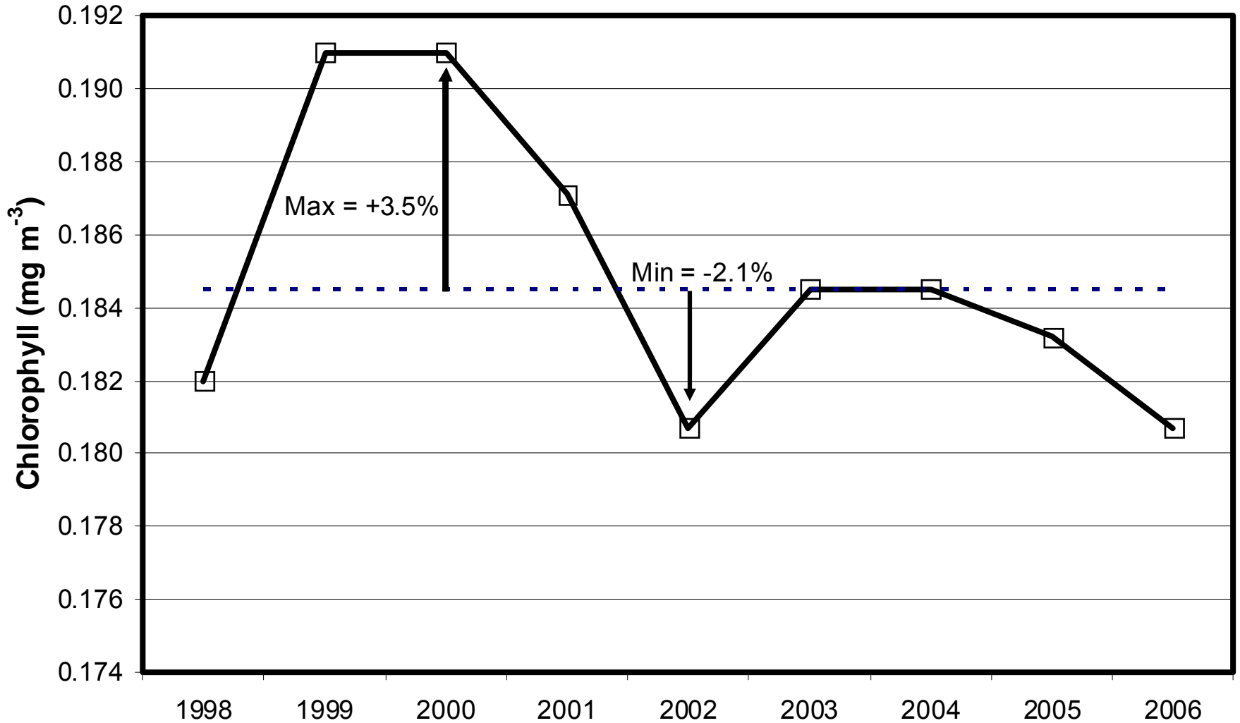
Figure 3. Global annual median global chlorophyll for the 9-year chlorophyll time series for SeaWiFS. The dashed line represents the climatological median. Minimum and maximum departures from the climatology are shown.
