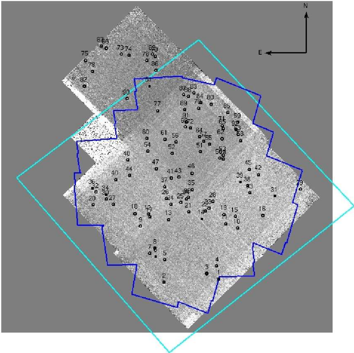
Fig. 1.— WFPC2 drizzled U-band image overlaid with UDF(cyan) and ACS/SBC(blue) footprints. Note the large number of detections in the second rectangular region from the top of the image due to a higher net exposure time for this region.
