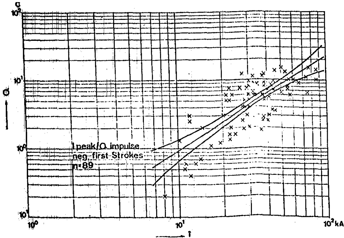
Figure 7.1-3. Scatter Plot of Impulse Charge, Q, Versus Return-Stroke Peak Current, I (Note: Both Vertical and Horizontal Scales are Logarithmic - The Best Fit to Data, I = 10.6 Q^{0.7} , Where Q is in Coulombs and I is in Kiloamperes, was used in Deriving Equation (1) - Adapted From Berger 8 )
