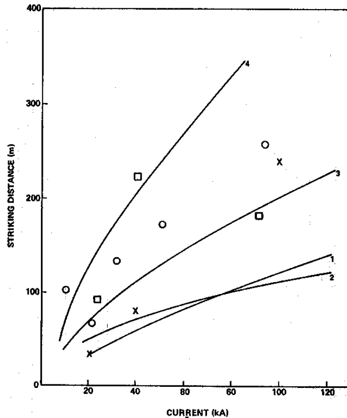
Figure 7.1-4. Striking Distance versus Return-Stroke Peak Current: Curve 1, Golde 9 ; Curve 2, Wagner 10 (1963); Curve 3, Love 11 ; Curve 4, Rühling 12 ; X, theory of Davis 13 ; 0, Estimates from Two-Dimensional Photographs by Eriksson 14 ; □, Estimates from Three-Dimensional Photography by Eriksson 15 (Adapted from Golde and Eriksson as Referenced Above)
