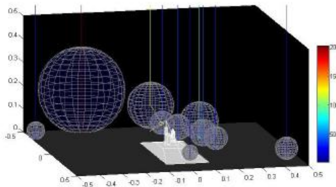
Figure 6. Positive strikes to the pad using spheres to illustrate the algorithm. Note the angle of inclination of the initially vertically traveling leader (yellow line) as it attaches to the catenary system.
