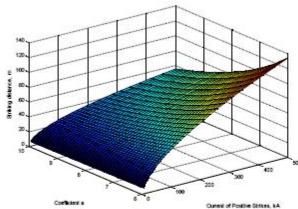
Figure 3. Striking distance as a function of positive stroke current peak and a_{(r)} .
