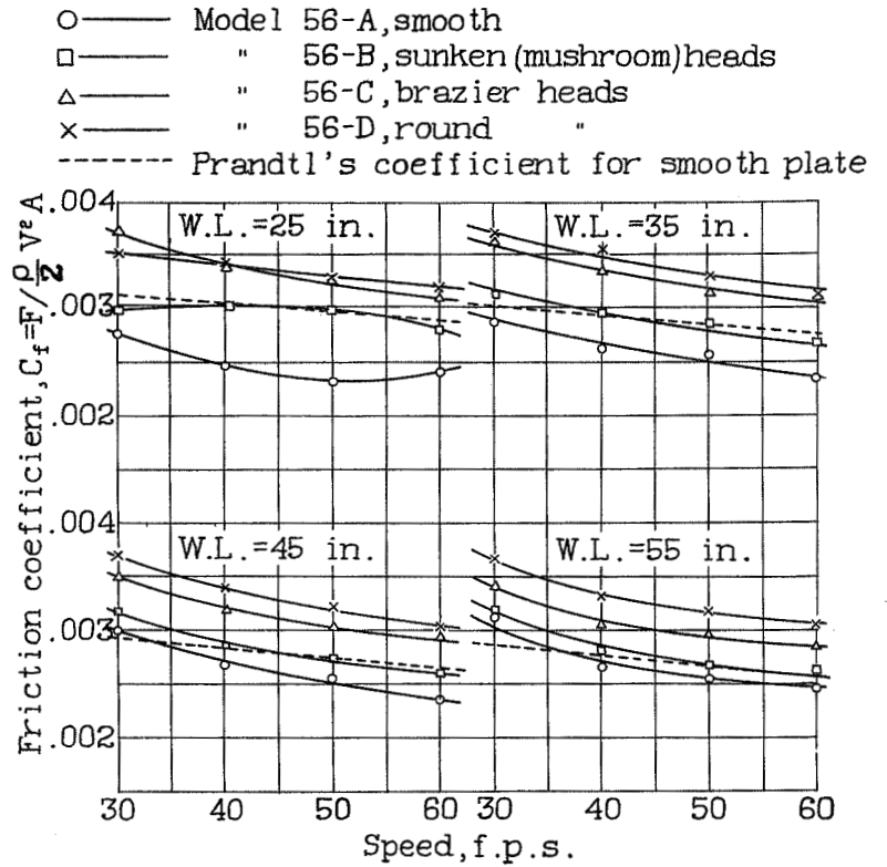
Figure 14. - Variation of friction coefficient with speed.
