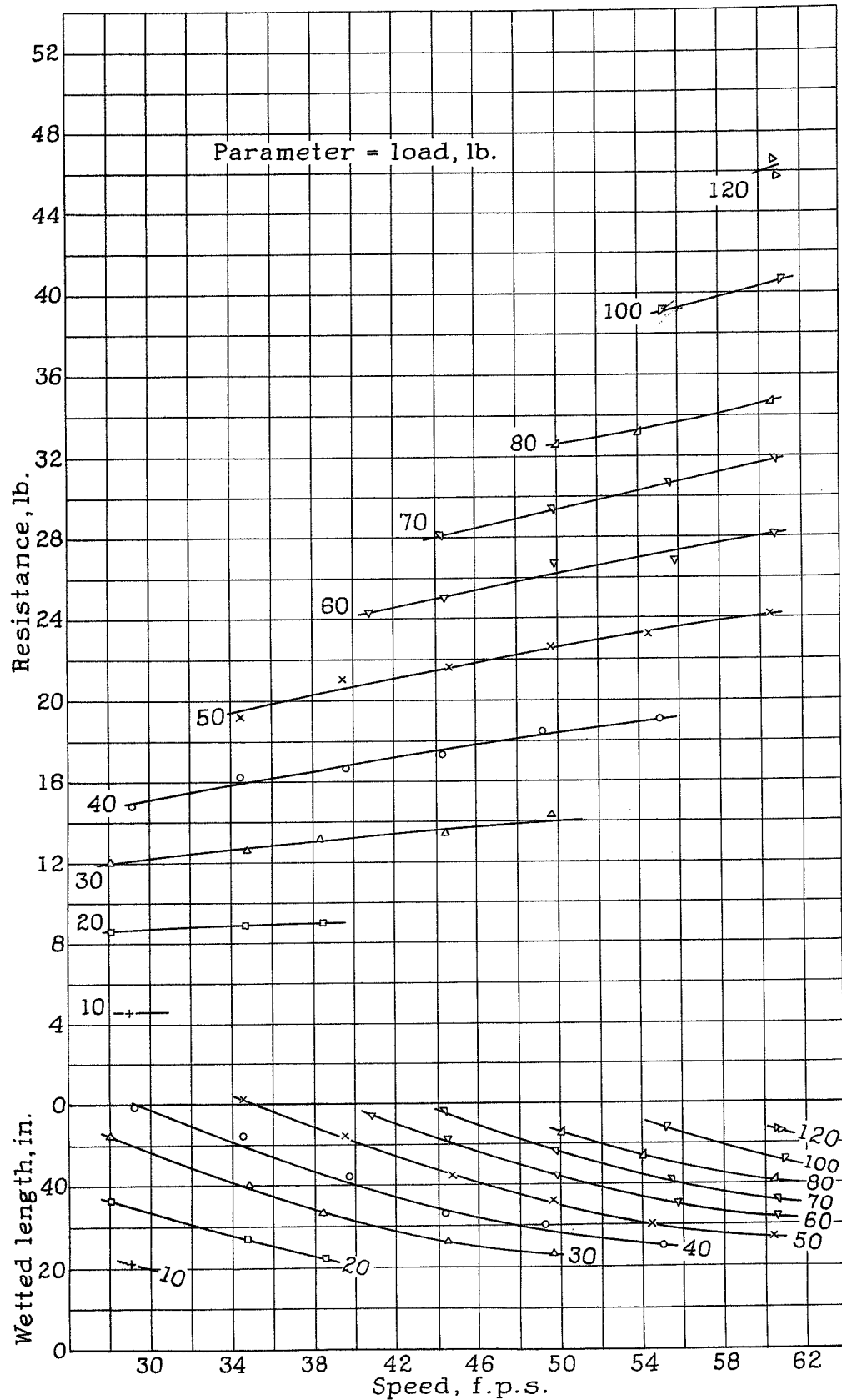
Fig. 7.- Model 56-B. Variation of resistance with speed. \tau = 1.5^\circ
