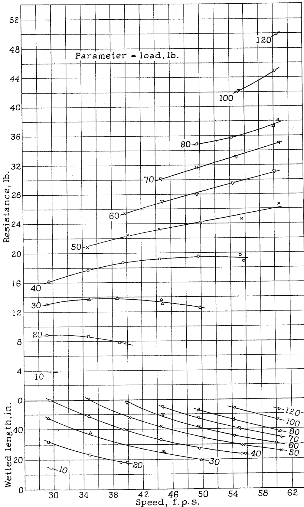
Fig. 9.- Model 56-C. Variation of re- sist- ance with speed. \tau = 1.5^\circ
