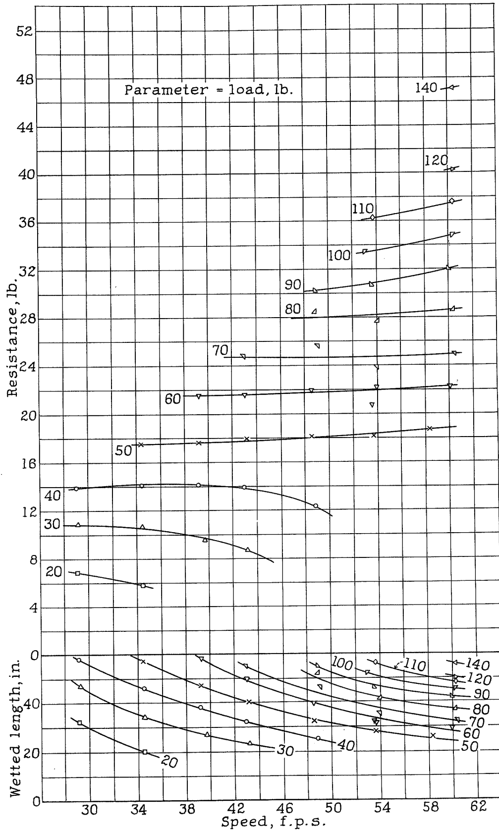
Fig. 5.- Model 56-A. Variation of re- sist- ance with speed. \tau = 1.5^\circ
