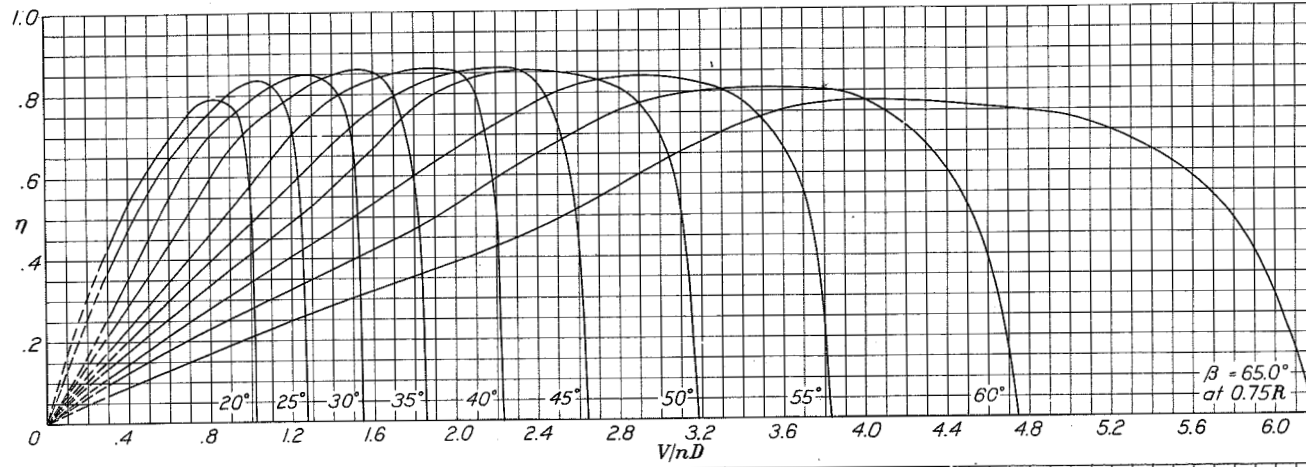
Figure 28.- Efficiency curves for six-blade single- rotation propeller with wing.
