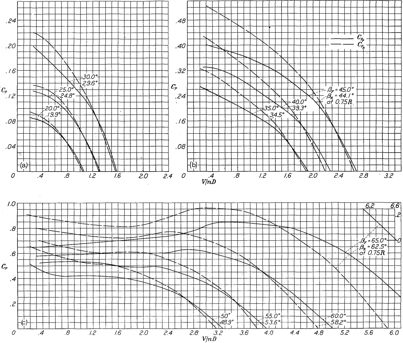
Figure 33a,b,c. Individual power-coefficient curves for six-blade dual-rotation propellers with wing.
