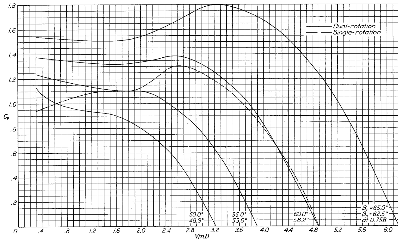
Figure 34c.- Power-coefficient curves for six-blade dual-rotation propellers with wing, showing superimposed curve for the corresponding single-rotation condition at 60° blade angle.
