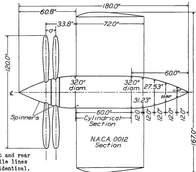
Figure 3.- Plan view showing dimensional details of wing and nacelle. Dimension a for four-blade propeller = 9.7" and for six-blade propeller = 10.0".
