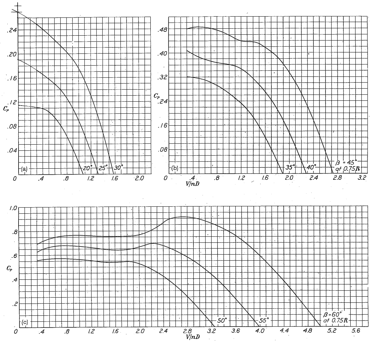
Figure 23.- Power-coefficient curves for four-blade single-rotation propeller with wing.
