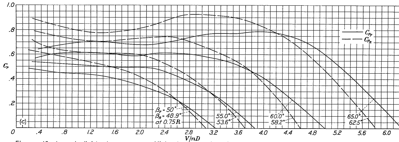
Figure 19a,b,c.-Individual power-coefficient curves for six-blade dual-rotation propellers without wing.
