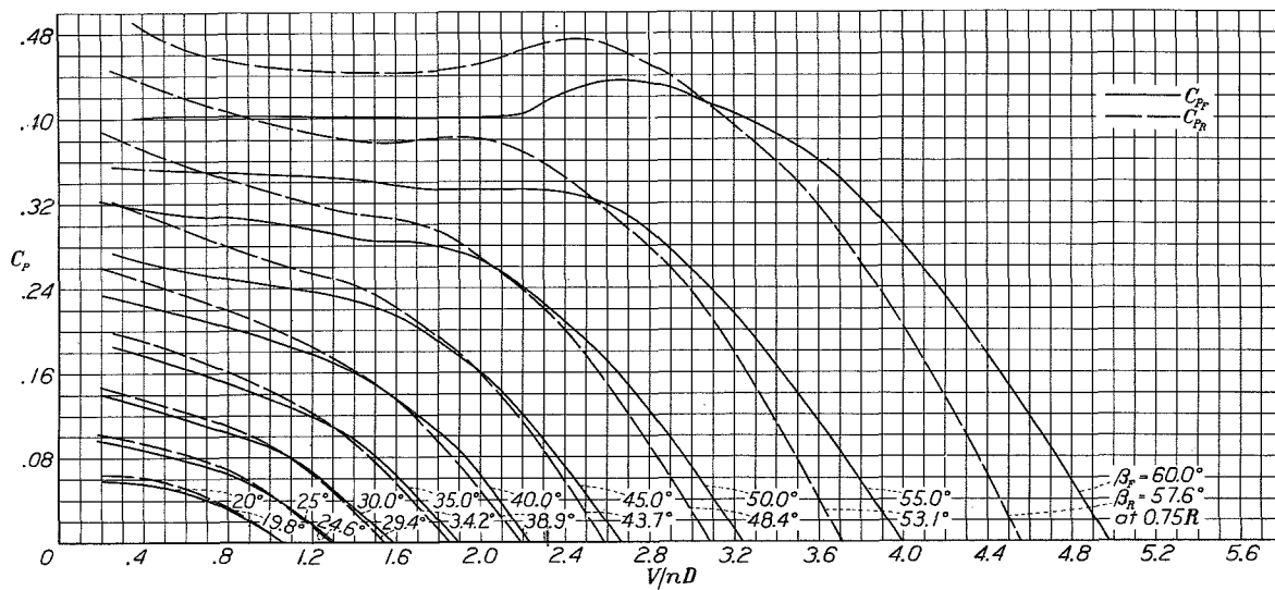
Figure 26.- Individual power- coefficient curves for four-blade dual-rotation propellers with wing.
