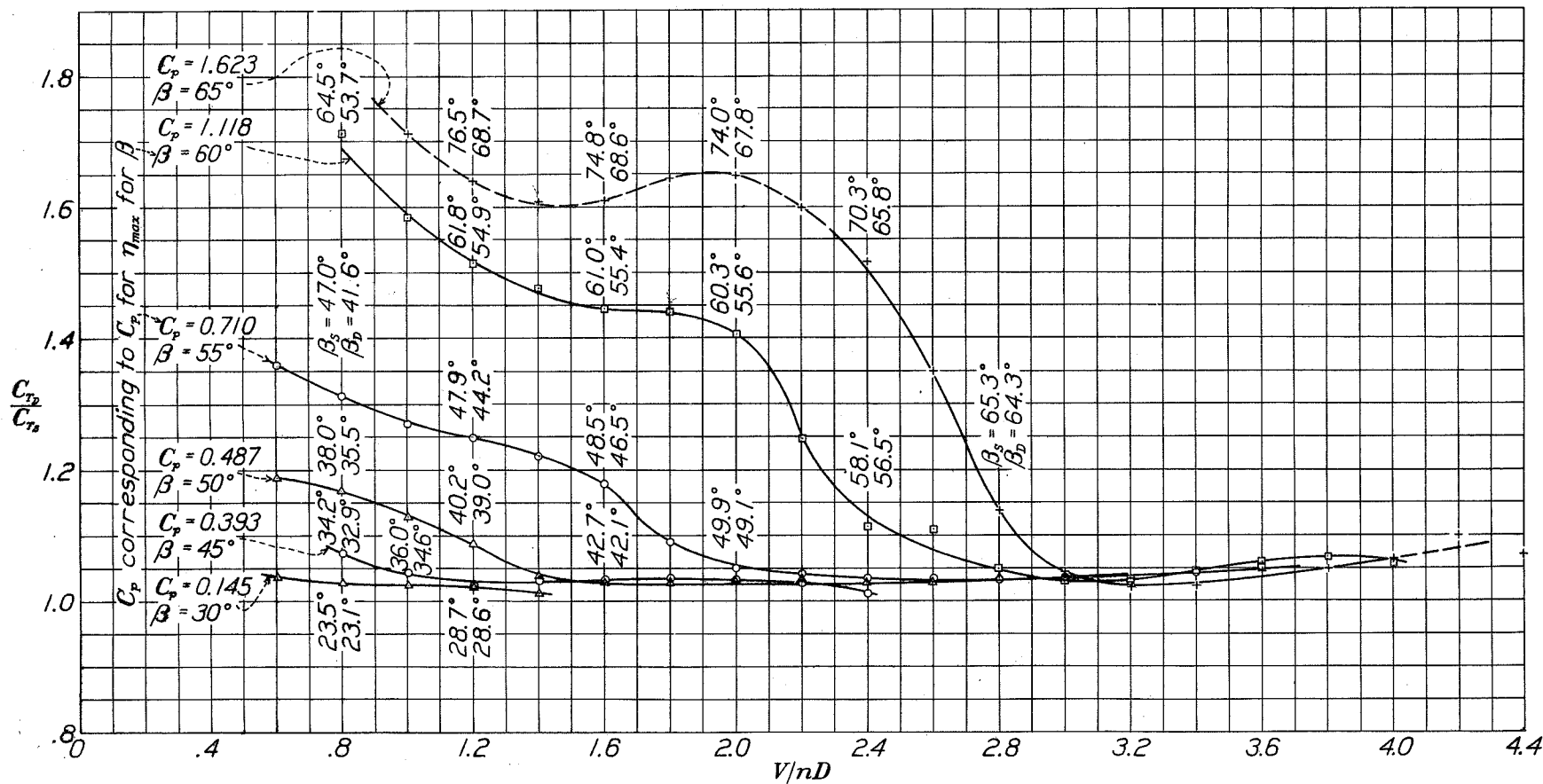
Figure 40.- Ratio of \frac{C_{T2}}{C_{T1}} for constant values of C_p . Six-blade propellers without wing.
