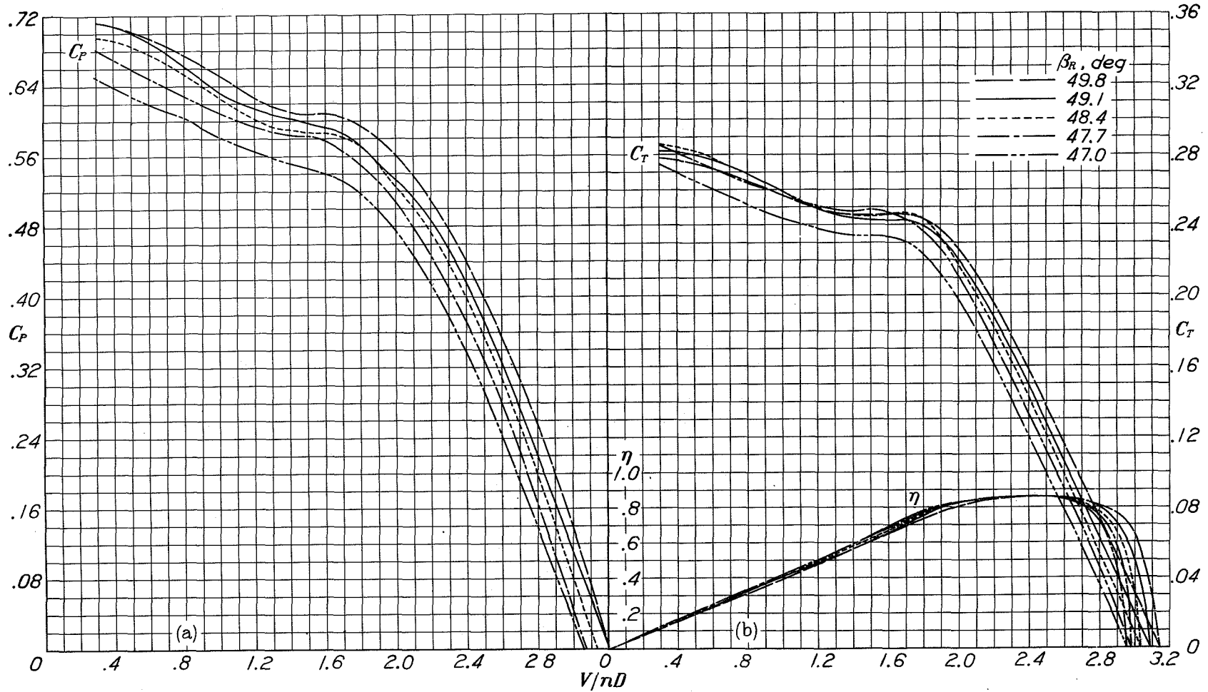
Figure 36.-Propeller curves showing the effect of small variations in rear blade angle at a front blade angle of 50°. (Four-blade dual-rotation propellers without wing.)
