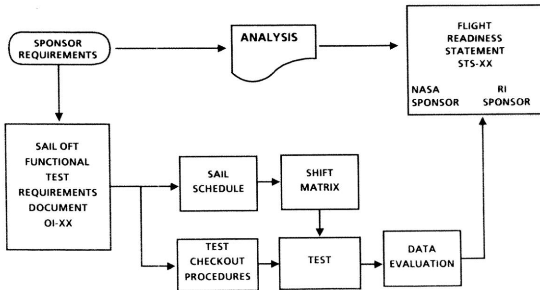
Figure 5.3-9. SAIL Verification Process Flow
