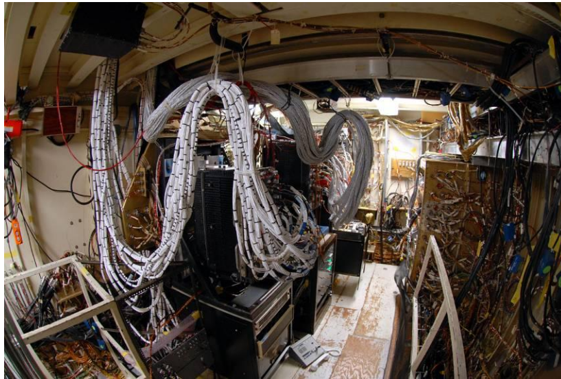
Figure 5.3-5. Aft Avionics Bays with Two SSME Controllers
