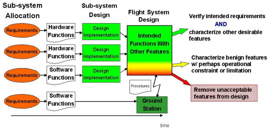
Figure 5.1-1. Flight System Development Process
