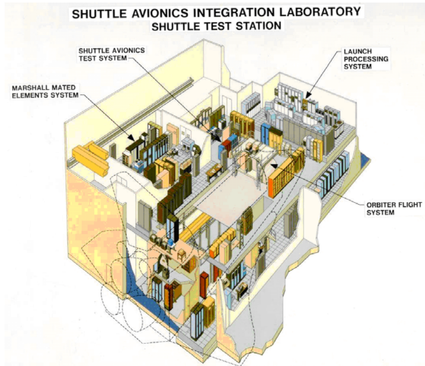
Figure 5.3-3. Shuttle Test Station, including the SAIL Flight System
