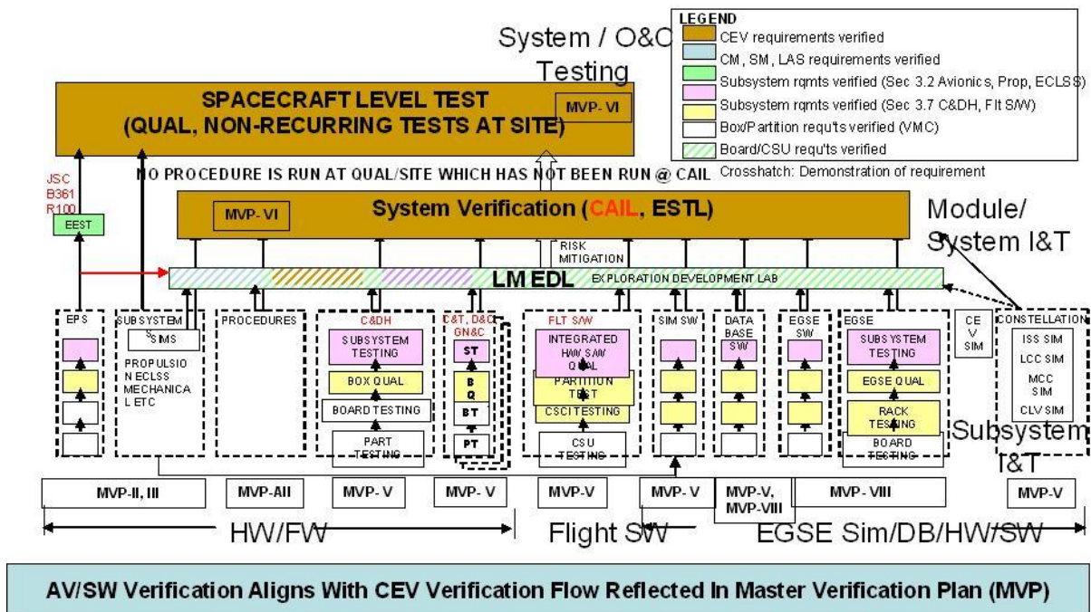
Figure 5.4-1. CEV Development Flow
