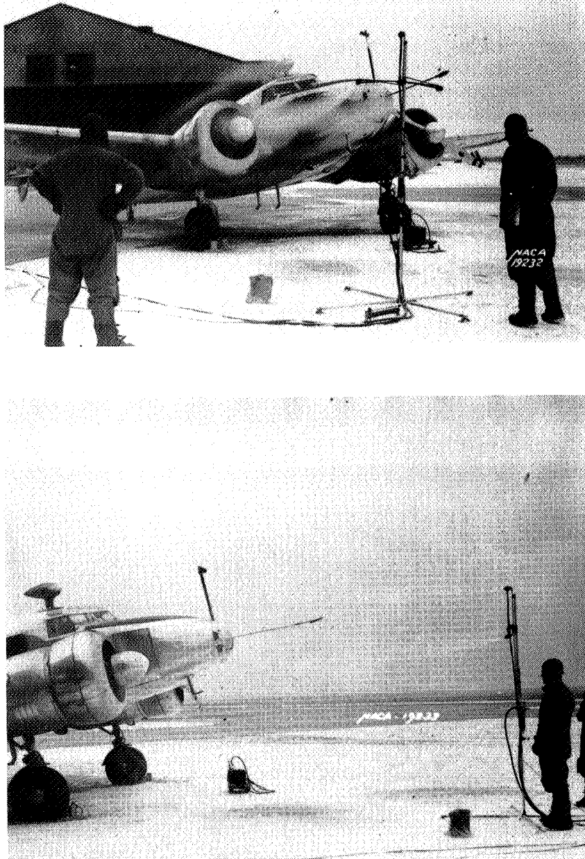
Figure 1.- Two views of Lockheed 12A airplane. Ice was formed on the rotating propellers of the airplane while on the ground.
