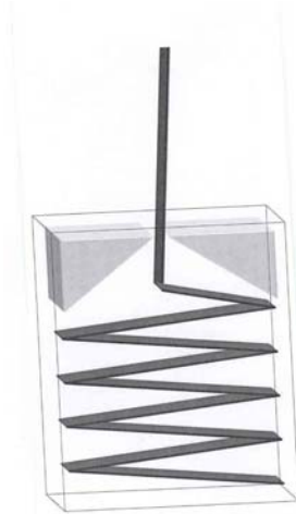
Figure 4. Concept drawing showing the Fortissimo tape tether stored and being deployed from an open-ended box.
