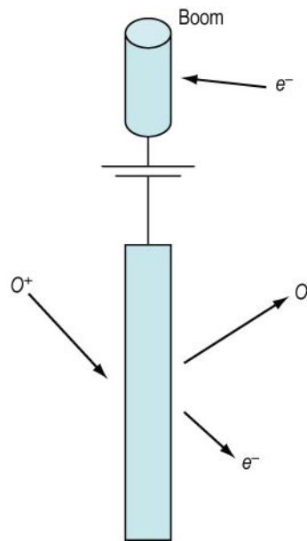
Figure 2. Configuration for testing OML theory without the use of an active plasma contactor. The boom and tether are biased positive and negative, respectively.
