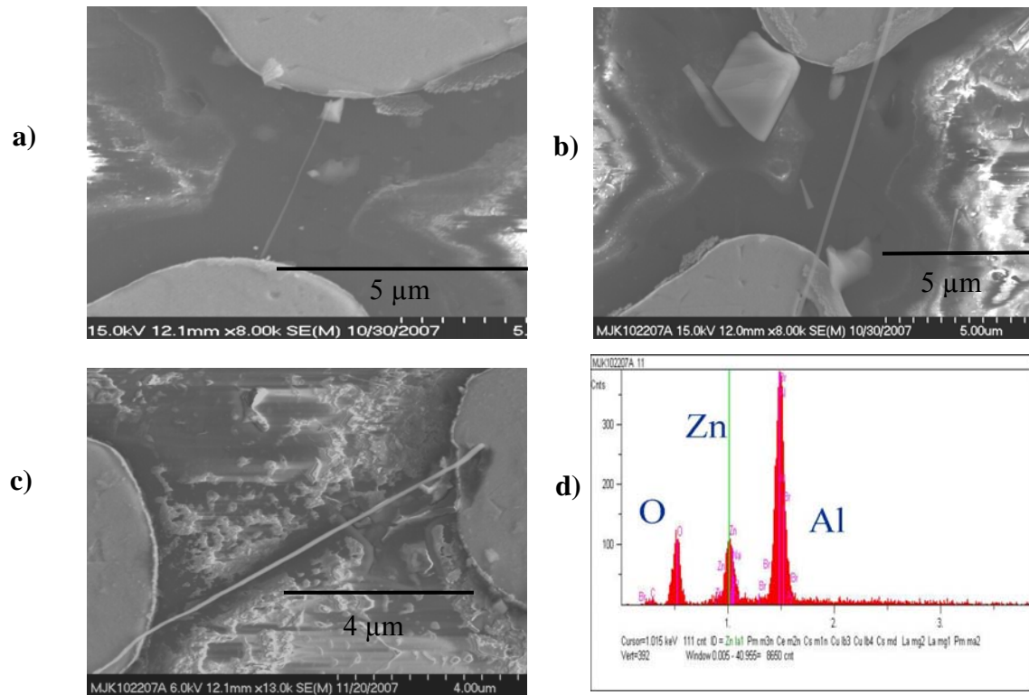
Figure 2. SEM micrographs of three different oxide nanostructures of various sizes on a single Al 2 O 3 substrate. a) SnO 2 nanowire with a diameter of 60 nm. b) In 2 O 3 nanowire with a diameter of 140 nm. c) ZnO nanowire with a diameter of 80 nm. d) Corresponding EDS analysis of the ZnO nanowire in Figure 2c verifying the elemental configuration of the nanowire and substrate.
