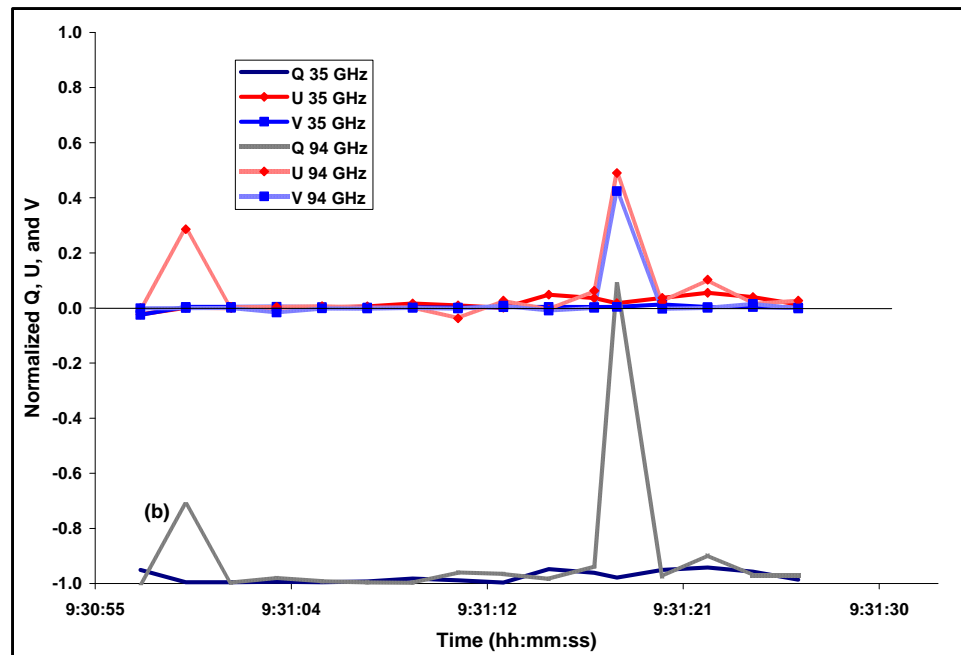
Fig. 9. a) Plot of 35 GHz and 94 GHz signal strength for a terrestrial area consisting of a creek and flood plain. b) normalized Q, U, and V values corresponding to the values in (a).
