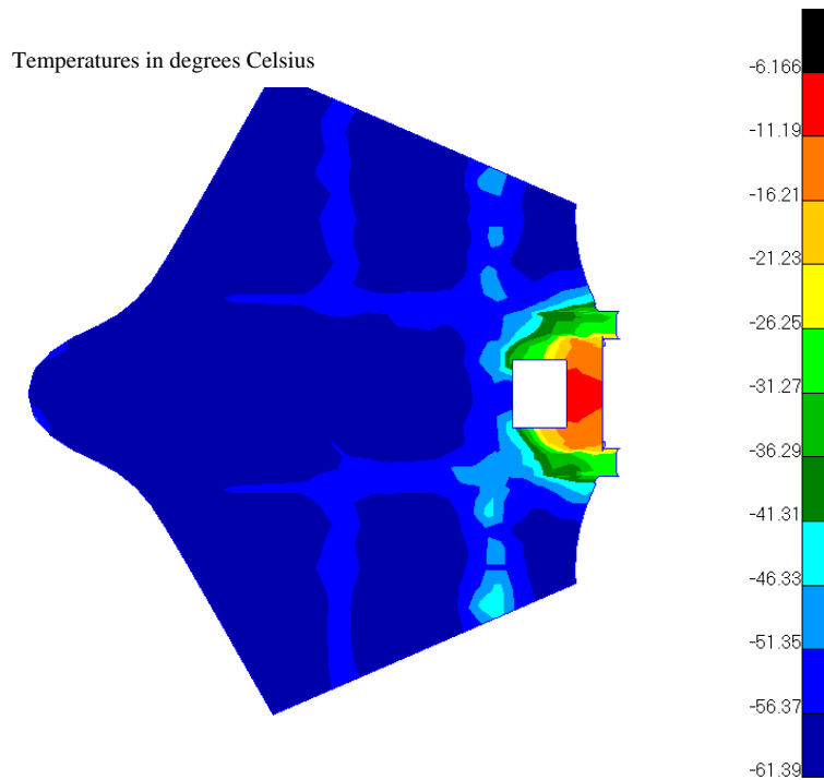
Figure 21. Temperature profile of lower fuselage with heat shield. (Max T = -6.17°C).
