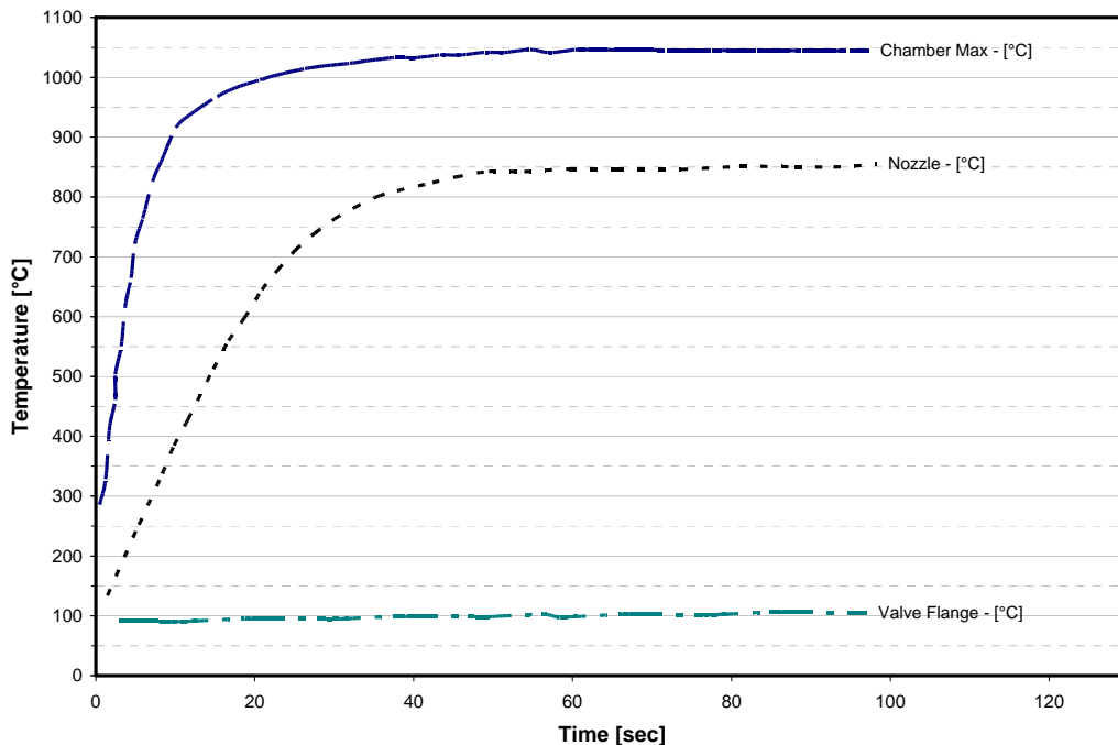
Figure 19. Hot Fire Test Data for AMPAC-ISP 22N Thruster 9 .
