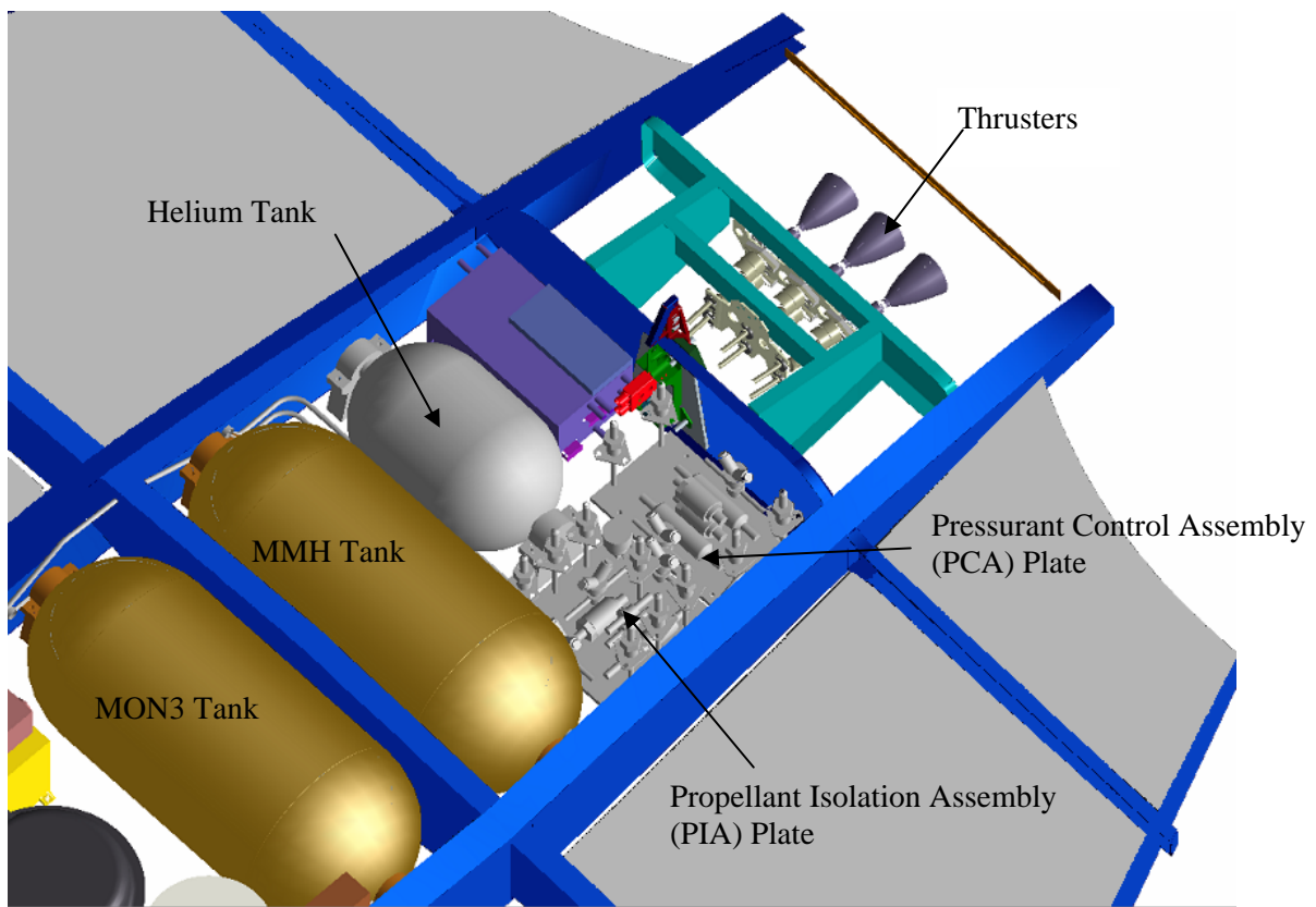
Figure 18. Propulsion System / Airframe Integration
