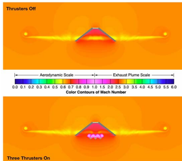
Figure 22. Rear view of Airplane showing airplane in coast (above) and with thrusters firing (below)
