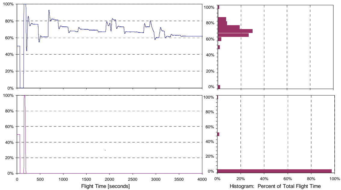
Figure 24. Thruster Duty Cycles for No Turbulence Conditions
