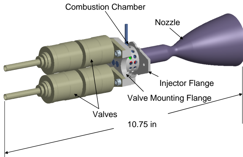
Figure 8. AMPAC-ISP 22N Thruster Details
