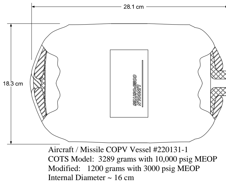
Figure 6. Helium Composite Over-wrapped Pressure Vessel
