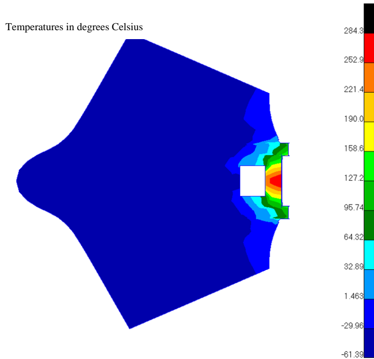
Figure 20. Temperature profile for lower fuselage without heat shield. (Max Temperature = 284°C).
