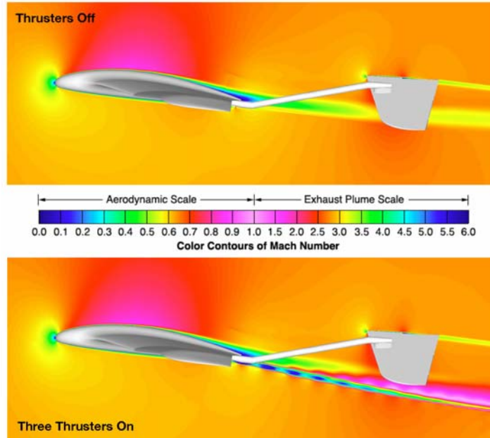
Figure 23. Side view of Airplane showing airplane in coast (above) and with thrusters firing (below).
