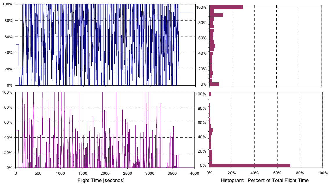
Figure 25. Thruster Duty Cycles for Severe Turbulence Conditions
