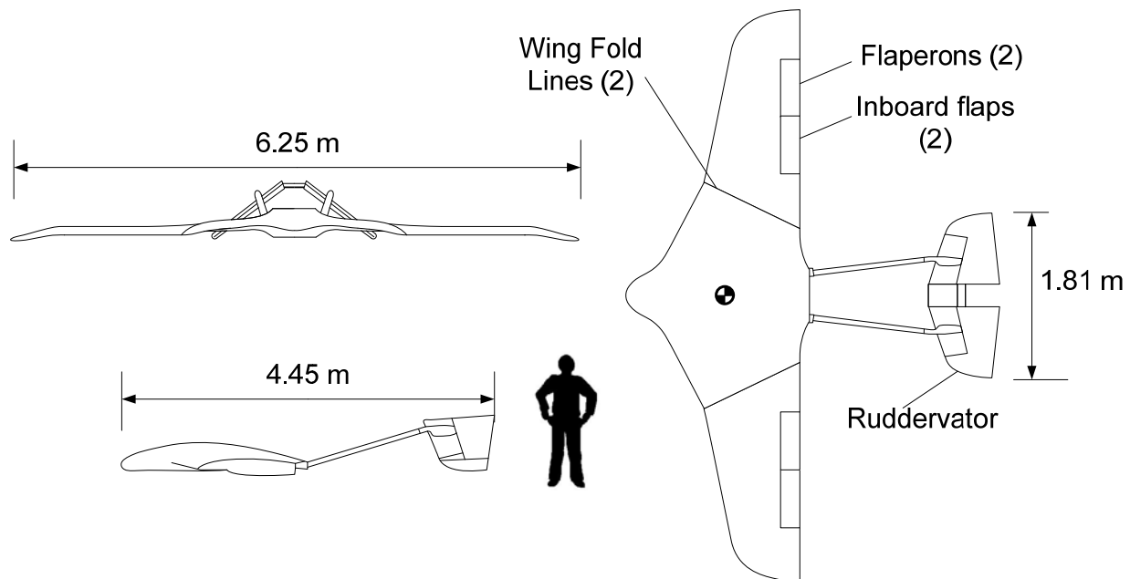
Figure 4. ARES Airplane Geometry
