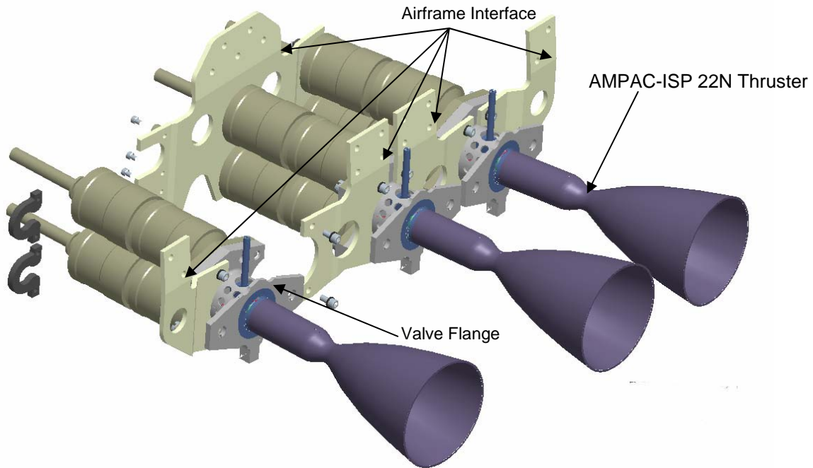
Figure 10. Triple 22N In-Line Thruster Mounting and Assembly
