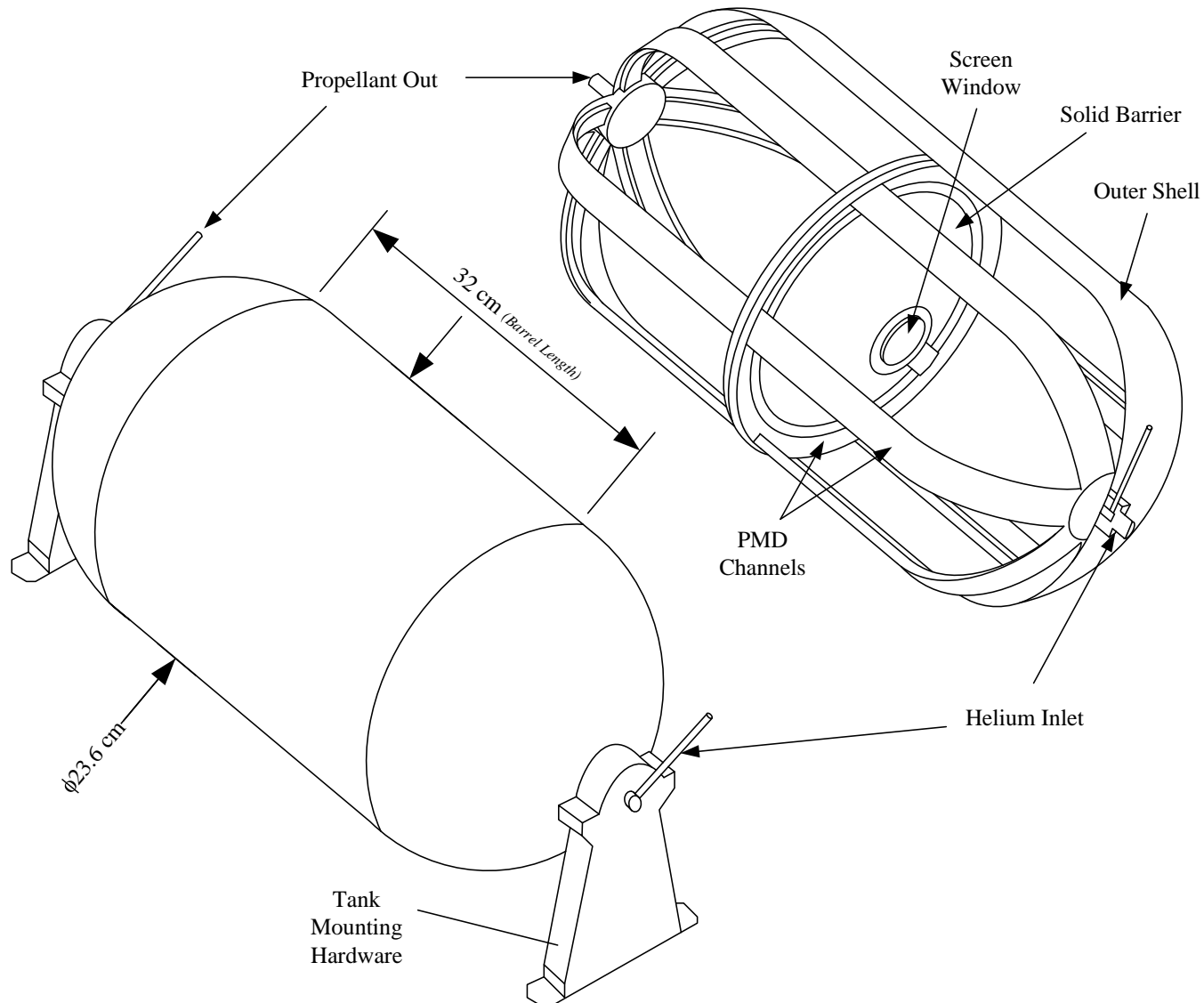
Figure 7. Propellant Tank and PMD Design
