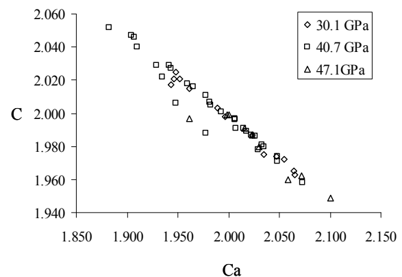
Figure 1. Plot of C (carbon) vs. Ca (calcium) from 42 quantitative EMP analyses of calcite in the 30.1, 40.7, and 47.1 GPa shock experiments. No significant carbon deviation from stoichiometric calcite compositions (based on 6 oxygens) that would indicate CO 2 degassing had occurred was detected.
