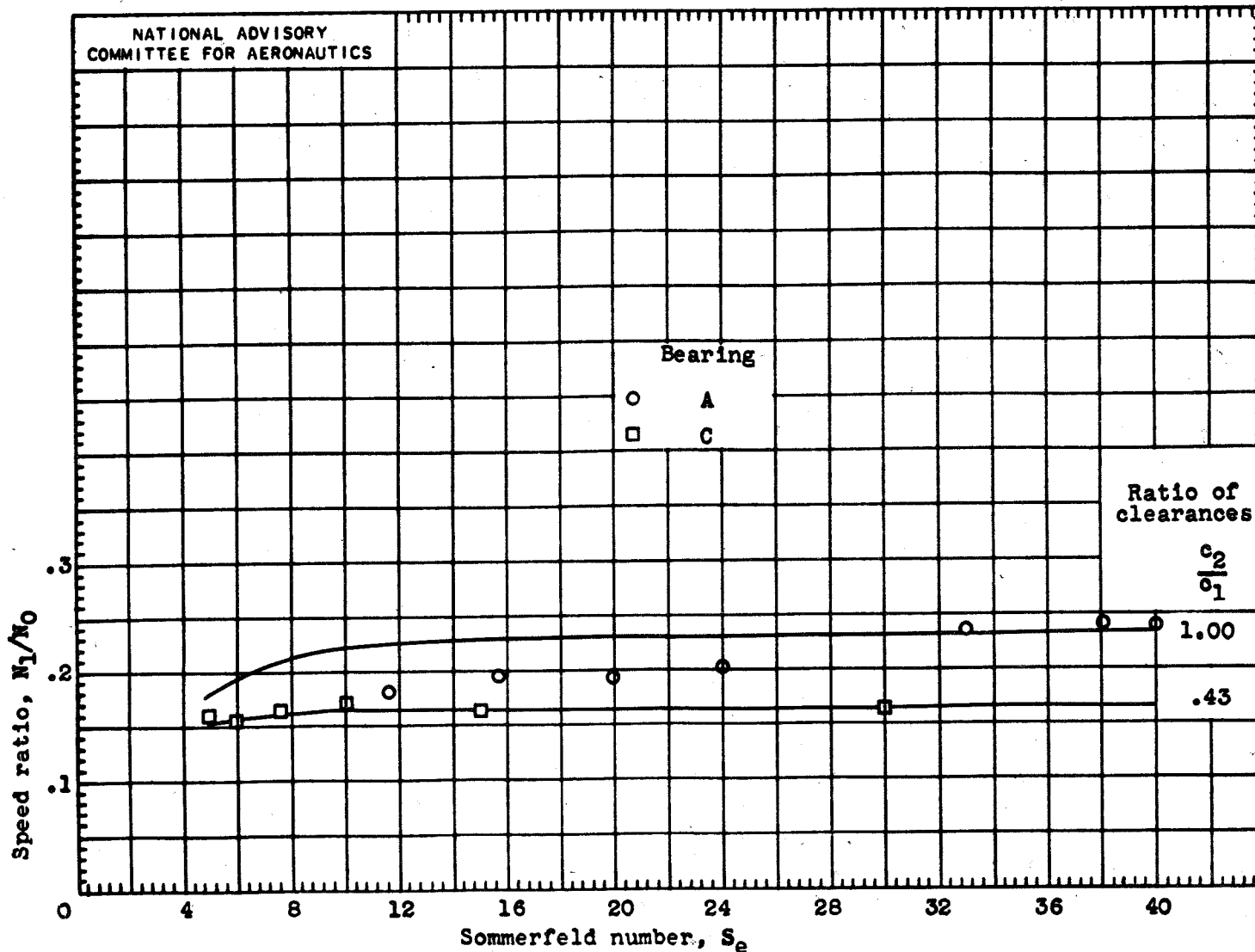
Figure 9. - Comparison of experimental and analytically determined values of speed ratio at different values of Sommerfeld number. Ratio of radii, 1.30.
