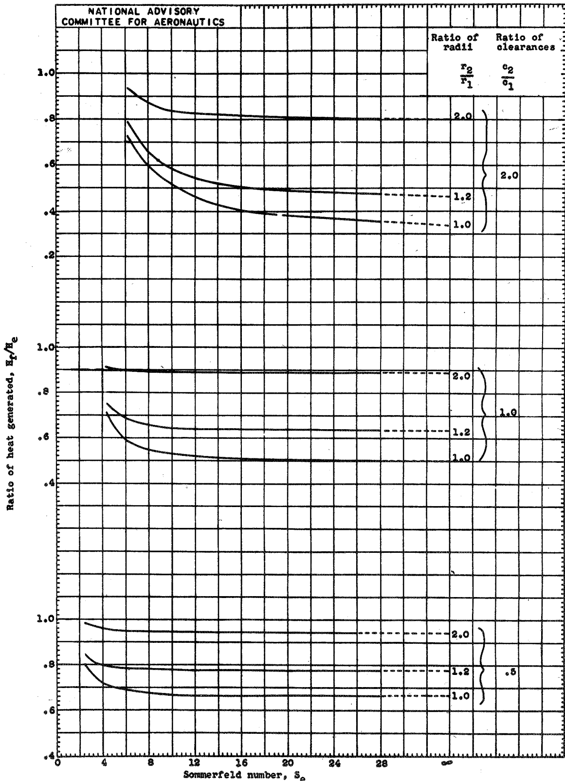
Figure 4. - Variation of ratio of heat generated in full-floating bearing to heat generated in an equivalent journal bearing with Sommerfeld number.
