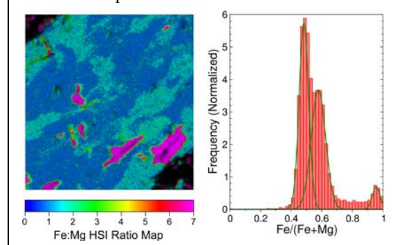
Figure 1. Left: HSI ratio map of a polished section of Copper Lake siderite showing a range of compositions from Mg -rich (blue) to Fe -rich (pink) (adapted from [7]). Right: Frequency distribution of compositions from image on left shows three compositional groups comprise this siderite sample.
