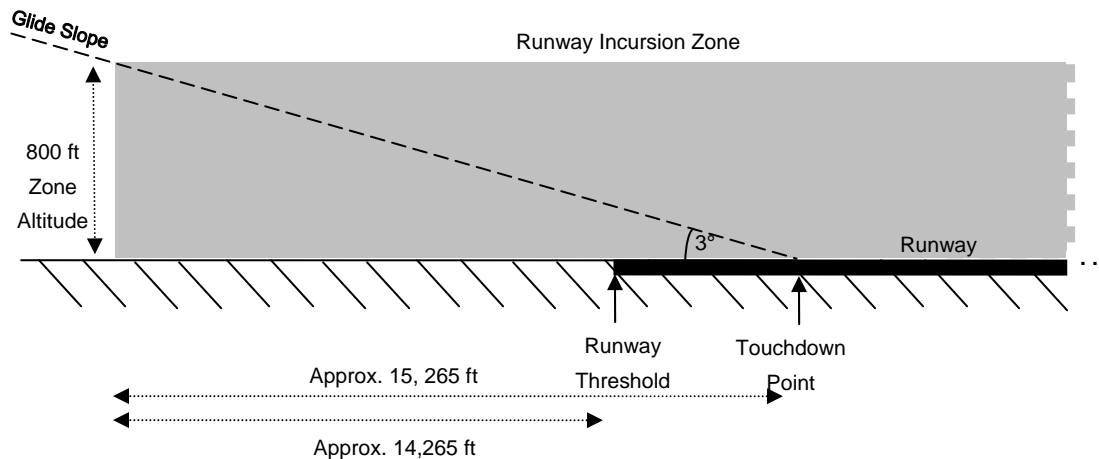
Figure 6. Example Using 3-Degree Glide Slope to Determine Incursion Zone Ends
