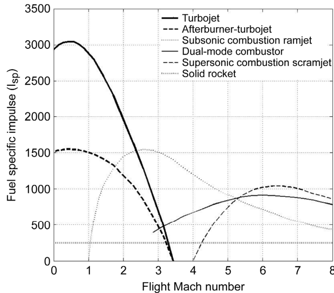
Figure 2.—Fuel specific impulse ( I_{sp} ) for various propulsion systems (Ref. 3).
