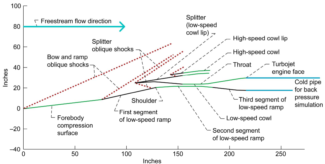
Figure 4.—Oblique shocks (dot traces) originating from the large-scale inlet to study mode transportation (L-IMX) forebody tip, forebody compression surface break point, the low-speed cowl lip, and the high-speed cowl lip.
