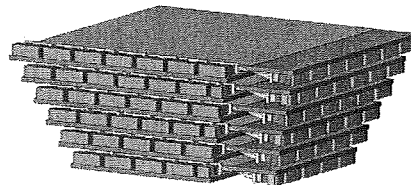
Fig. 2: The SOFTI detector concept.
