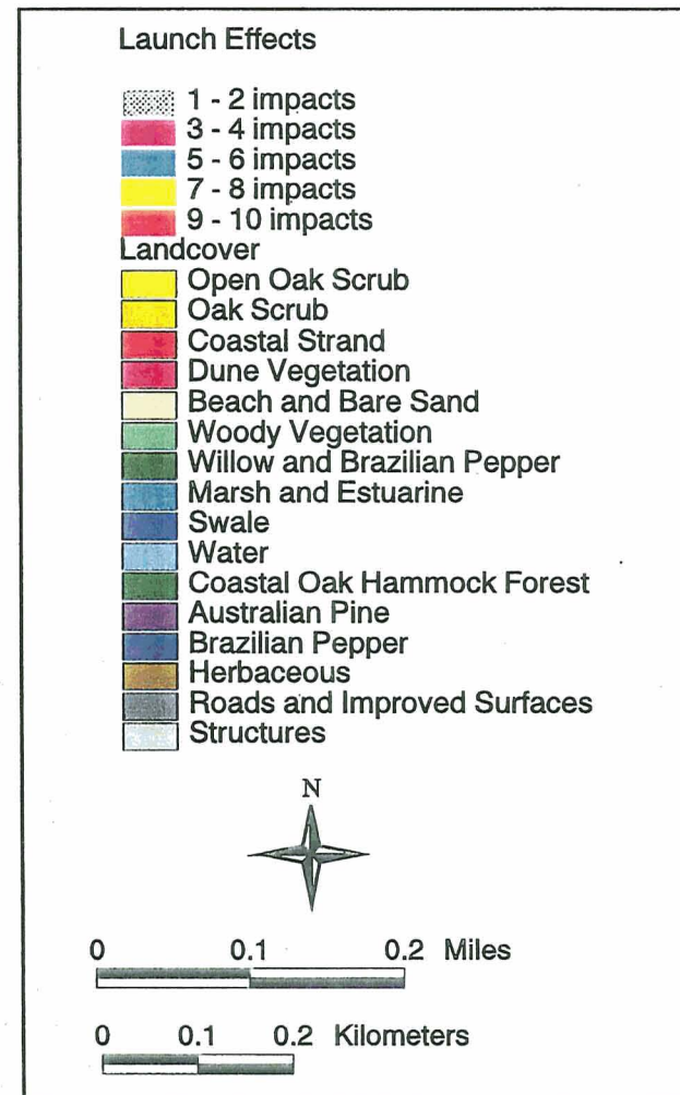
Figure 6: Vegetation and landcover impacted by Atlas Rocket launch effects within one kilometer of Atlas launch complex.
