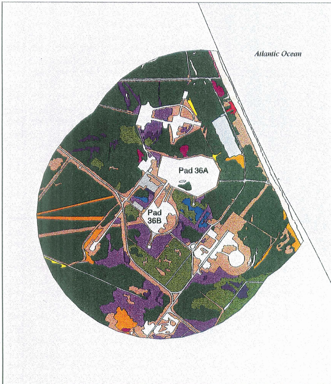
Figure 3: Vegetation and landcover within one kilometer radius of the Atlas launch complex.
