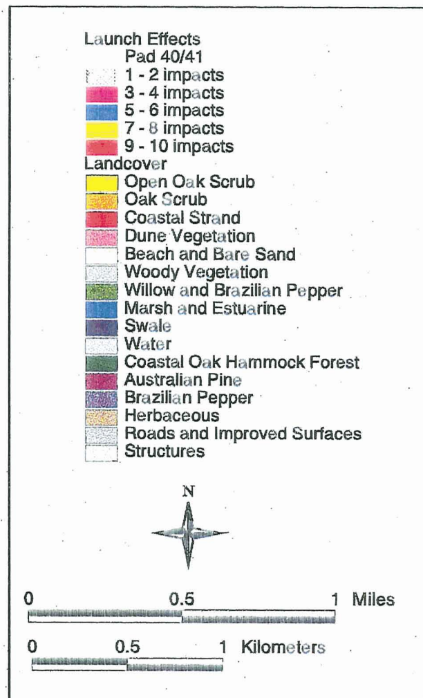
Figure 7: Vegetation and landcover impacted by Titan Rocket launch effects within one kilometer of Titan launch complexes and area in between.
