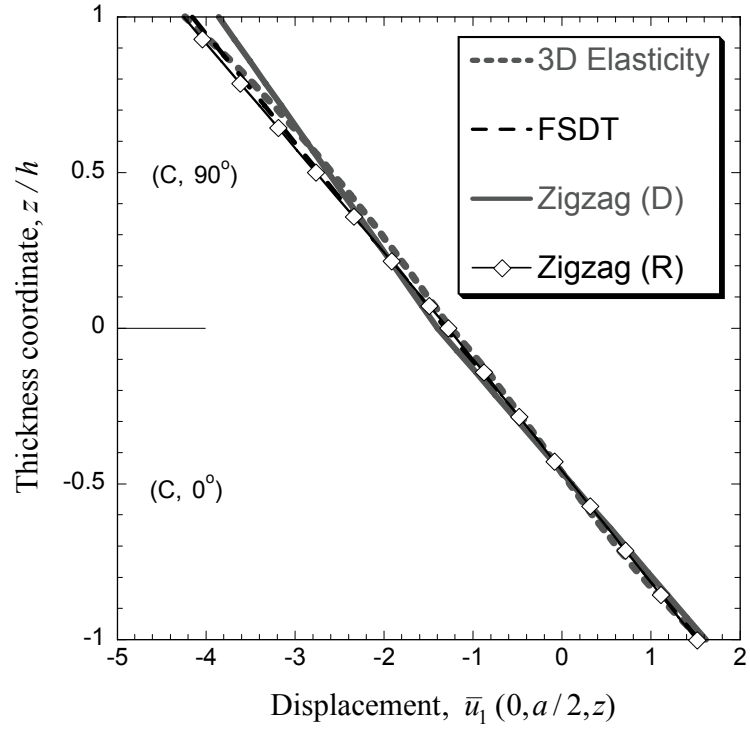
Figure 4. Normalized in-plane displacement for simply supported laminate A subjected to sinusoidal transverse pressure.
