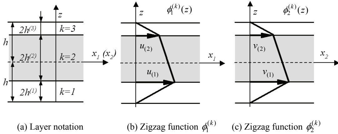
Figure 2. Notation for a three-layered laminate and \phi_1^{(k)} and \phi_2^{(k)} zigzag functions defined in terms of interfacial displacements, u_{(i)} and v_{(i)} ( i = 0, 1, \dots, N ).
