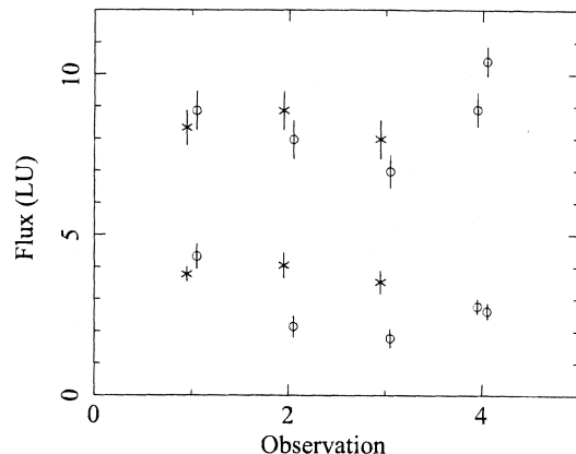
Fig. 1.— Fitted values for the O VII (upper grouping of points) and O VIII line fluxes (lower grouping of points). Data points with an X symbol are in the direction of the SEP and data points with a circle symbol are in the direction of the HDFN. The pairs of points at observations 1–3 are ObsIDs (0162160101, 0162160201), (0162160301, 0162160401), and (0162160501, 0162160601), respectively. The observation 4 data points are from two HDFN spectra (0111550201, 0111550401) from Snowden, Collier, & Kuntz (2004).
