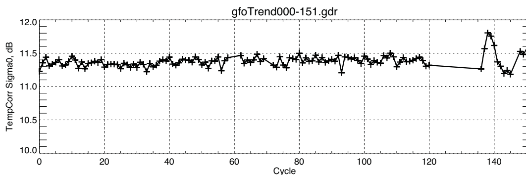
Figure 2-15 GFO Cycle-Averages Temperature Corrected Sigma0 in dB
