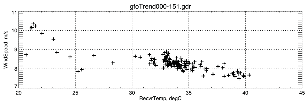
Figure 2-14 GFO Cycle-Averages Windspeed vs. Temperature
