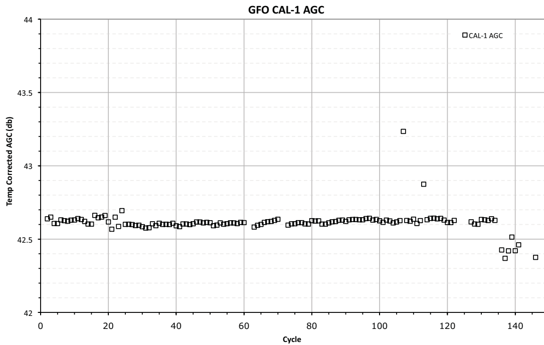
Figure 2-4 CAL-1 AGC for the First 152 GFO Cycles
