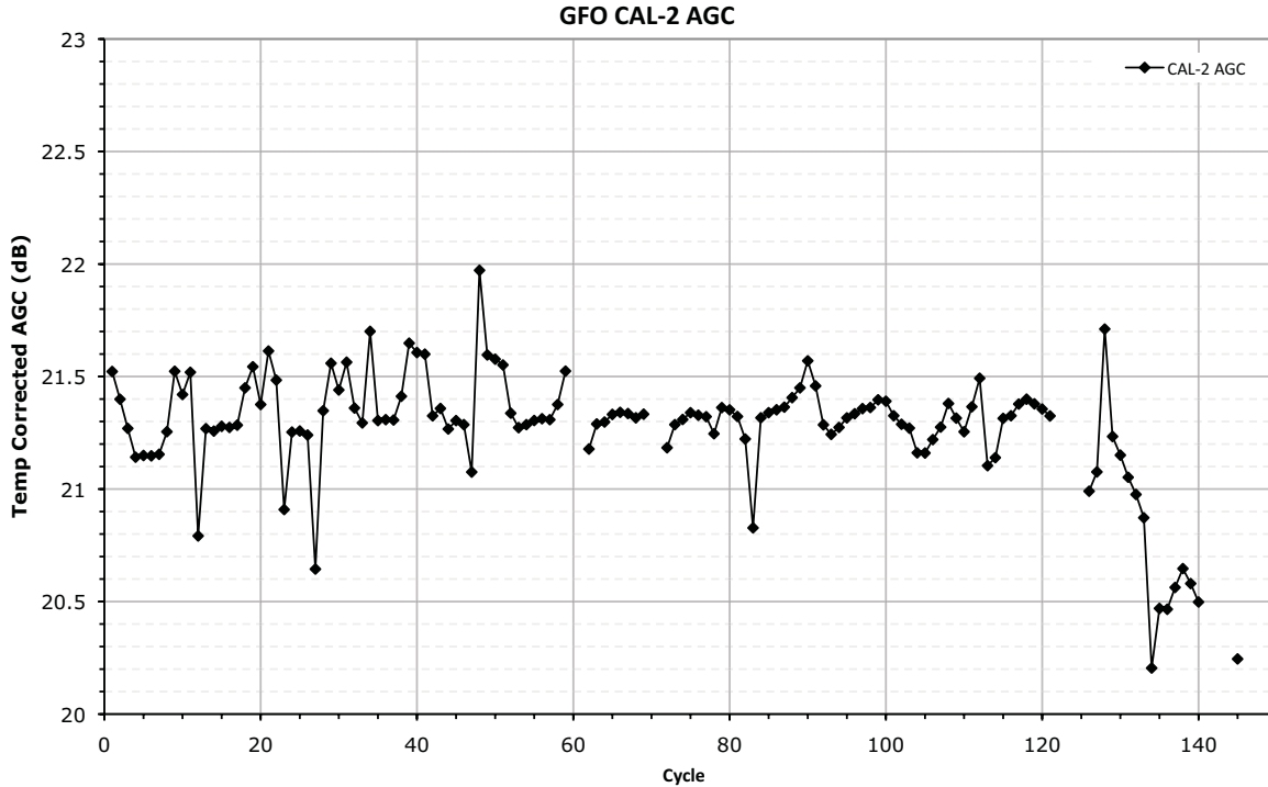
Figure 2-5 CAL-2 AGC for the First 152 GFO Cycles
