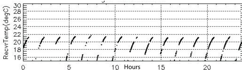
Figure 2-2 Receiver Temperature
