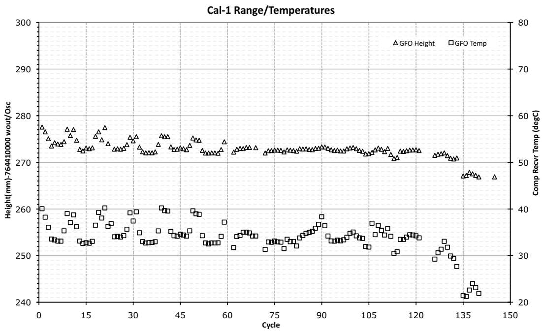
Figure 2-3 CAL-1 Range/Temperatures for the First 152 GFO Cycles
