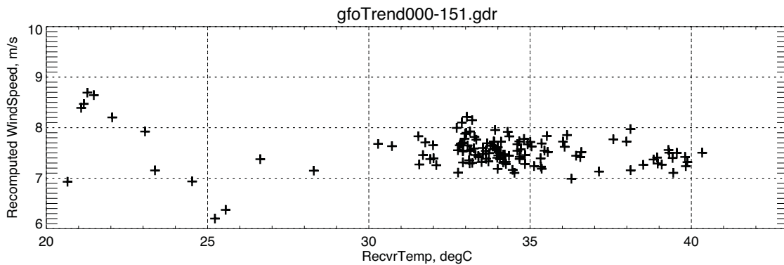
Figure 2-18 GFO Cycle-Averages Recomputed Windspeed vs. Temperature
