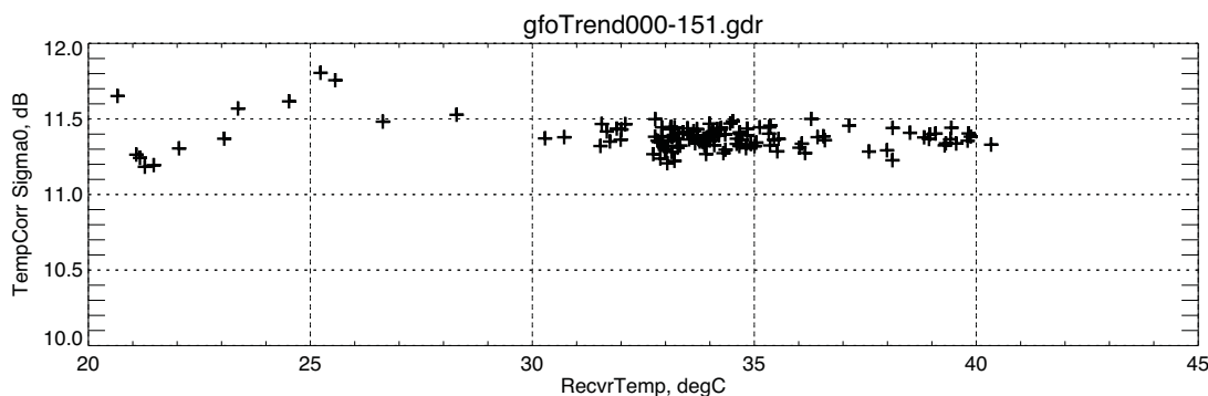
Figure 2-16 GFO Cycle-Averages Temperature Corrected Sigma0 vs. Temperature
