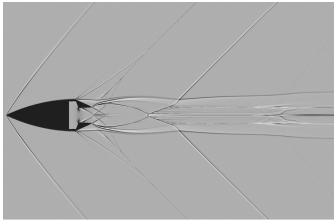
d) Nozzle pressure ratio of 25.2.
