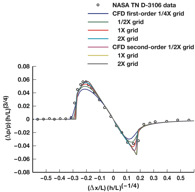
b) Pressure distribution at h/L = 10 .
