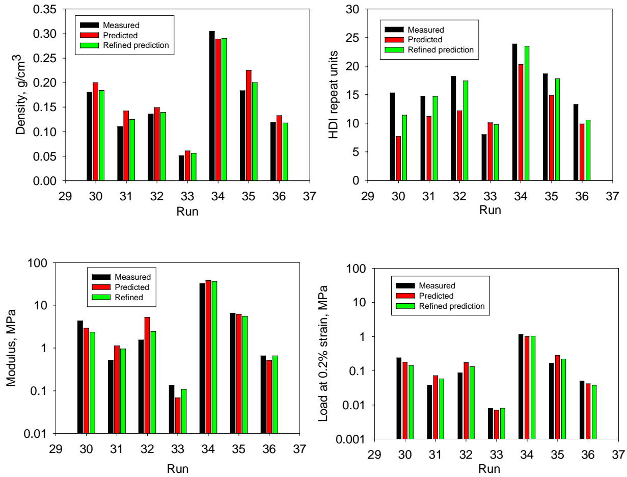
Figure 13. Select data from optimum runs compared to that predicted from the models.
