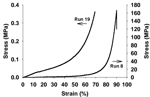
Figure 9. Stress-strain curves for selected runs showing range of strengths from different density samples. Arrows indicate correct axis for each plot.
