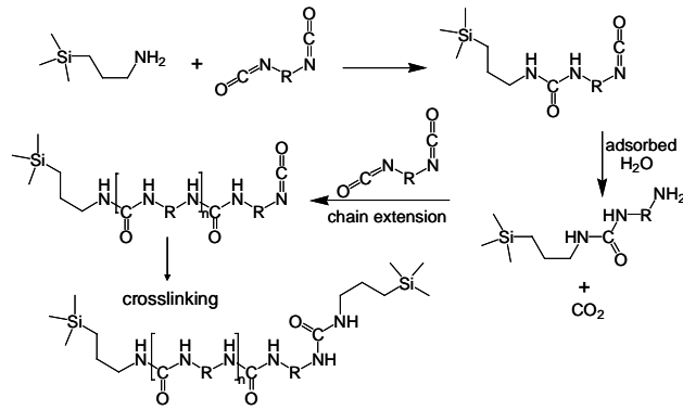
Scheme 1. Mechanism of cross-linking amine modified silica aerogels with di-isocyanate.
