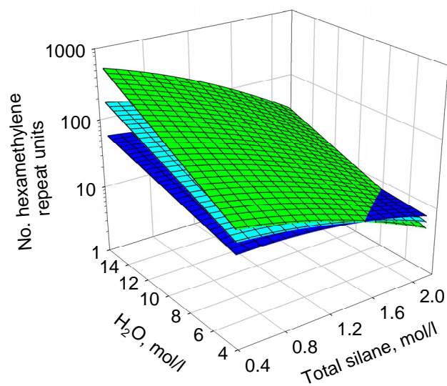
Figure 4. Empirically derived graphs showing number of repeat units as measured by end group analysis vs. total silane and water concentration where di-isocyanate concentration is a) 6.89 w/w % and b) 33.9 w/w % . (Green: no washes, cyan: 2 washes, blue: 4 washes.)
