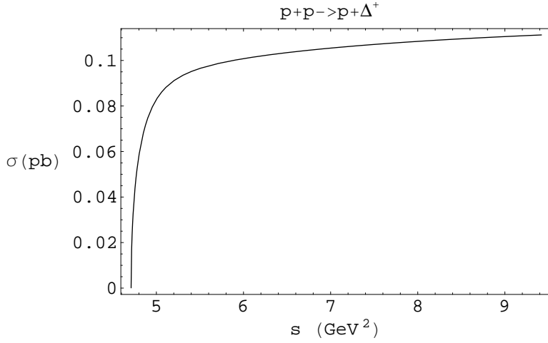
Figure 21: Total cross section (non-Rutherford).
