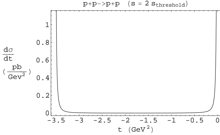
Figure 19: Invariant differential cross section (Rutherford).
