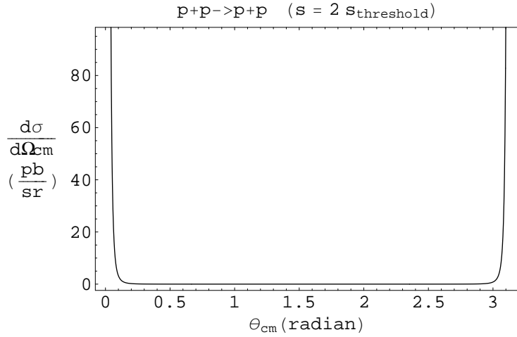
Figure 19: Invariant differential cross section (Rutherford).
