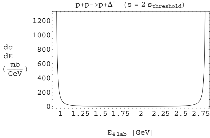
Figure 10: Differential cross section d\sigma/dE_{4l} .
