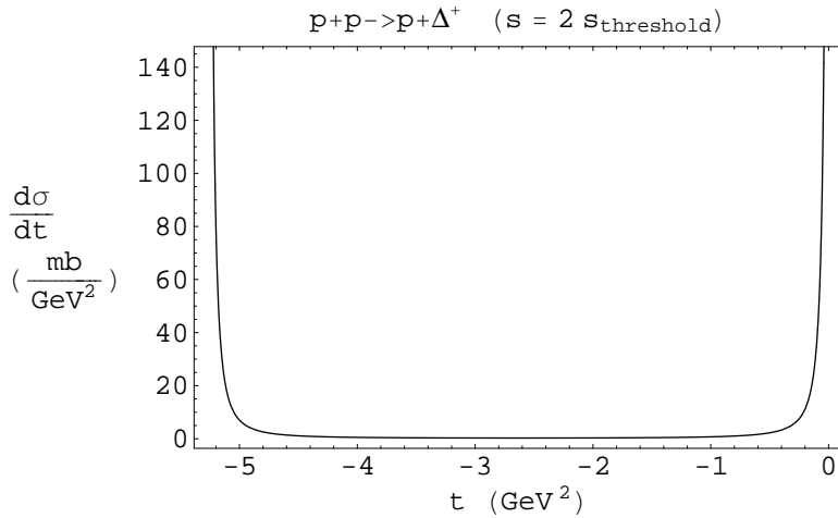
Figure 4: Differential cross section d\sigma/dt .
