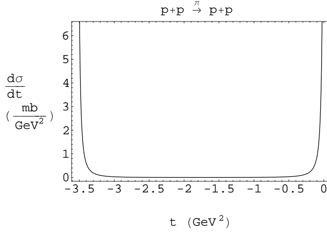
Figure 23: Invariant distribution for pp \rightarrow pp by pion exchange.
