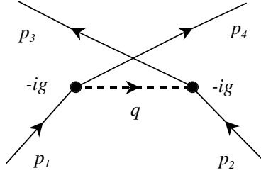
Figure 3: Exchange term of reaction 1 + 2 \rightarrow 3 + 4 .
