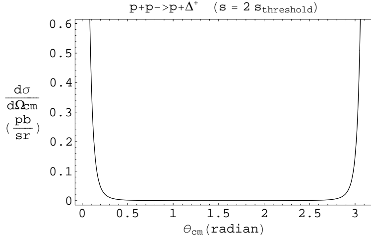
Figure 17: Invariant differential cross section (non-Rutherford).
