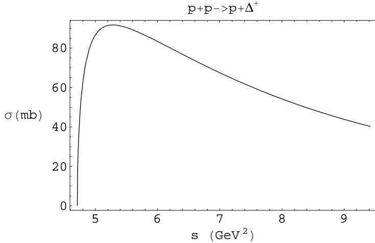
Figure 9: Total cross section \sigma .
