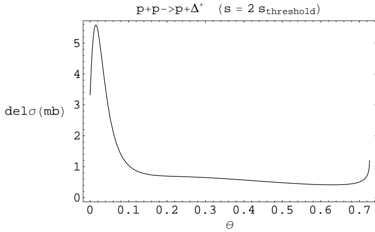
Figure 12: Differential cross section d\sigma/d\Omega_{3l} .
