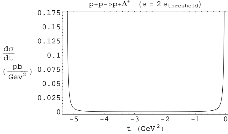
Figure 17: Invariant differential cross section (non-Rutherford).
