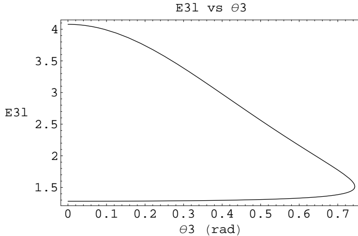
Figure 11: Energy E_{3l}(\theta_{3l}) . Upper and lower parts of the curve correspond to E_{3l} roots 1 and 2, respectively.
