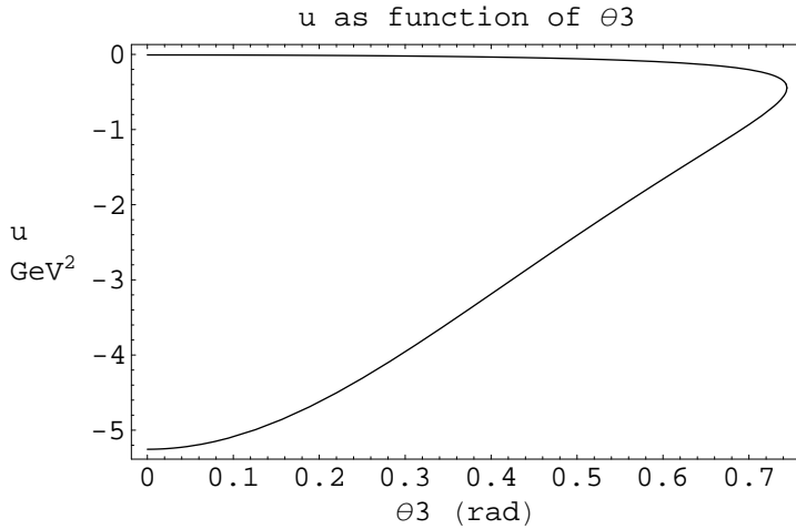
Figure 16: Mandelstam variable u as a function of \theta_{3l} .
