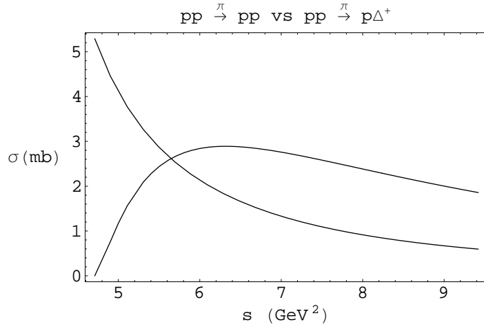
Figure 21: Total cross section (non-Rutherford).
