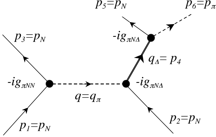
Figure 25: The Feynman diagram for the reaction NN \rightarrow N\Delta \rightarrow NN\pi . Note the labeling of the particle numbers. The initial state nucleons are labeled as particles 1 and 2. The final state nucleons are labeled as particles 3 and 5. The intermediate \Delta state is labeled as particle 4, and the final produced \pi is labeled as particle 6.
