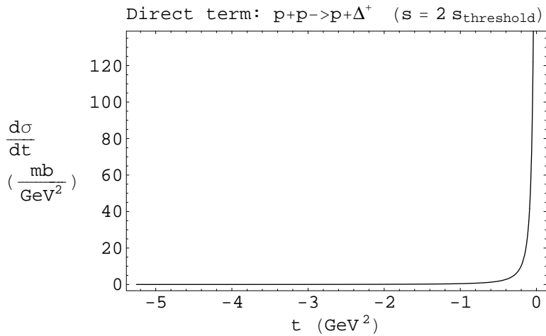
Figure 5: Differential cross section d\sigma/dt direct term.
