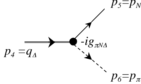
Figure 27: The Feynman diagram for the decay \Delta \rightarrow N\pi .
