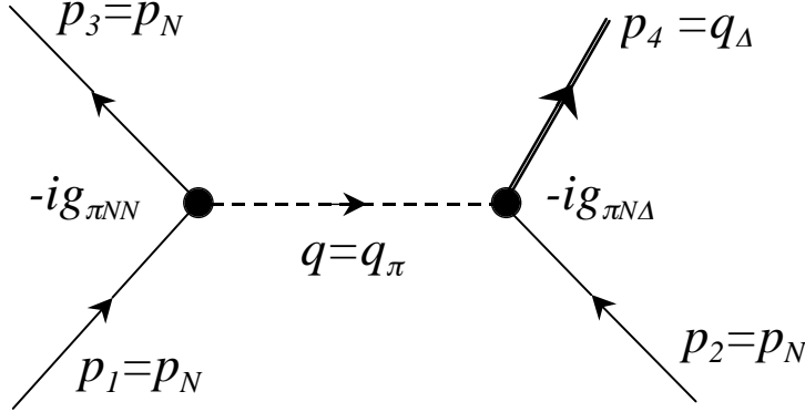
Figure 26: The Feynman diagram for the reaction NN \rightarrow N\Delta .
