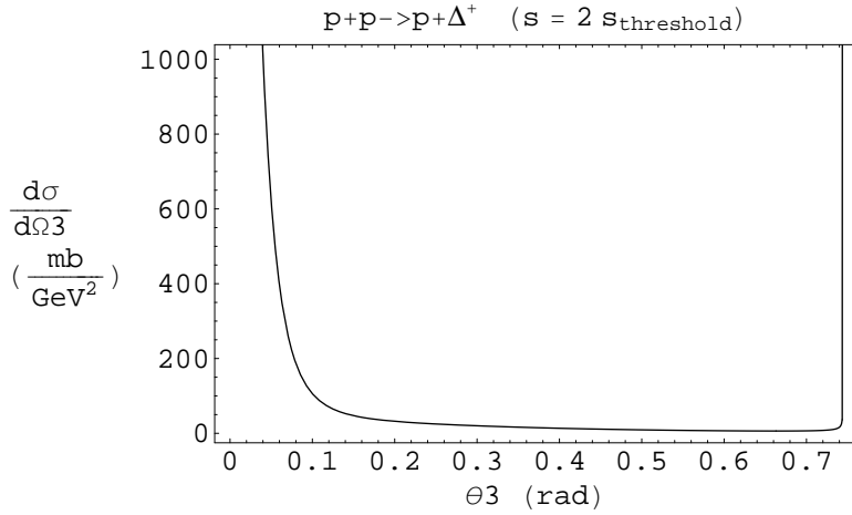
Figure 12: Differential cross section d\sigma/d\Omega_{3l} .
