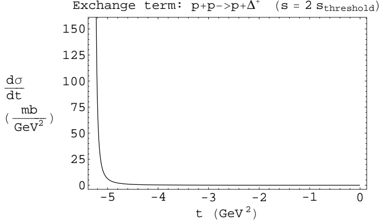
Figure 6: Differential cross section d\sigma/dt exchange term.
