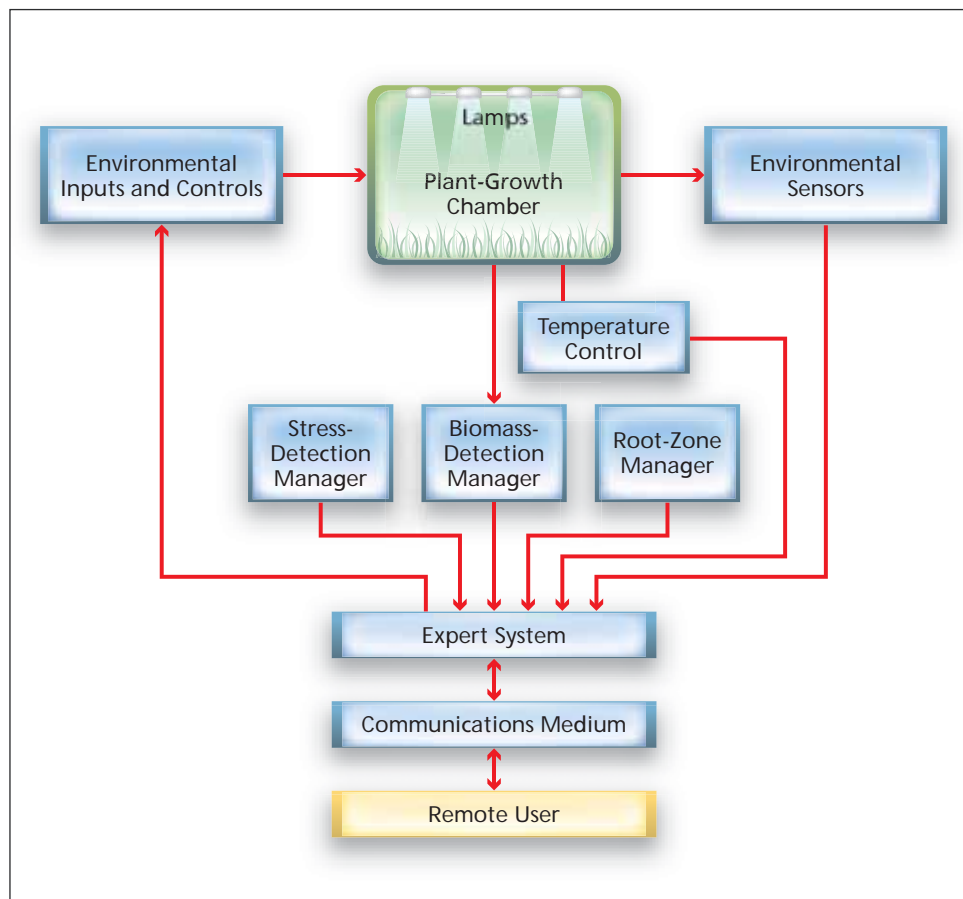
The Expert System adjusts inputs in response to image data and other sensory data, and controls the environment so that optimum plant-growth conditions are maintained.
