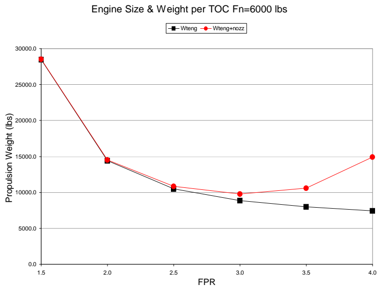
Figure 7: Engine weight with and without a noise suppressing nozzle
