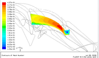
Mach in Ejector Slot region
