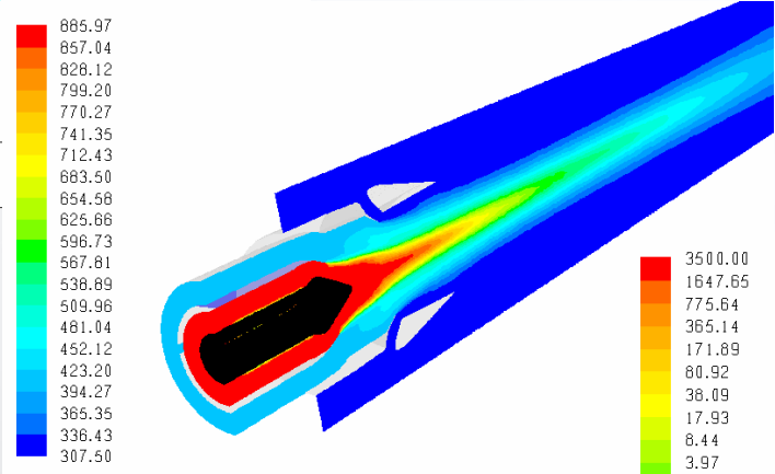
Total Temperatures
