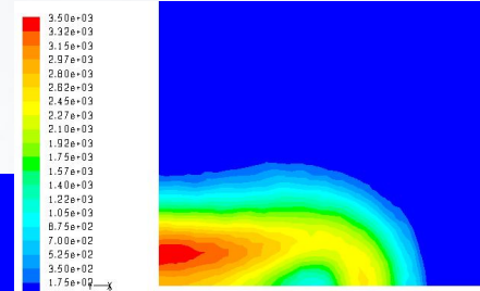
Contours of Turbulent Kinetic Energy (k) [m2/s2] Jul 26, 2008 FLUENT 6.3 [3d, pbns, ste]
