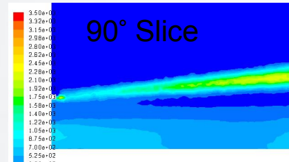
Contours of Turbulent Kinetic Energy (k) [m2/s2] Jul 26, 2008 FLUENT 6.3 [3d, pbns, ste]
