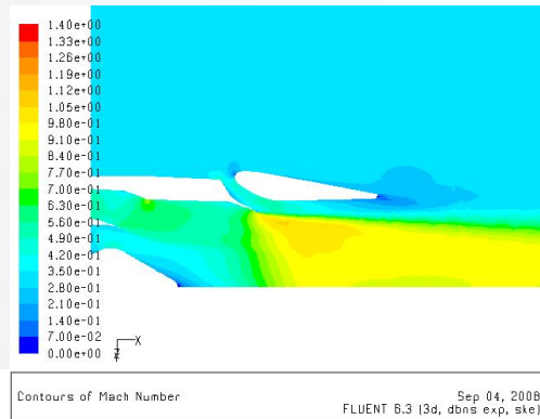
90° Plane Slice
