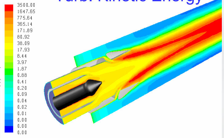
Sep 16, 2008 FLUENT 6.3 (3d, pbns, ske)
