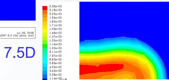
Contours of Turbulent Kinetic Energy (k) [m2/s2] Jul 26, 2008 FLUENT 6.3 [3d, pbns, ste]
