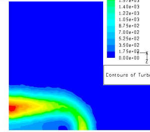
Contours of Turbulent Kinetic Energy (k) [m2/s2] Jul 26, 2008 FLUENT 6.3 [3d, pbns, ste]
