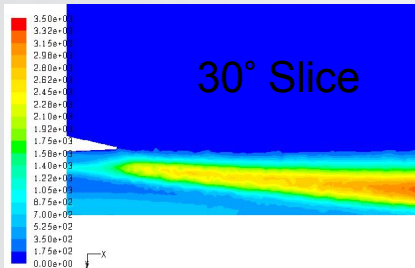
Contours of Turbulent Kinetic Energy (k) [m2/s2] Jul 26, 2008 FLUENT 6.3 [3d, pbns, ste]
