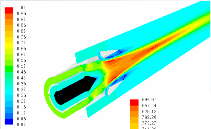
Mach Numbers
