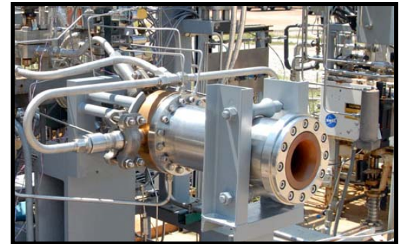
MSFC 6"-diameter combustion chamber
