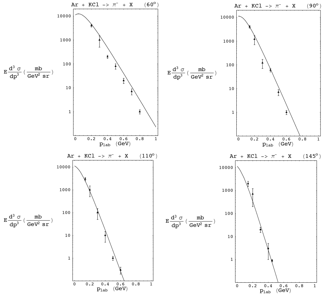
Figure 6: Same as figure 5, except different lab angles.
