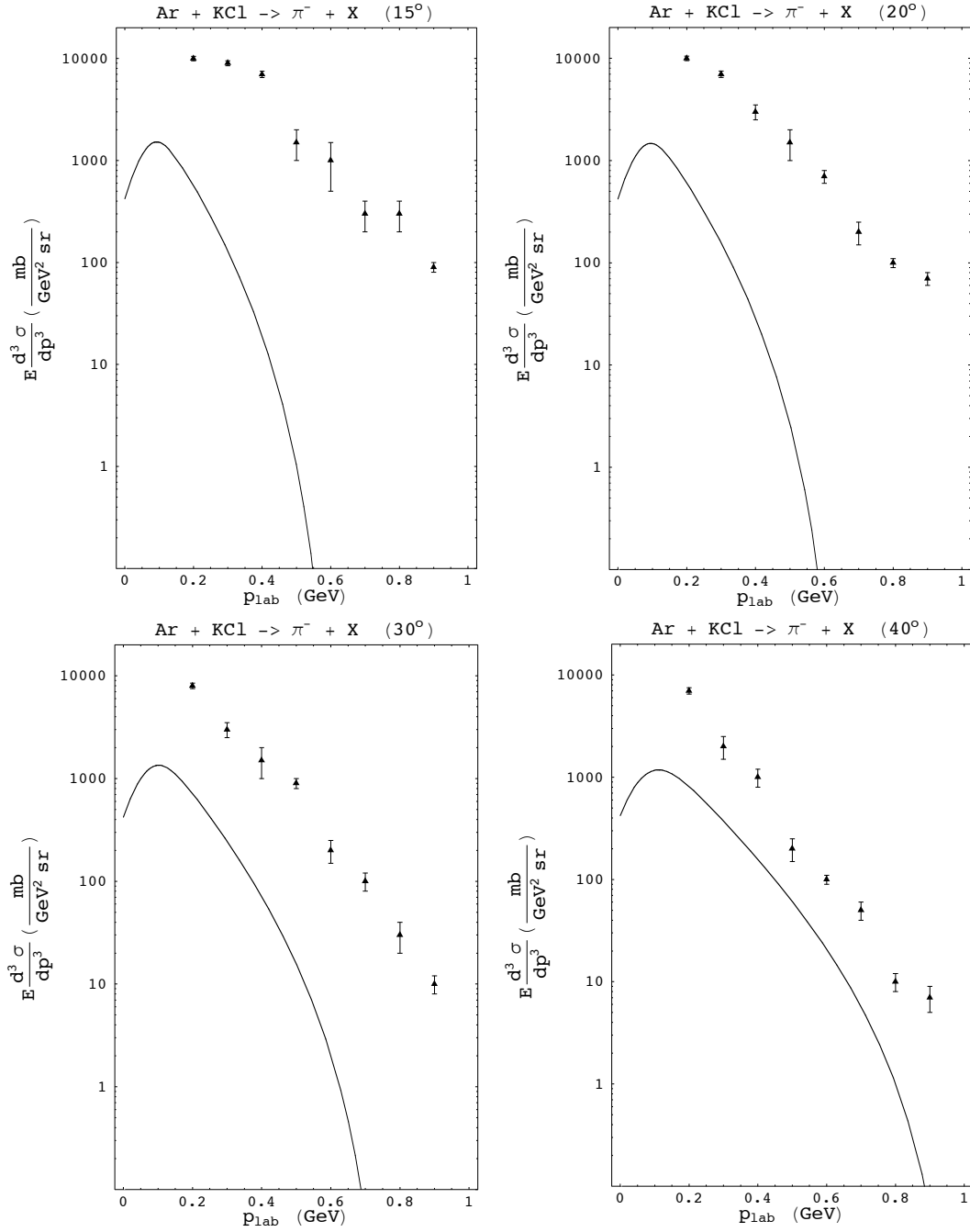
Figure 3: Badhwar parameterization [9] multiplied by (A_P A_T)^{2/3} fails to describe the data [10] at 800 A MeV. Lab angles are indicated. (Parameterizations of Alper [24], Carey [27], Ellis [26] and Mokhov [25] are of similar poor quality.)
