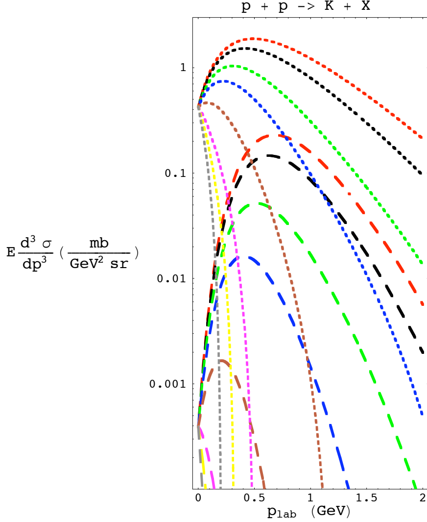
Figure 2: Kaon inclusive Lorentz invariant differential cross sections as a function of lab momentum and angle for proton - proton collisions with an incident proton kinetic energy of T_{\text{lab}} = 5 \text{ GeV} . The long dashed lines are K^- and the short dashed lines are K^+ . The lab angles from top to bottom are 15^\circ , 20^\circ , 30^\circ , 40^\circ , 60^\circ , 90^\circ , 110^\circ and 145^\circ . The curves have been generated using the Badhwar and Stephens parameterizations [9] and by transforming to the lab frame.
