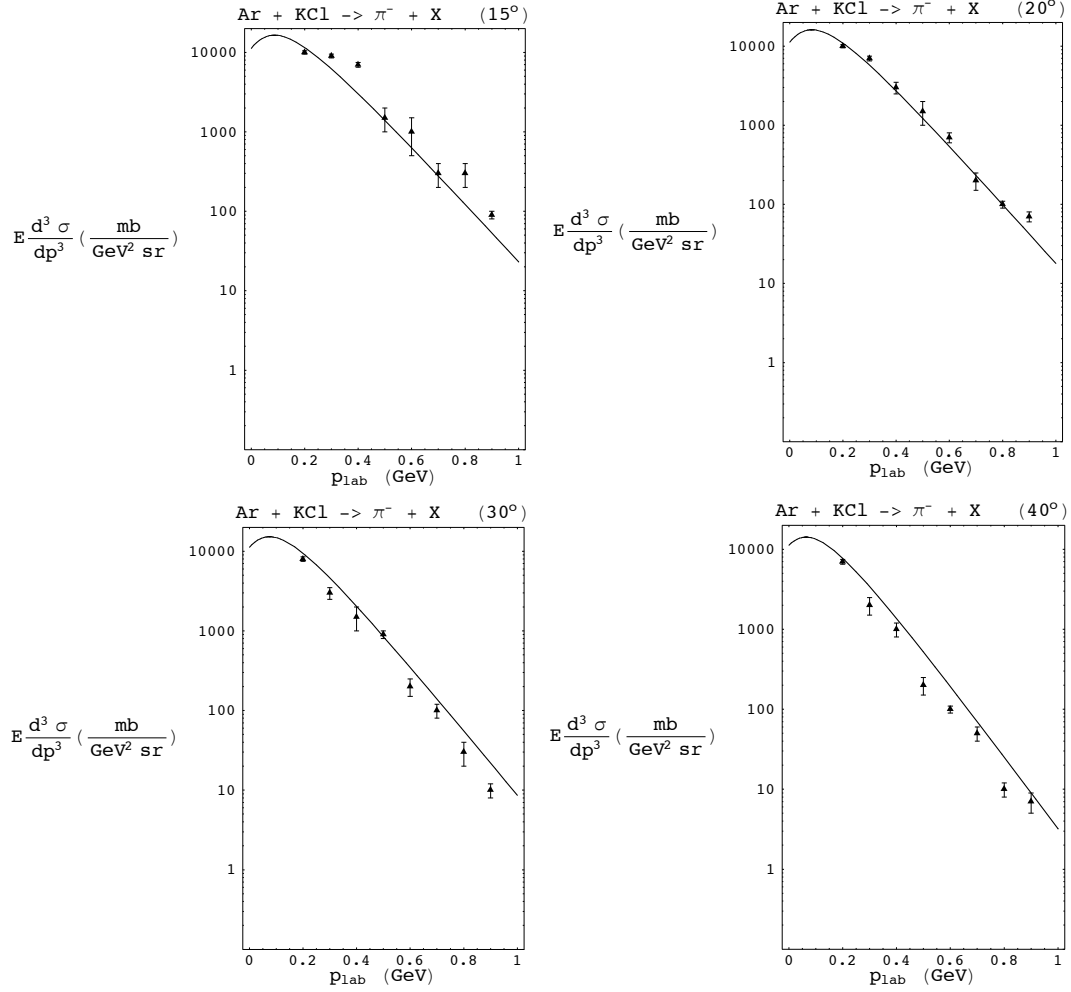
Figure 5: Thermal spectrum successfully describes data [10] at 800 A MeV. The overall normalization from equation (44) was fitted as N = 1.7 \times 10^4 \text{ mb/GeV}^2\text{sr} . The effective nuclear temperature, taken from reference [10], is E_0 = 66 \text{ MeV} . Lab angles are indicated.
