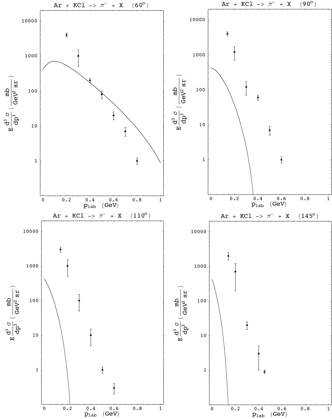
Figure 4: Same as figure 3, except different lab angles. (Parameterizations of Alper [24], Carey [27], Ellis [26] and Mokhov [25] are of similar poor quality.)
