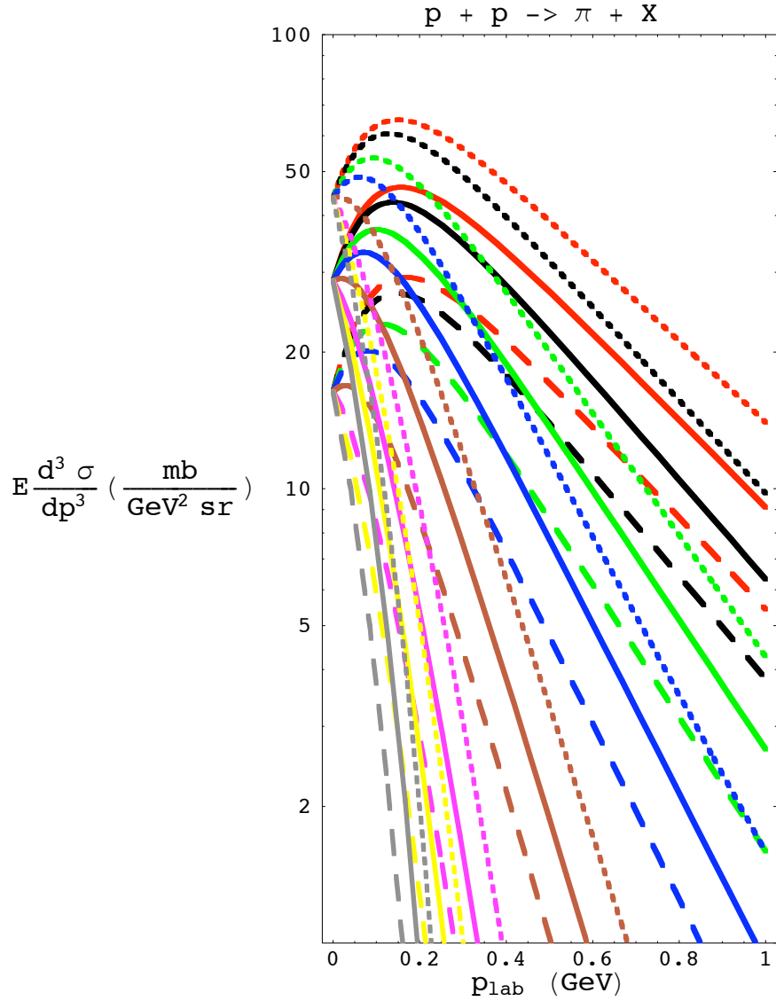
Figure 1: Pion inclusive Lorentz invariant differential cross sections as a function of lab momentum and angle for proton - proton collisions with an incident proton kinetic energy of T_{\text{lab}} = 5 \text{ GeV} . The solid lines are \pi^0 , the long dashed lines are \pi^- and the short dashed lines are \pi^+ . The lab angles from top to bottom are 15^\circ , 20^\circ , 30^\circ , 40^\circ , 60^\circ , 90^\circ , 110^\circ and 145^\circ . The curves have been generated using the Badhwar and Stephens parameterizations [9, 23] and by transforming to the lab frame.
