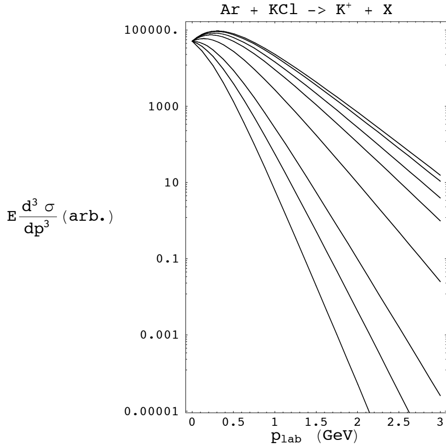
Figure 7: K^+ spectra at 2.1 A GeV, with the effective nuclear temperature, taken from references [17, 30], is E_0 = 142 MeV. Overall normalization is arbitrary. Lab angles from top to bottom are 15^\circ , 20^\circ , 30^\circ , 40^\circ , 60^\circ , 90^\circ , 110^\circ , 145^\circ .
