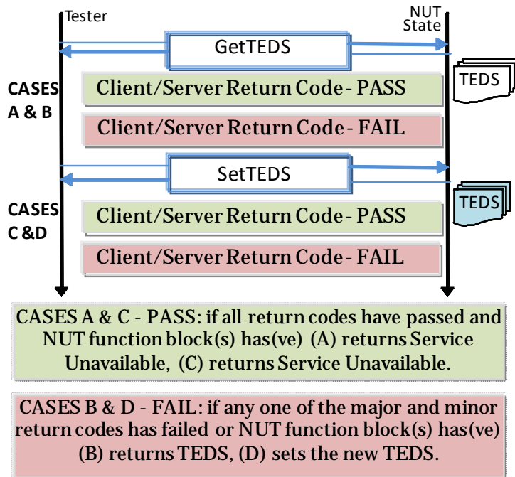
Figure 6. Before NUT is changed to active state (while in BL_INACTIVE state), GetTEDS and SetTEDS operations should return “Service Unavailable” in their return codes. When NUT is in BL_ACTIVE state the cases for FAIL and PASS would be reversed.
