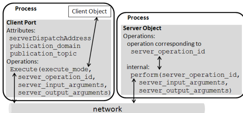
Figure 9. Client/Server communications using the attributes from Dot1 [8: p. 29 fig. 6].
