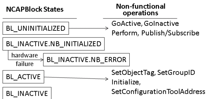
Figure 3. (a) NCAP block states and the corresponding non-functional operations. When NCAP block is active, addressing operations such as SetObjectTag is not operational to prevent conflicts.
