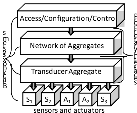
Figure 1. Current proprietary approach is based on complete solutions all the way up to the user access with no room for interoperability between components from different manufacturers.
