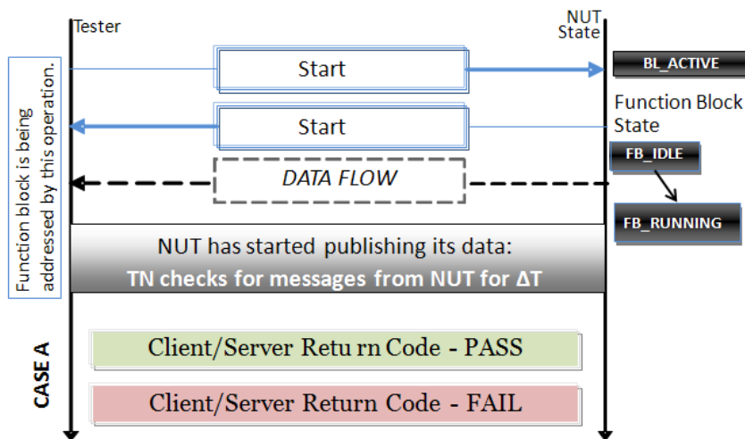
Figure 7. (a) Start operation will activate the publication of data in a multicast fashion when the update method is set to “Publish.”
