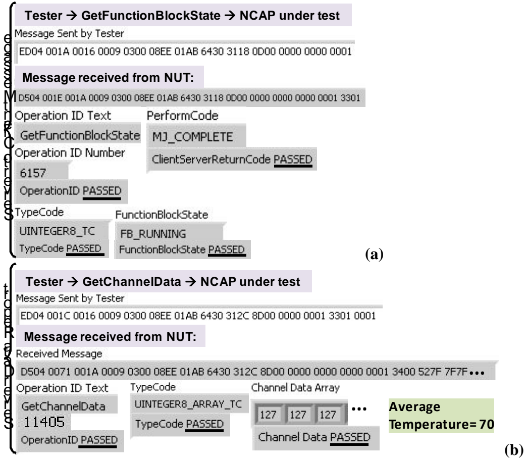
Figure 12. (a) Function block state is returned as FB_RUNNING which is suitable for sensor readings and reporting. (b) Channel data has been posted for temperature sensor.
