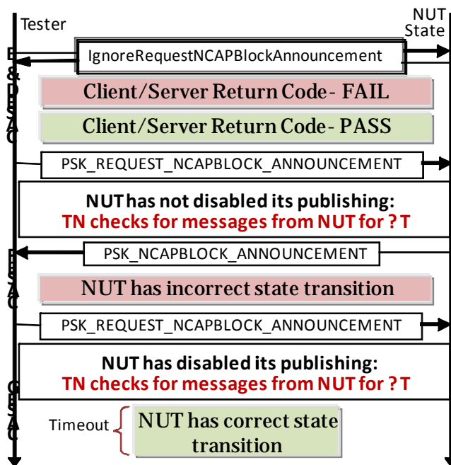
(b) NUT states are tested using state enabler and disabler operations.
