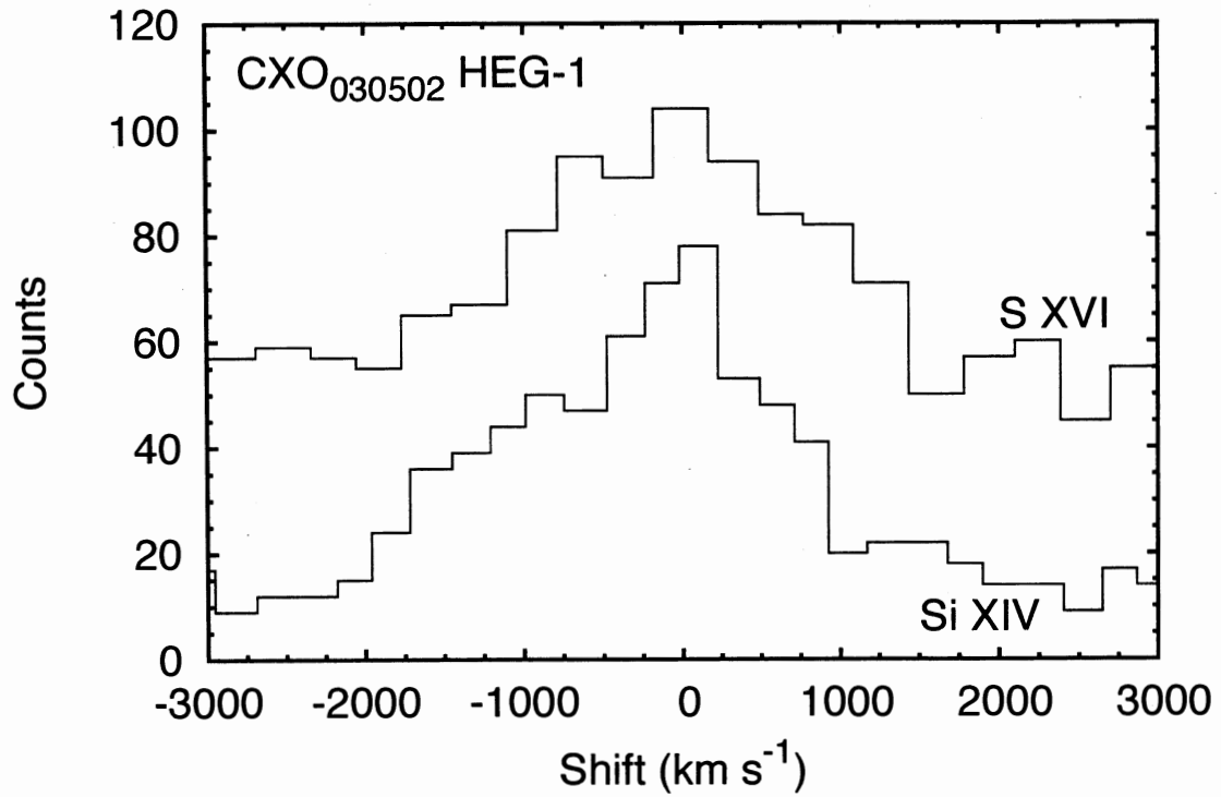
Fig. 13.— Comparison of the HEG -1 profiles of S xvi and Si xiv Ly \alpha from CXO 030502 . For clarity, the profiles have been binned by a factor of two, and the S xvi profile has been shifted upward by 30 counts.
