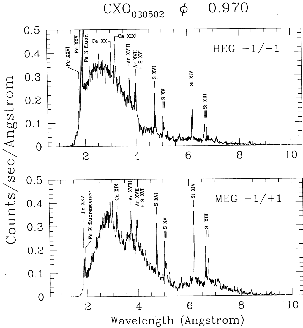
Fig. 3.— As Figure 1, but for CXO 030502 .
