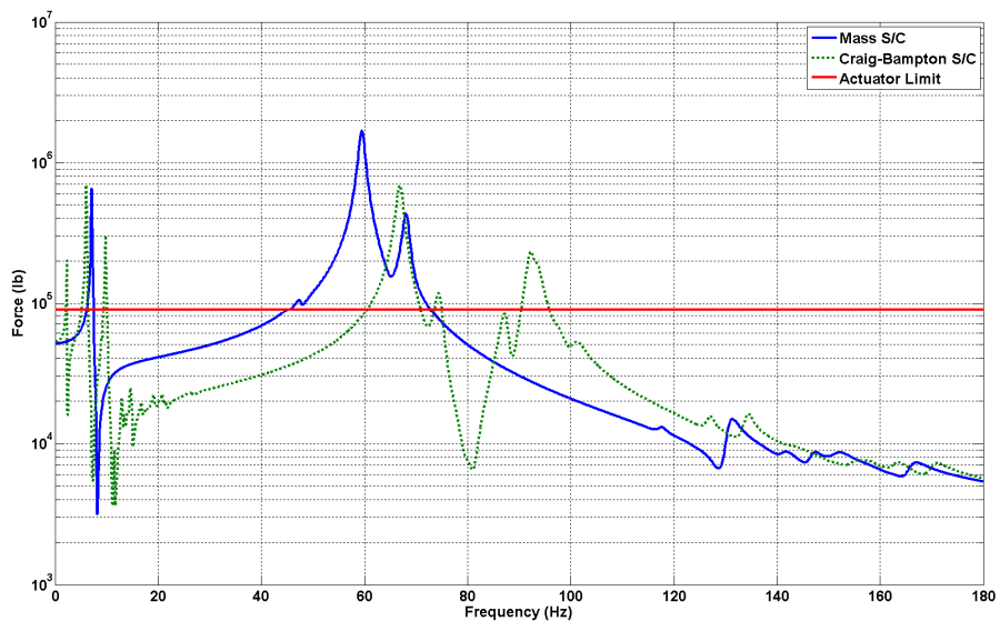
Figure 10.—Required average actuator force to produce 1 g lateral (X-axis) drive at actuator ends for lumped mass and Craig-Bampton models.
