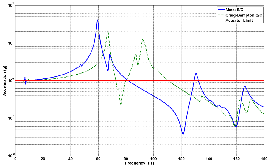
Figure 9.—Average response at spacecraft base due to 1 g lateral (X-axis) drive for lumped mass and Craig-Bampton models.
