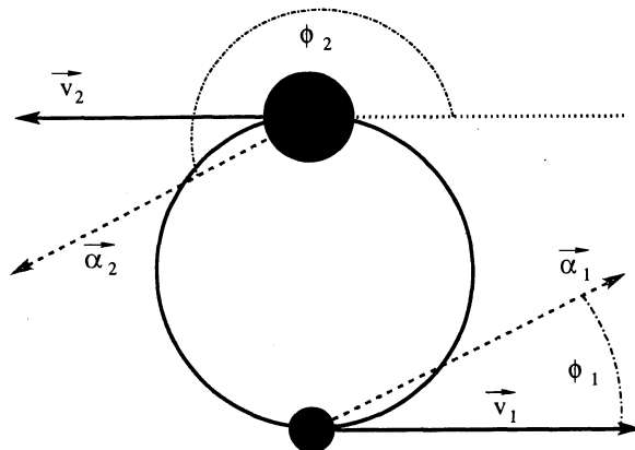
FIG. 1.— Configuration of black holes for all new simulations. The two holes' spins \vec{\alpha}_{1,2} lie initially in the orbital plane, at angles \phi_1 and \phi_2 to \vec{v}_1 , the smaller hole's initial velocity.
